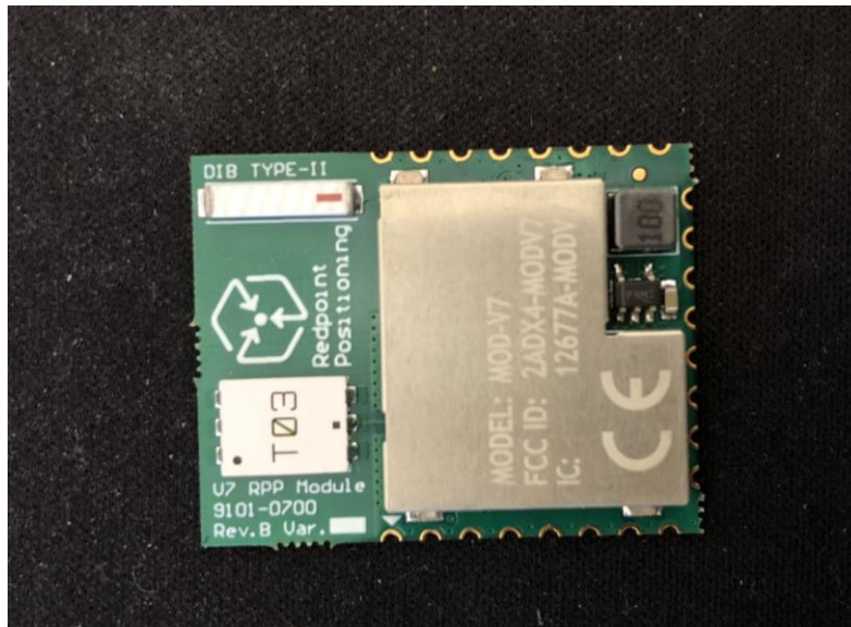
Figure 1. Top View
