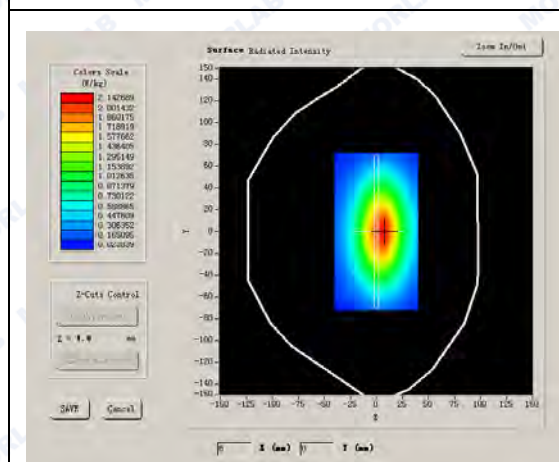
SURFACE SAR
