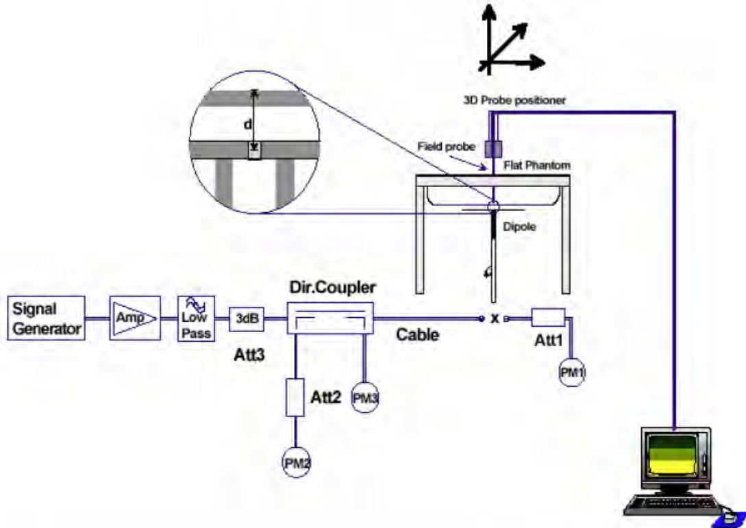
Picture 10. System Check Set-up
