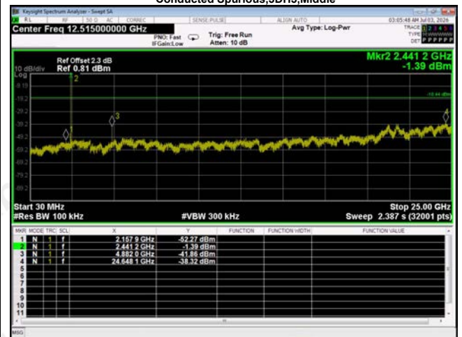
Conducted Spurious,3DH5,Middle
