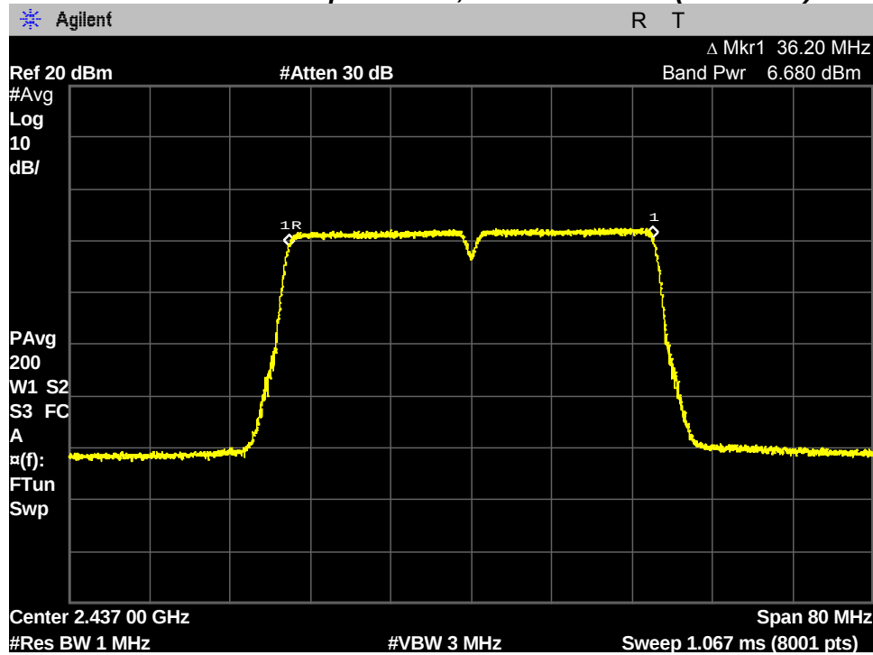
Maximum Conducted Output Power, Middle Channel (2437 MHz)
