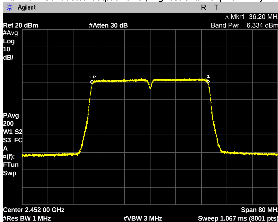
Maximum Conducted Output Power, Highest Channel (2452 MHz)
