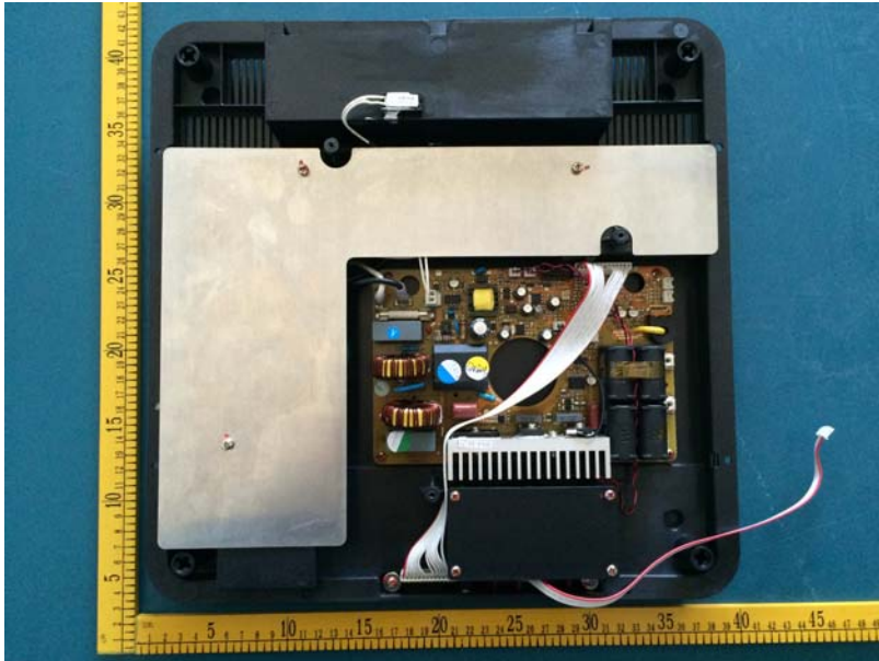
Photo 11 Internal of EUT
