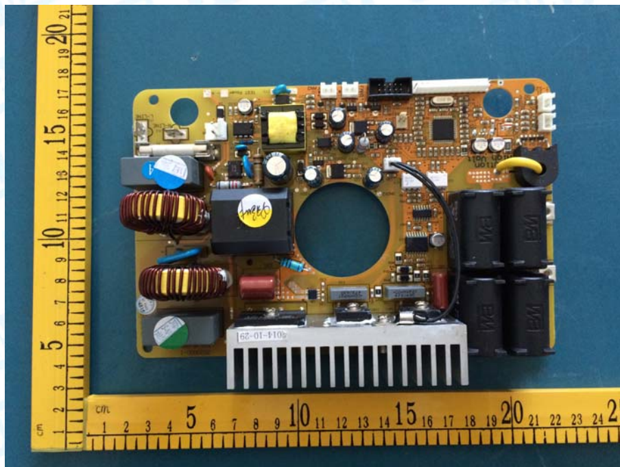
Photo 13 Appearance of Main Board
