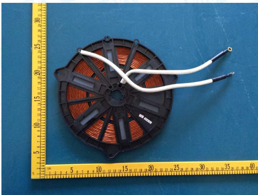
Photo 10 Appearance of Coil
