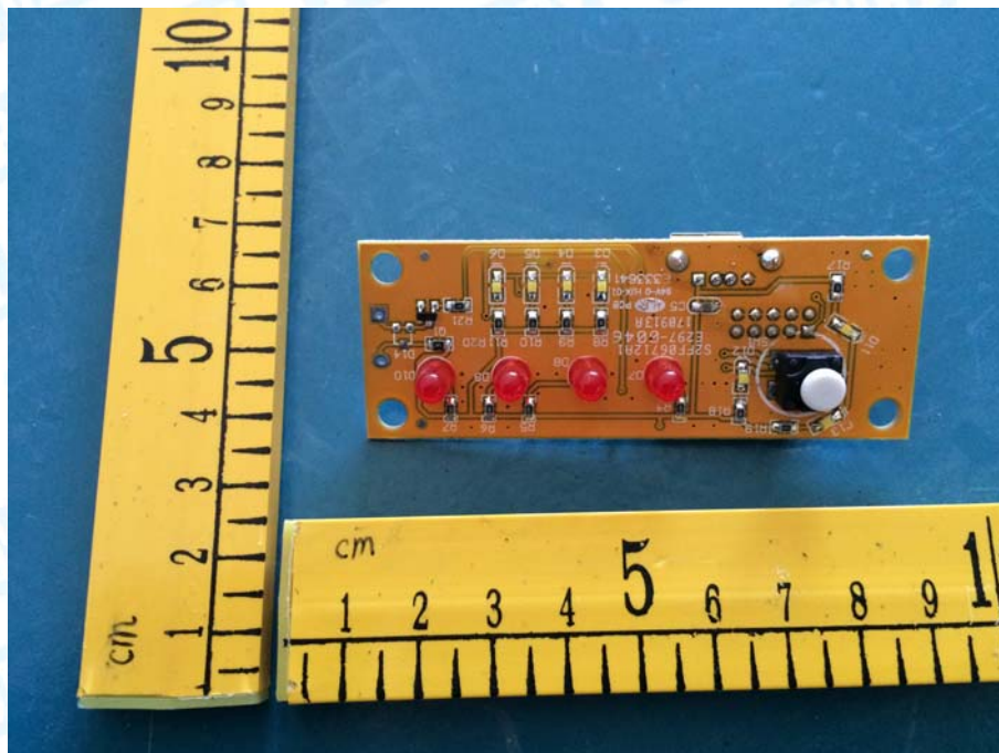
Photo 23 Appearance of Control Box Display Board
