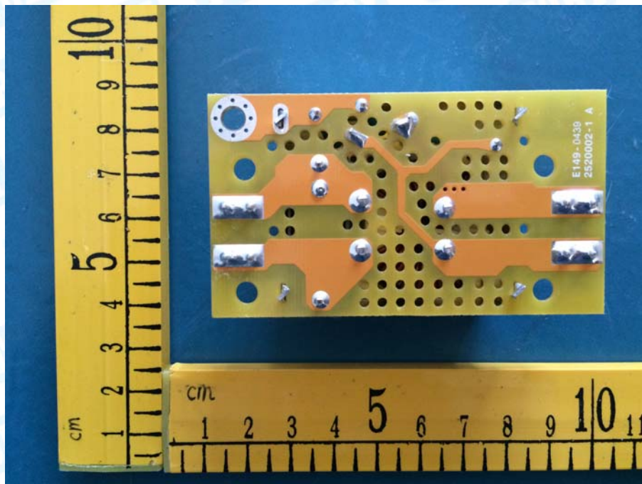
Photo 17 Appearance of EMI Board
