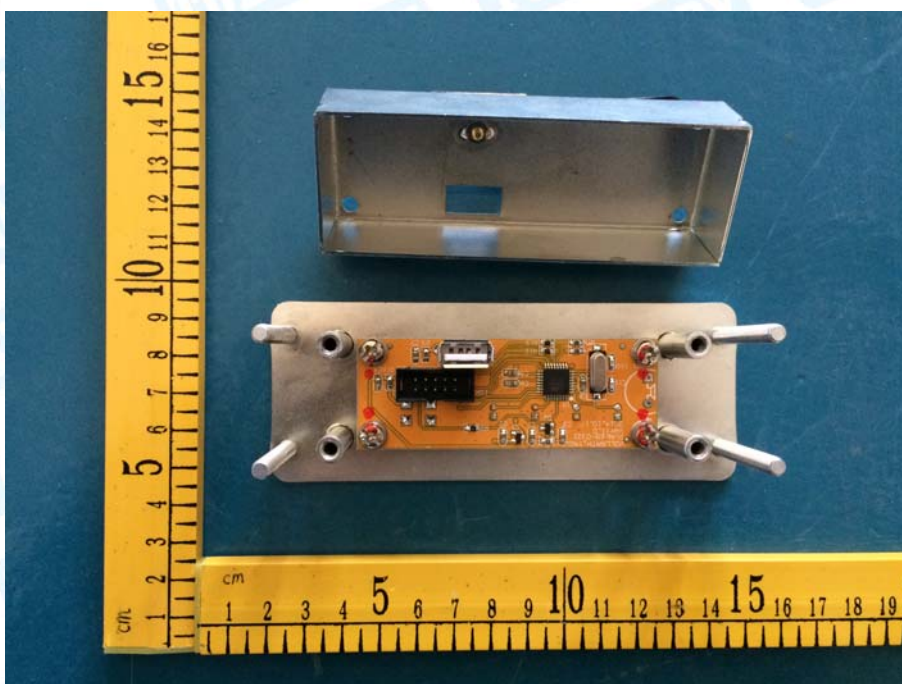
Photo 22 Internal of Control Box Display Board
