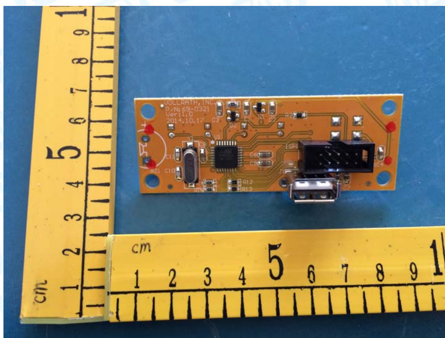
Photo 24 Appearance of Control Box Display Board
