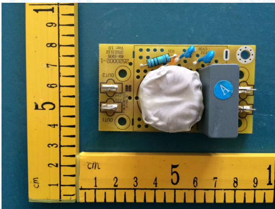
Photo 16 Appearance of EMI Board
