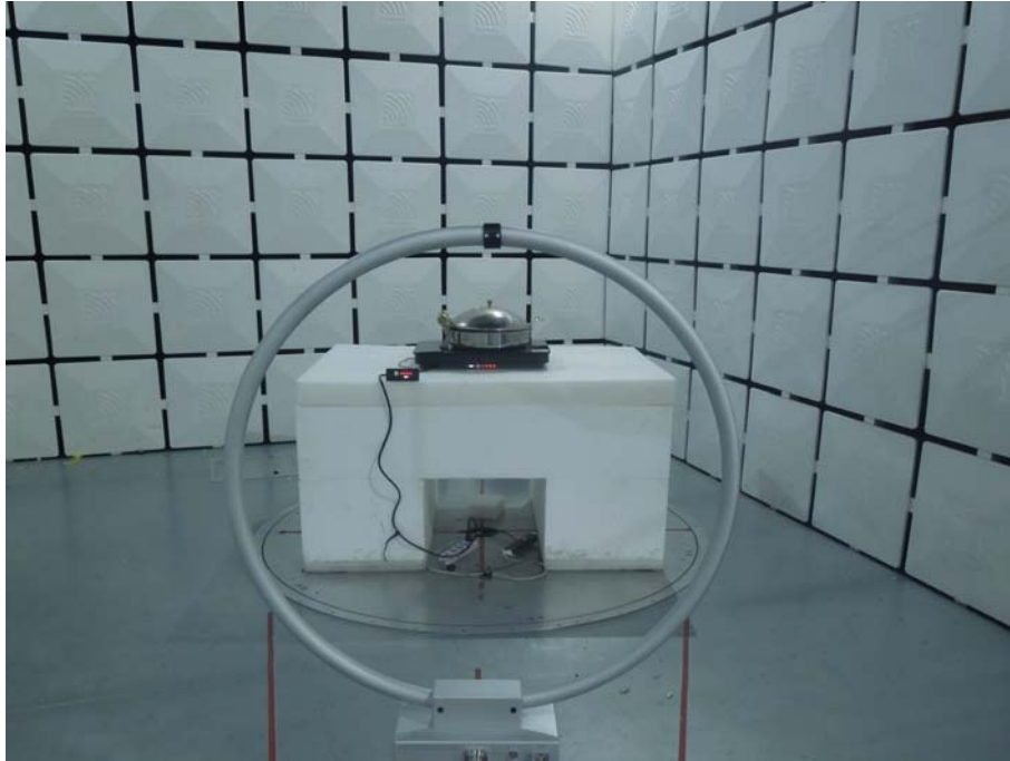
Photo of Setup for Radiated Emission (Three Unit)
