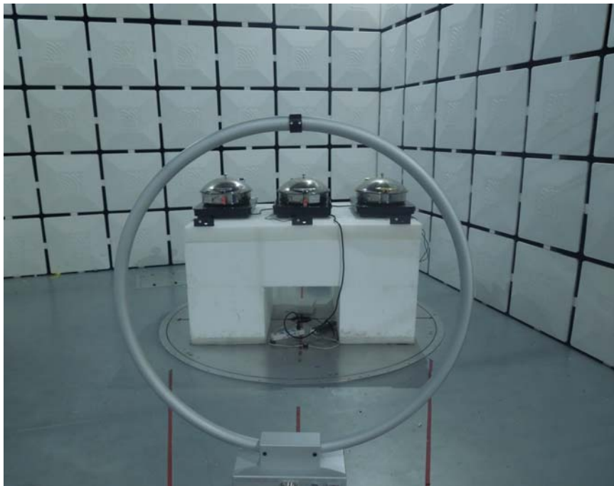
Photo of Setup for Radiated Emission (Three Unit)
