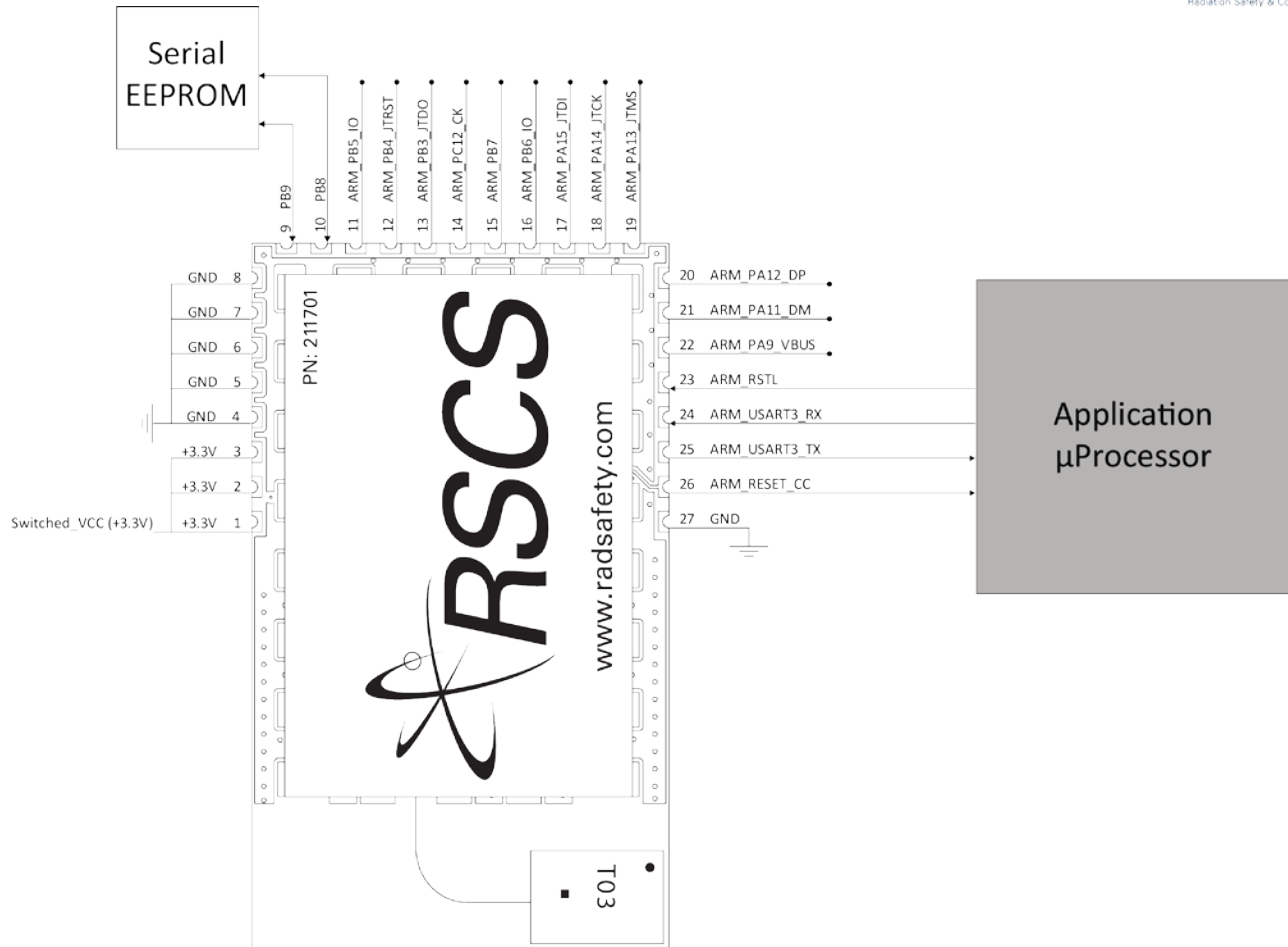
Figure 3 Example Application Circuit
