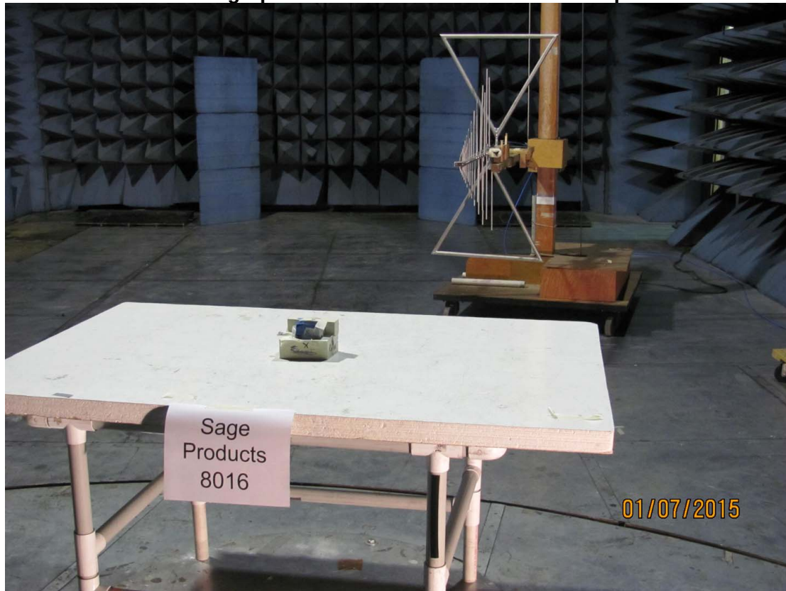
Photograph of Radiated Emissions Test Setup
