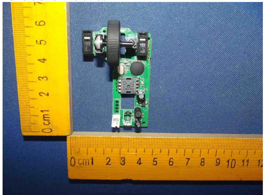
Figure 8 PCB of the EUT-Front View
