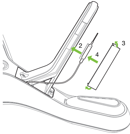
Figure 5.1.3: Leg Replacement Process 3
