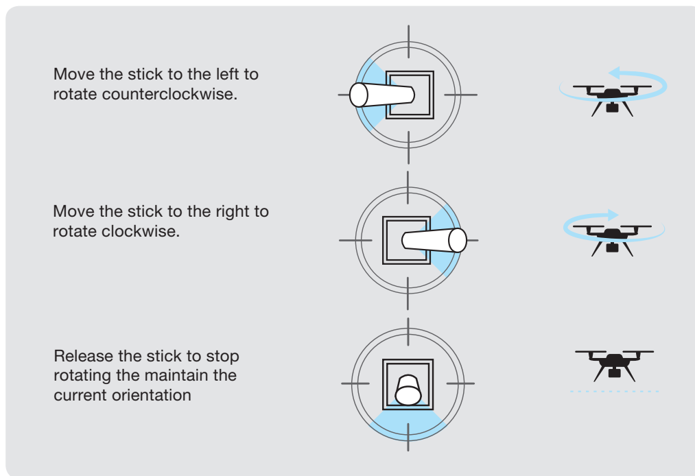
Figure 4.5.3: Yaw Joystick Behavior
