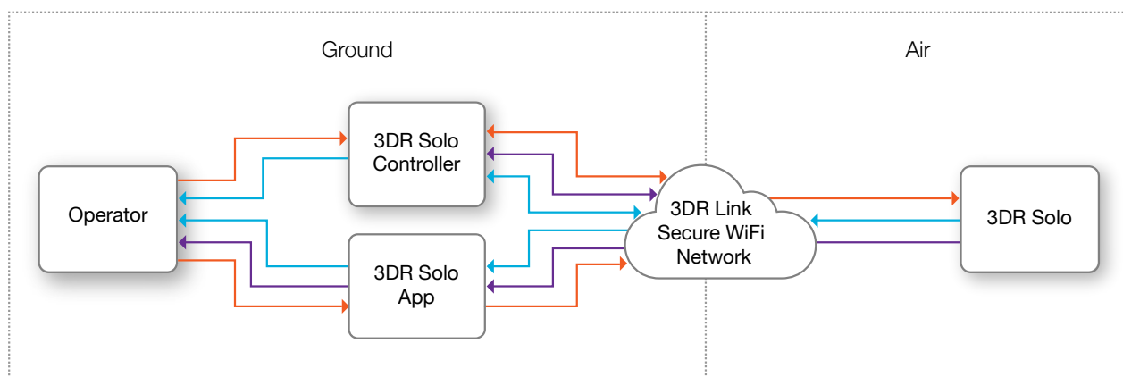
Figure 1.1.1: Solo System Context Diagram
