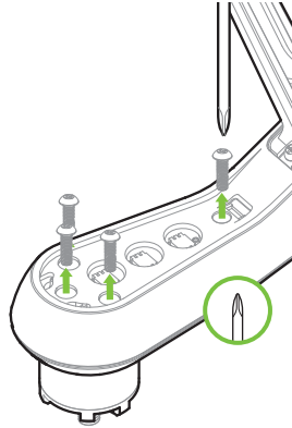
Figure 5.2.2: Motor Pod Replacement Process 2
