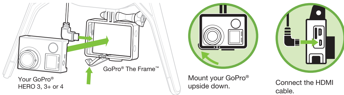
Figure 2.5.1: Attach Camera
