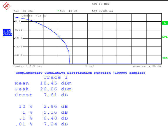
16QAM Low channel-25 RB offset 12
