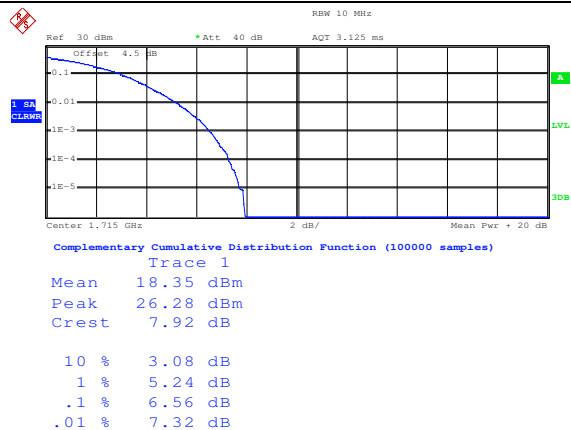
16QAM Low channel-25 RB offset 25
