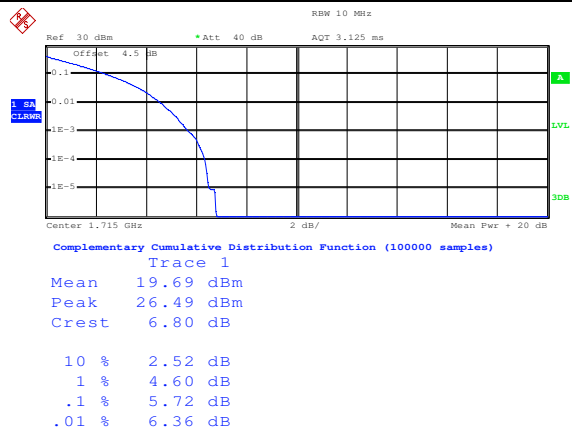
QPSK Low channel-25 RB offset 12
