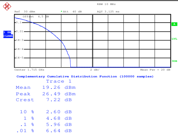
QPSK Low channel-25 RB offset 25
