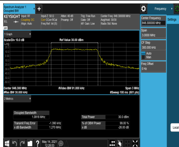
Band5-1.4MHz-16QAM-20643-6RB#0
