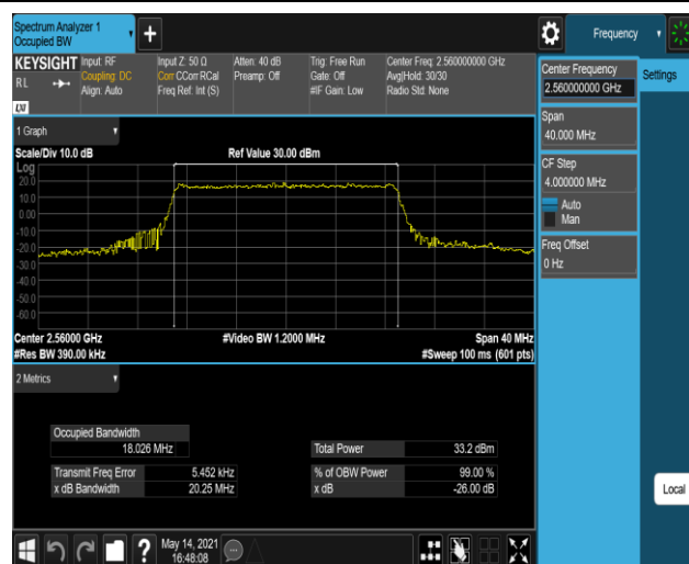
Band7-20MHz-16QAM-21350-100RB#0
