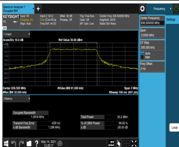
Band5-1.4MHz-16QAM-20525-6RB#0
