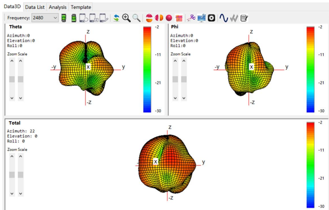
8. Antenna Pattern (2.0mm*1.2mm):
