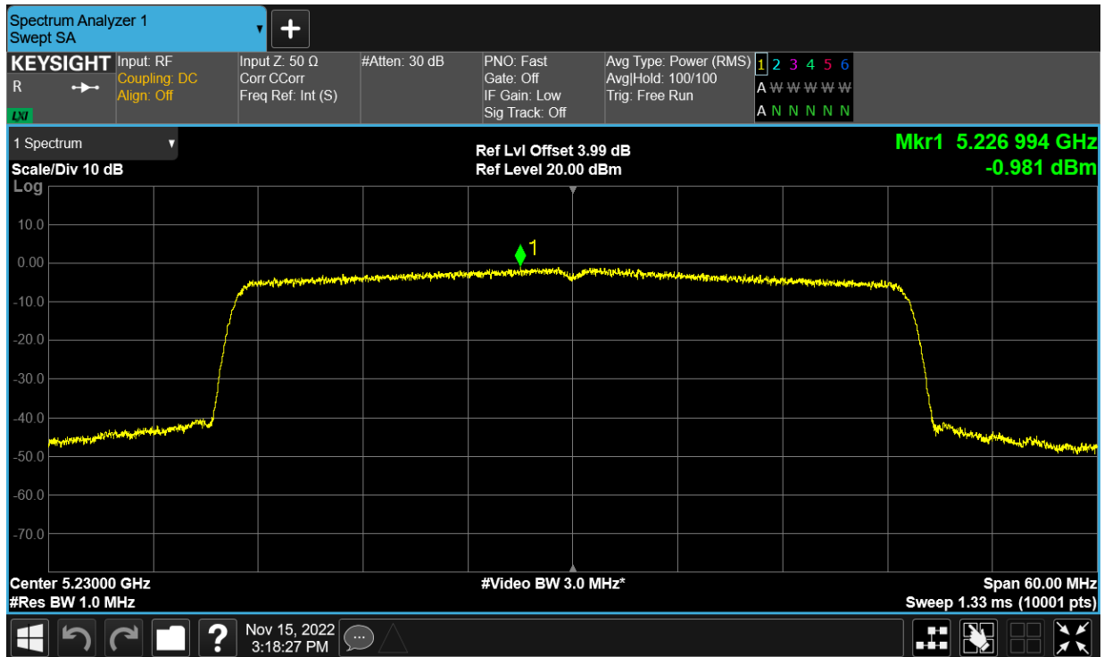
PSD NVNT ax40 5230MHz Ant24
