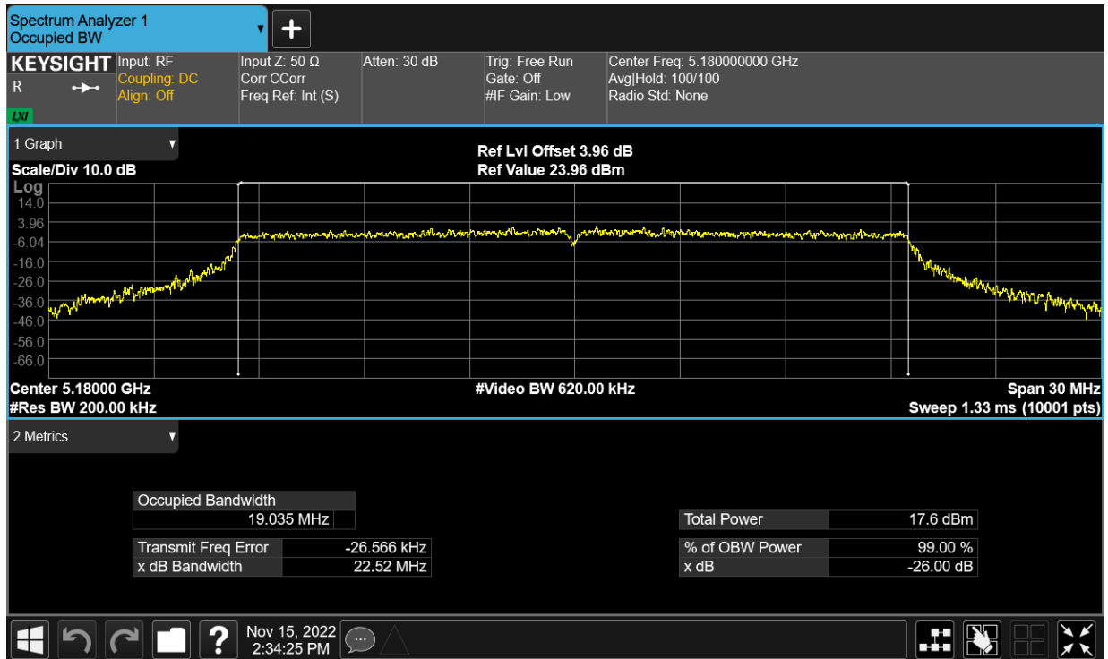
OBW NVNT ax20 5180MHz Ant24
