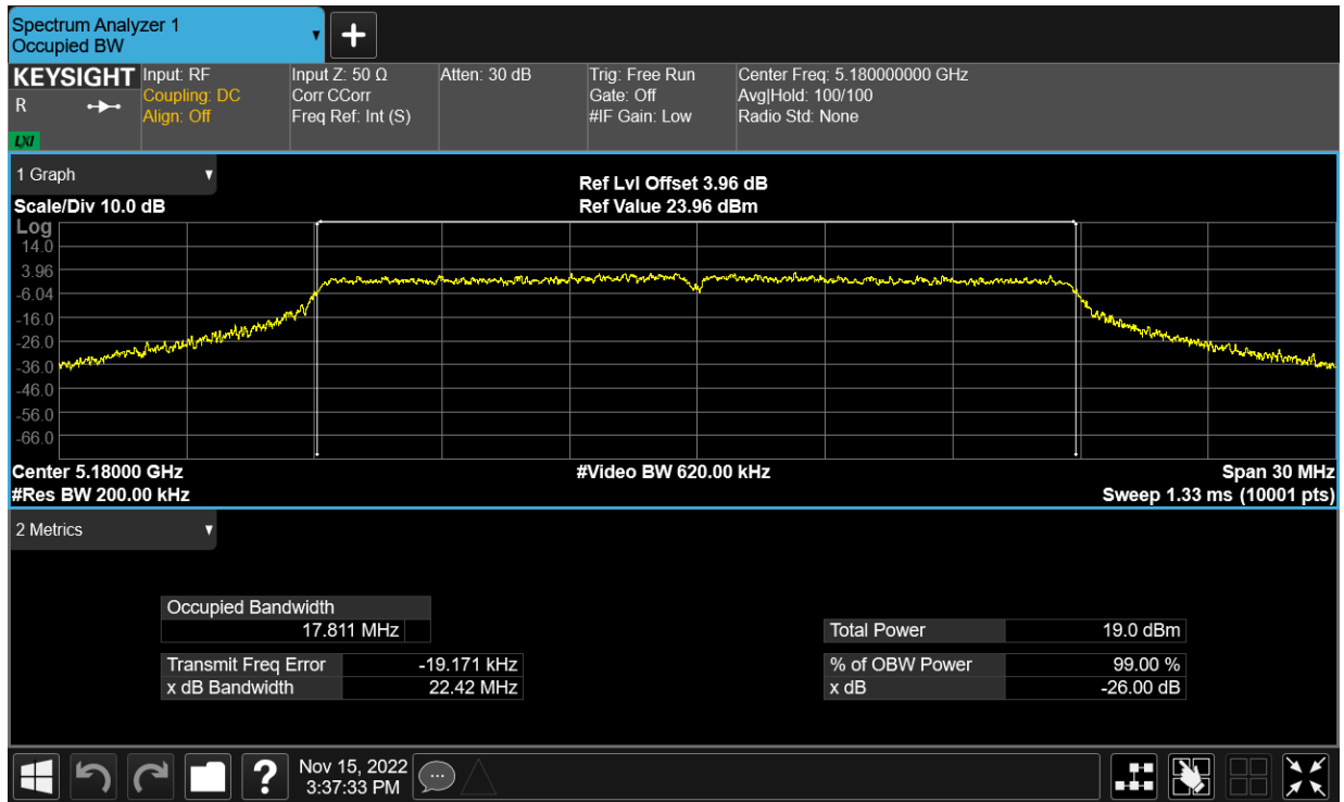
OBW NVNT n20 5180MHz Ant24
