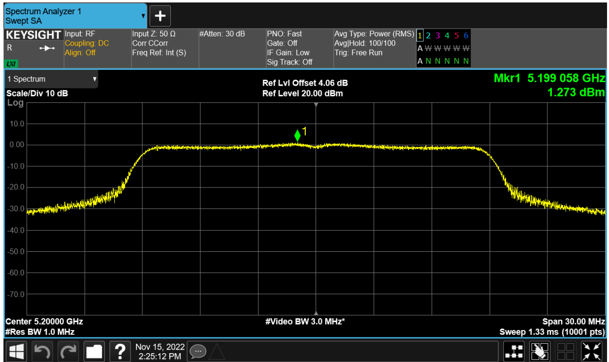
PSD NVNT ac20 5200MHz Ant24
