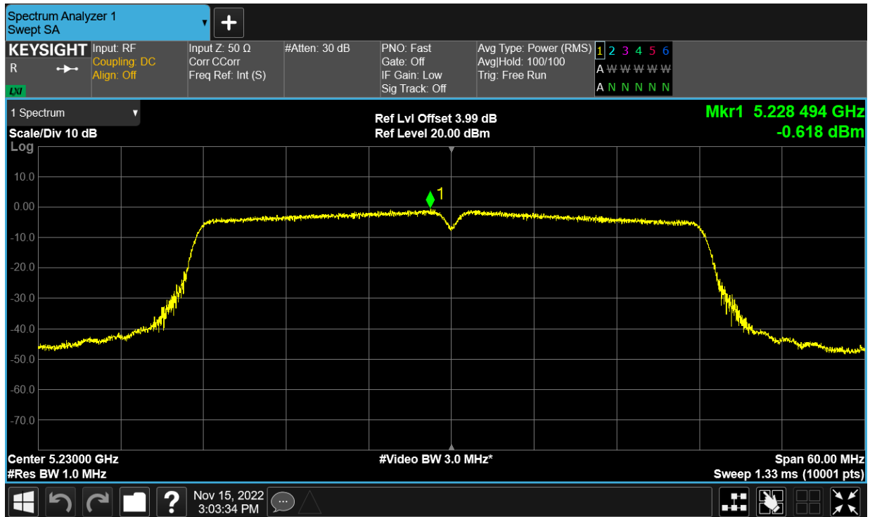
PSD NVNT ac40 5230MHz Ant24
