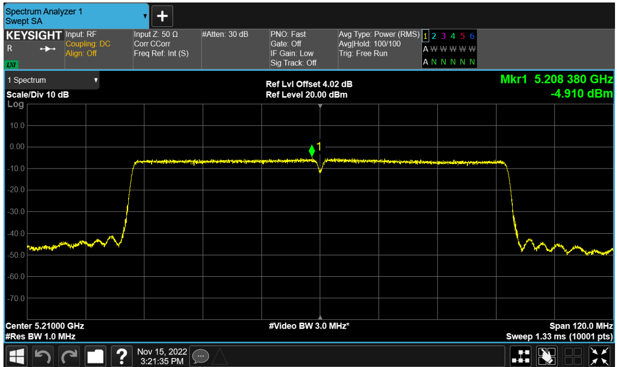
PSD NVNT ac80 5210MHz Ant24
