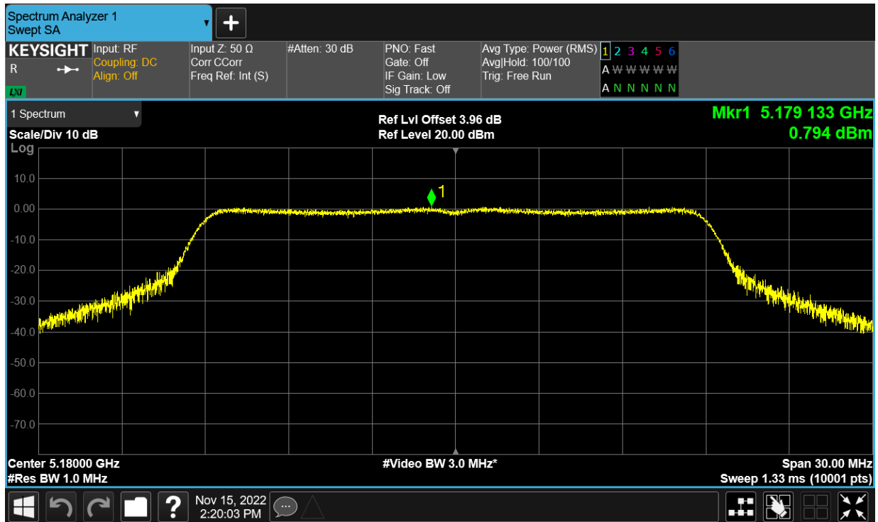
PSD NVNT ac20 5180MHz Ant24
