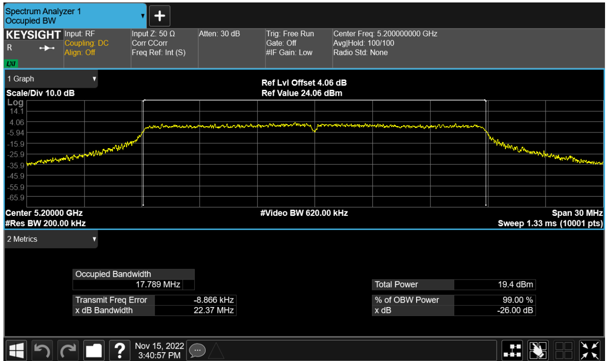
OBW NVNT n20 5200MHz Ant24
