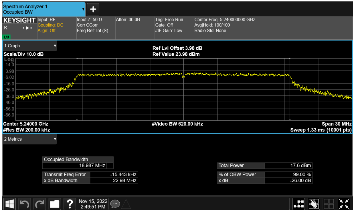
OBW NVNT ax20 5240MHz Ant24
