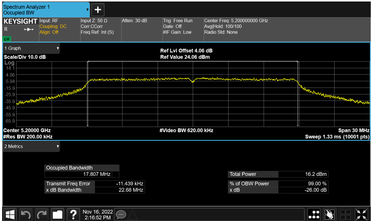
OBW NVNT ac20 5200MHz Ant24
