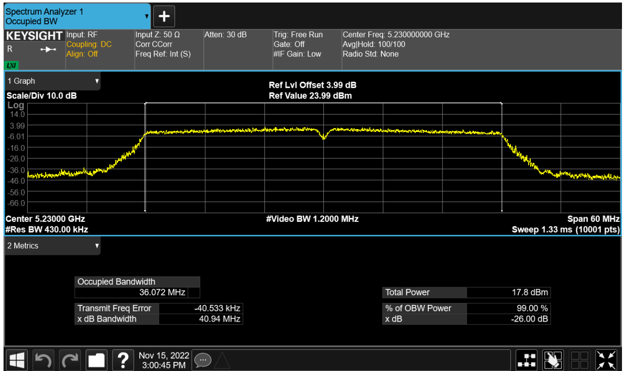
OBW NVNT ac40 5230MHz Ant24
