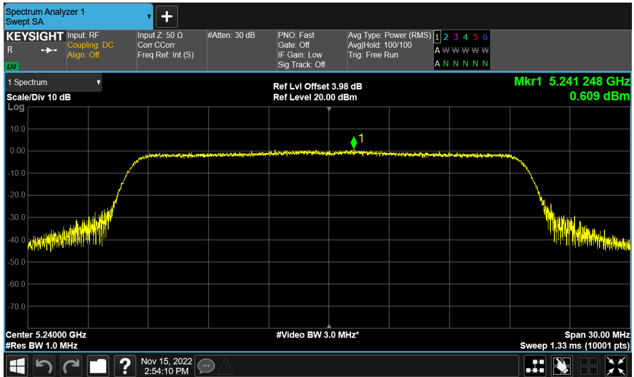
PSD NVNT ax20 5240MHz Ant24
