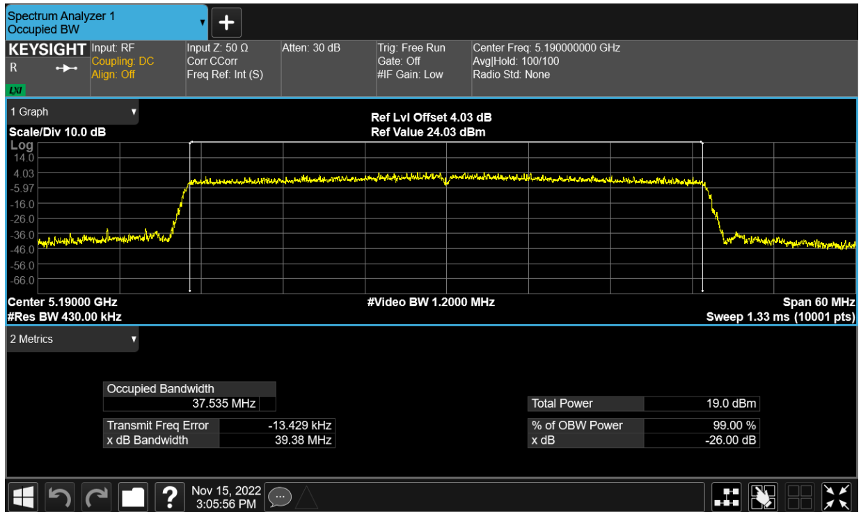
OBW NVNT ax40 5190MHz Ant24
