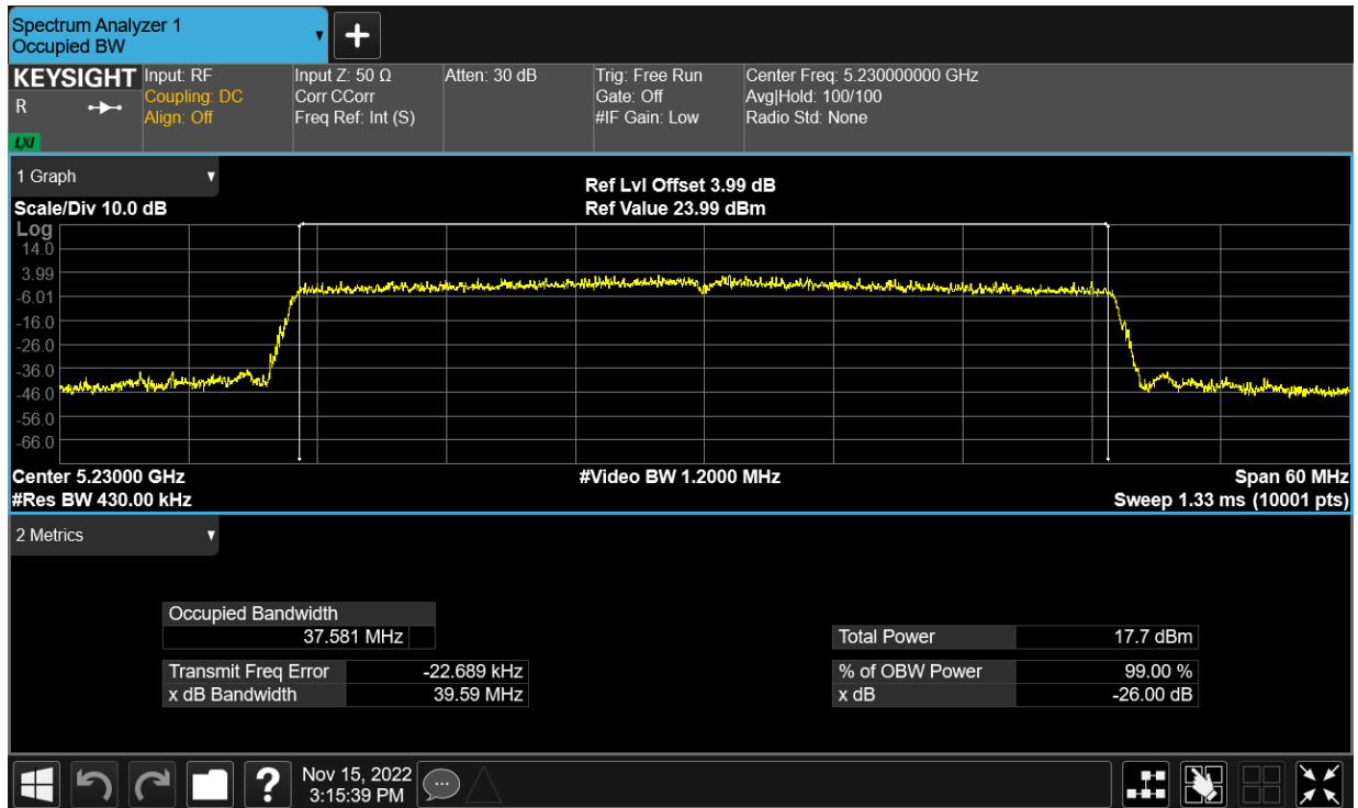
OBW NVNT ax40 5230MHz Ant24
