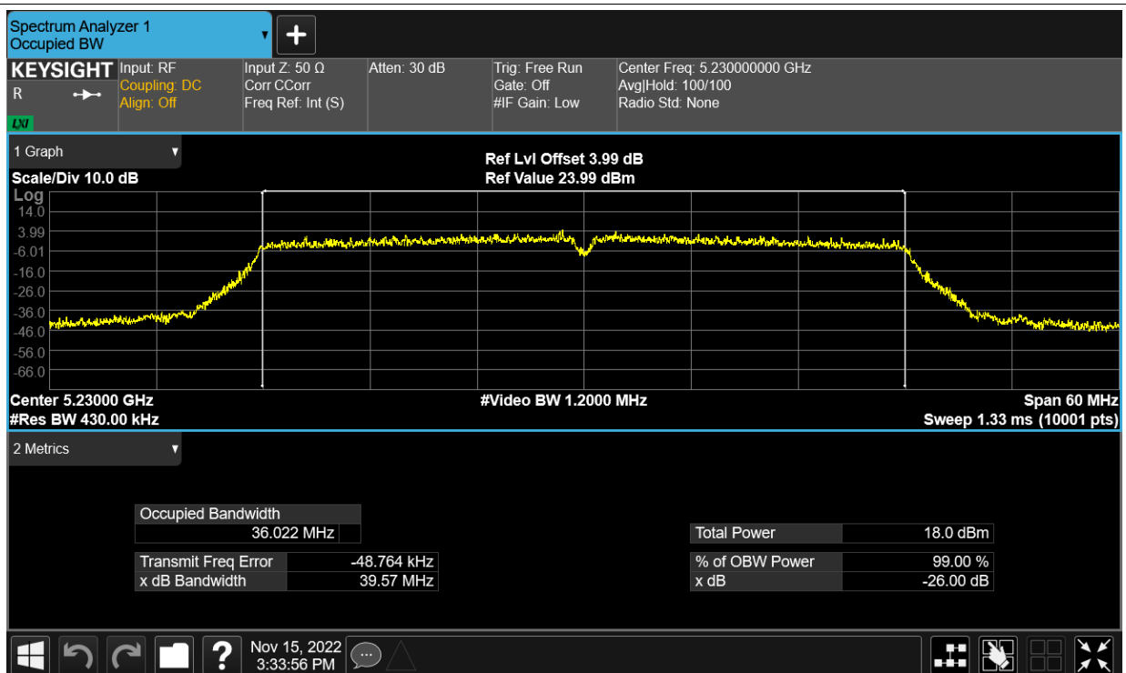
OBW NVNT n40 5230MHz Ant24
