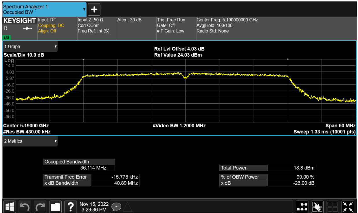
OBW NVNT n40 5190MHz Ant24
