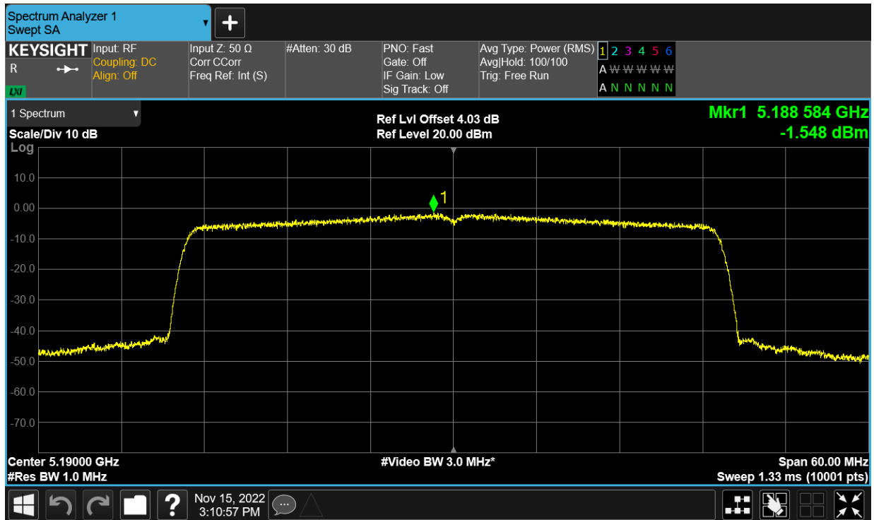
PSD NVNT ax40 5190MHz Ant24
