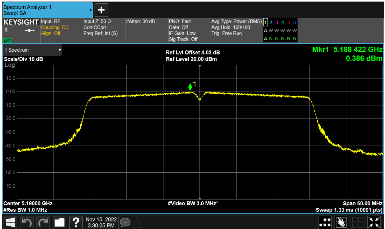
PSD NVNT n40 5190MHz Ant24
