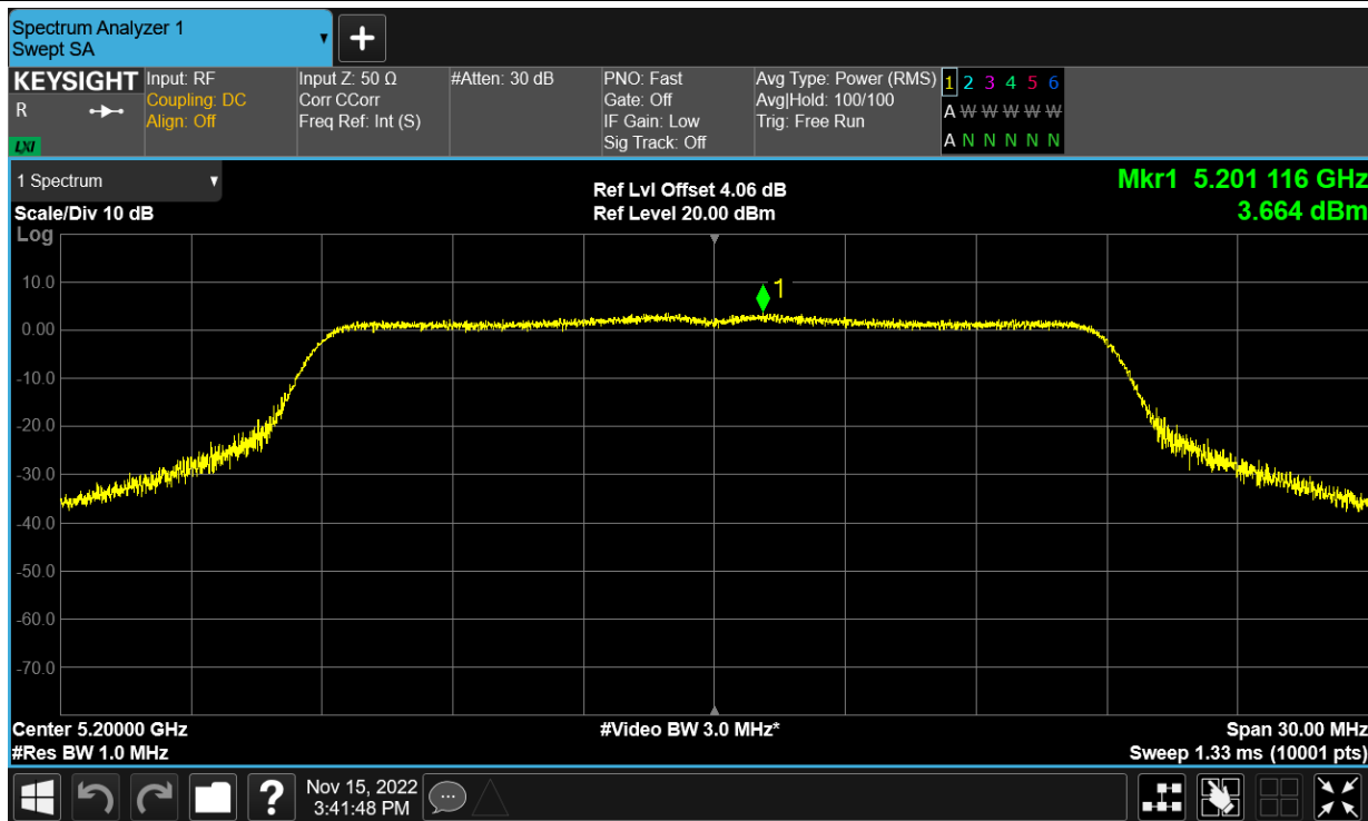
PSD NVNT n20 5200MHz Ant24
