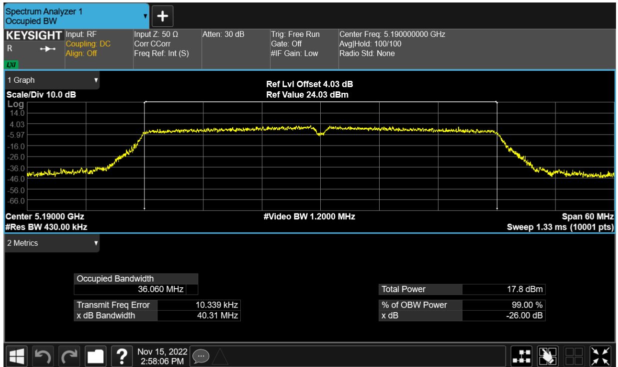
OBW NVNT ac40 5190MHz Ant24
