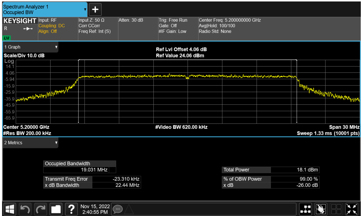
OBW NVNT ax20 5200MHz Ant24
