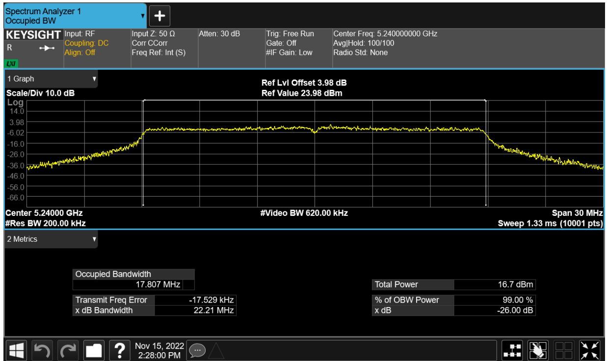
OBW NVNT ac20 5240MHz Ant24
