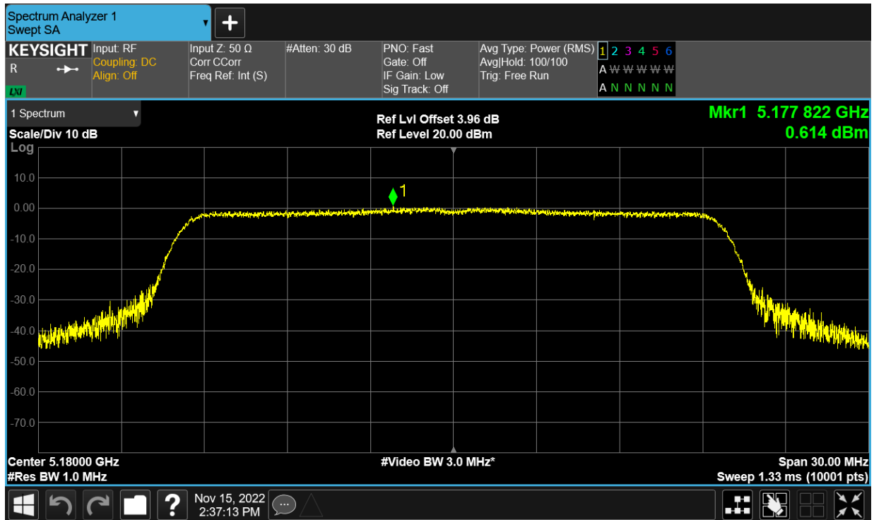
PSD NVNT ax20 5180MHz Ant24
