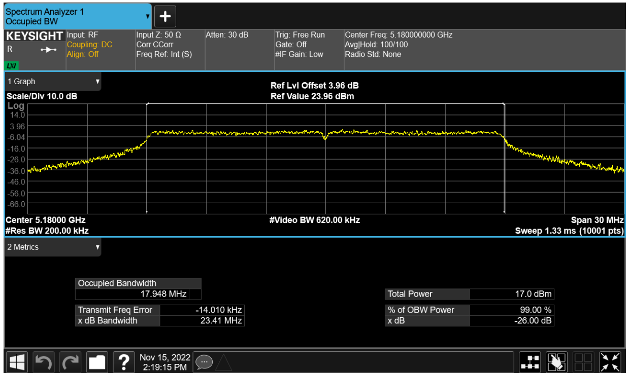
OBW NVNT ac20 5180MHz Ant24
