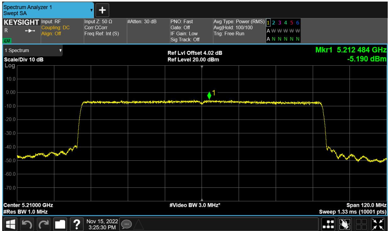
PSD NVNT ax80 5210MHz Ant24
