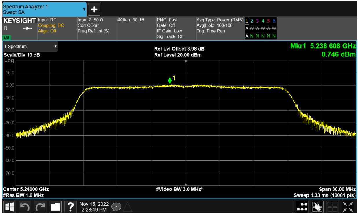
PSD NVNT ac20 5240MHz Ant24
