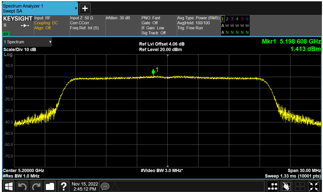
PSD NVNT ax20 5200MHz Ant24
