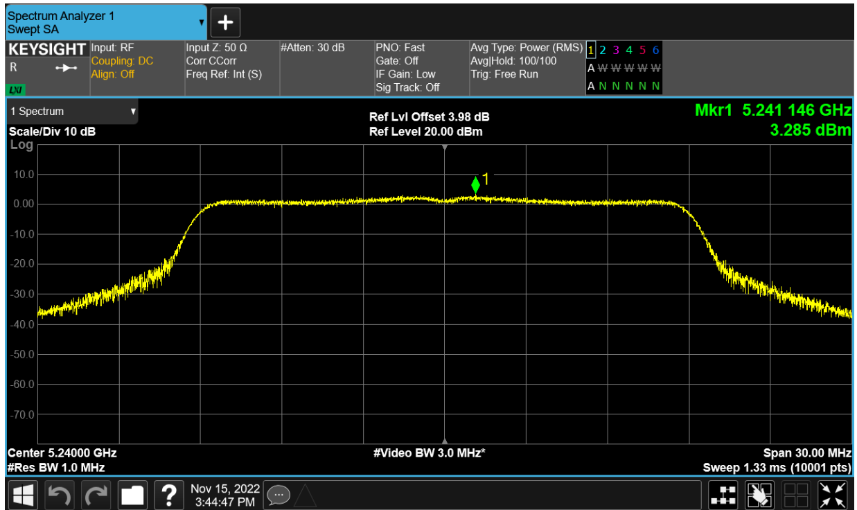
PSD NVNT n20 5240MHz Ant24
