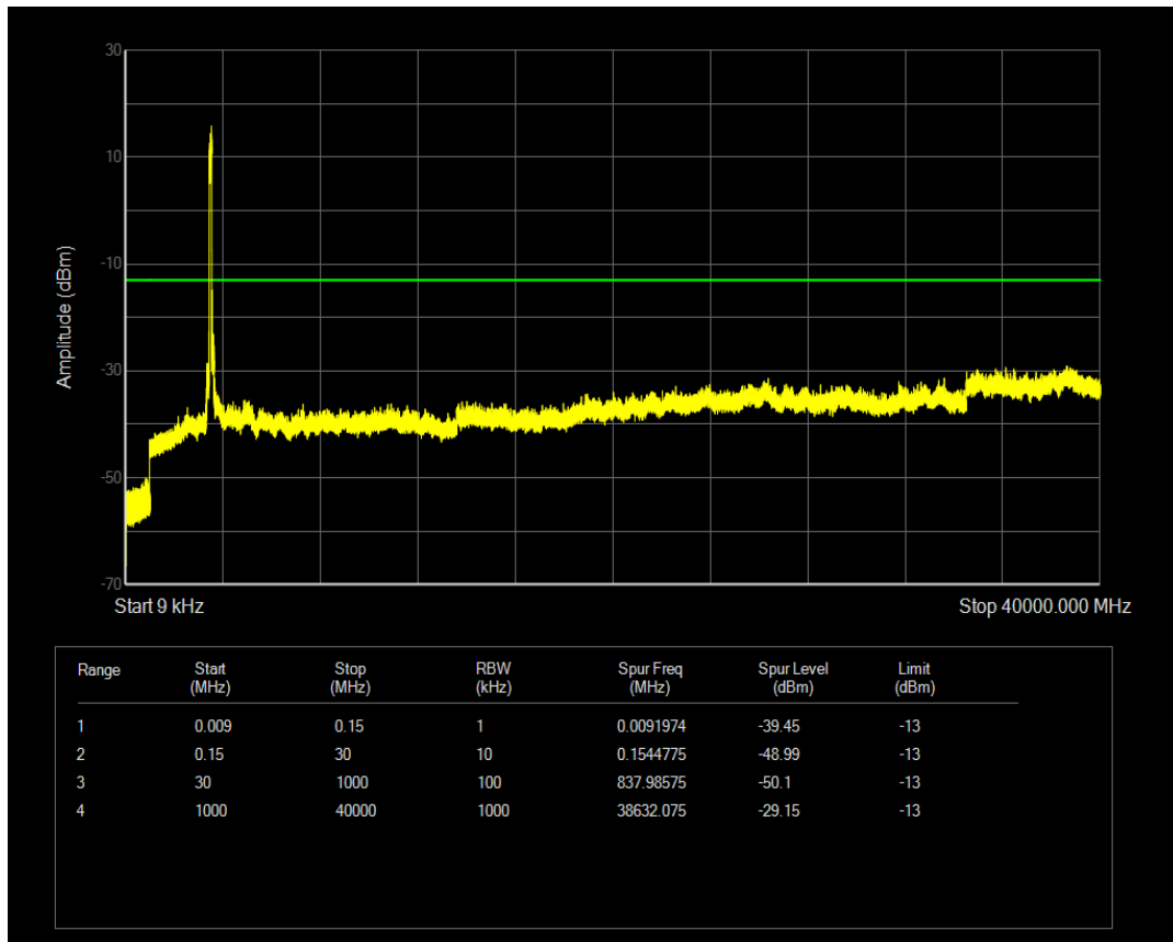
n77(3450-3550) SCS=30kHz DFT_QPSK BW=100MHz Channel=633334 RB=1@0
