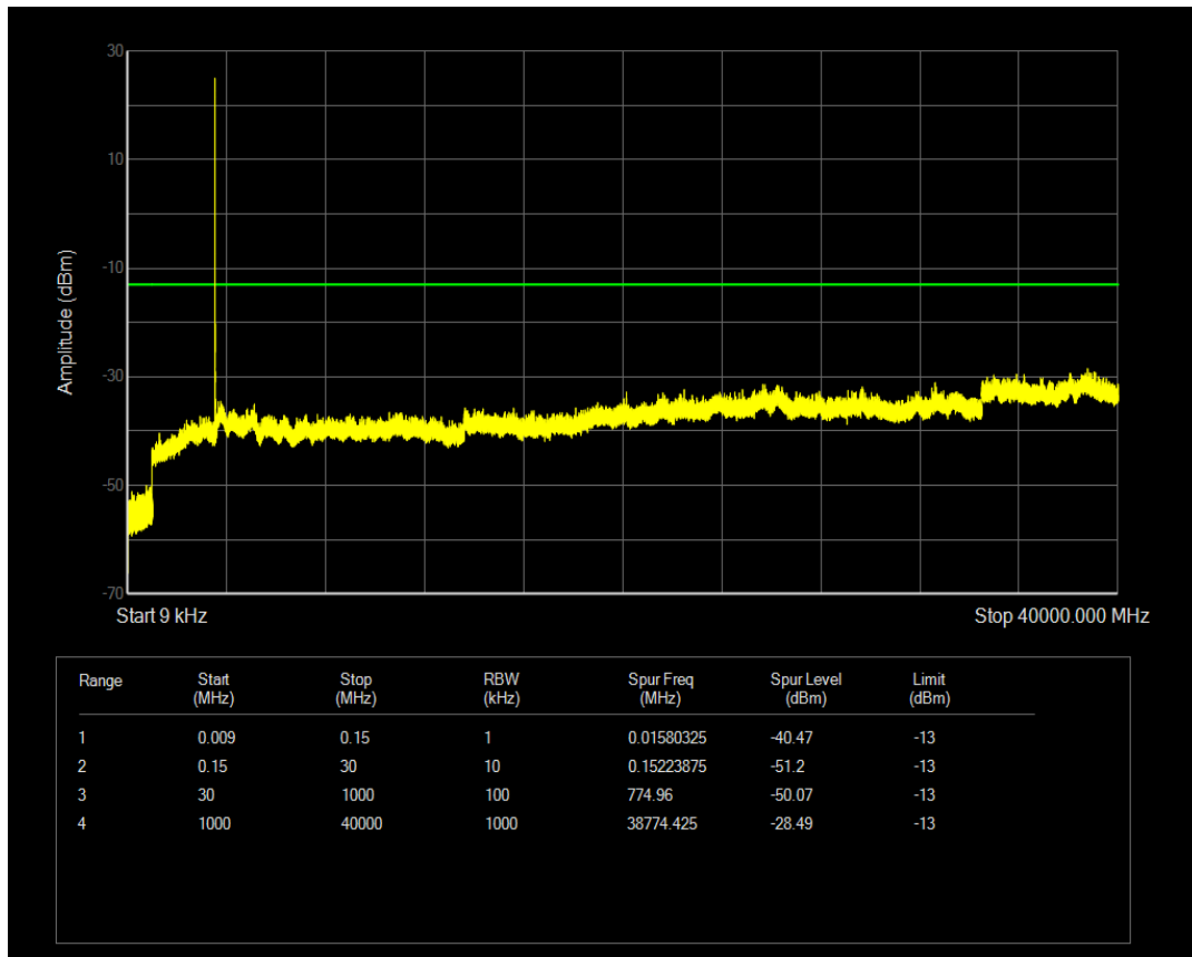
n77(3450-3550) SCS=30kHz DFT_QPSK BW=10MHz Channel=636332 RB=1@23
