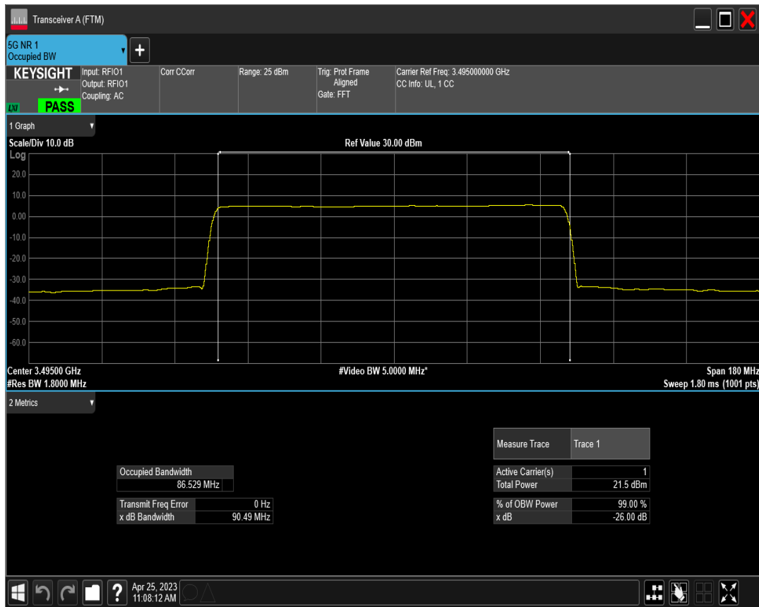
n77(3450-3550) SCS=30kHz CP_QPSK BW=90MHz Channel=633000 RB=245@0
