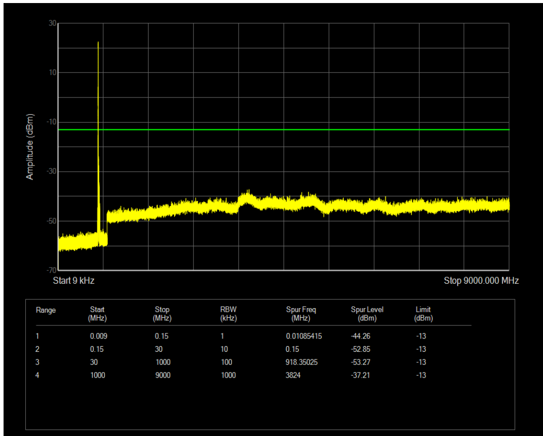
n5 SCS=30kHz DFT_QPSK BW=10MHz Channel=165800 RB=1@23
