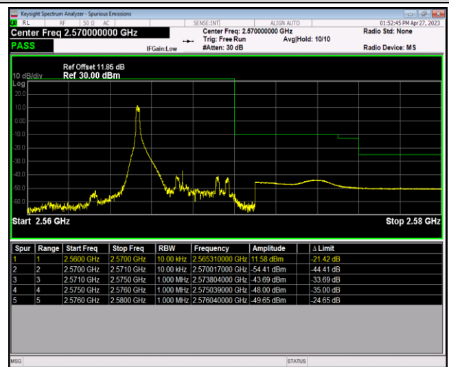
Band7-5MHz-64QAM-21425-25RB#0
