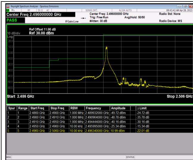
Band41-5MHz-QPSK-39675-25RB#0
