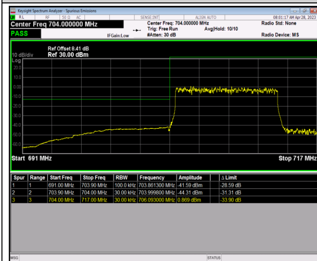
Band17-10MHz-64QAM-23800-1RB#49
