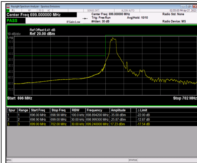
Band12-1.4MHz-64QAM-23017-6RB#0
