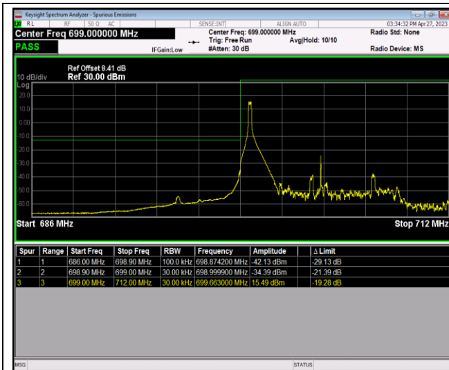
Band12-10MHz-64QAM-23060-50RB#0
