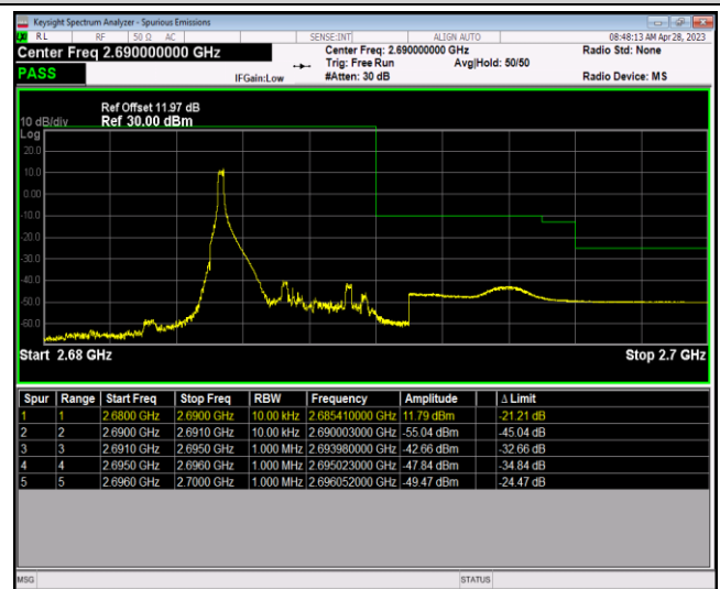
Band41-5MHz-QPSK-41565-25RB#0
