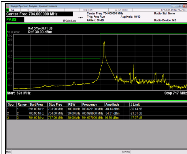
Band17-10MHz-64QAM-23780-50RB#0
