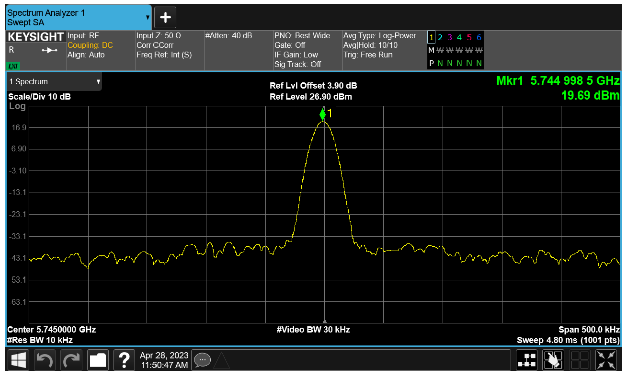
Freq. Stability HVNT a 5745MHz Ant10
