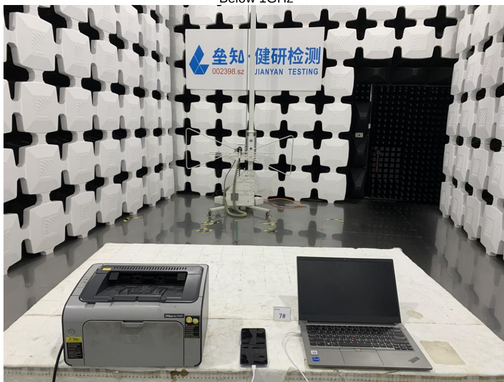
Unflip mode Radiated Spurious Emission Below 1GHz
