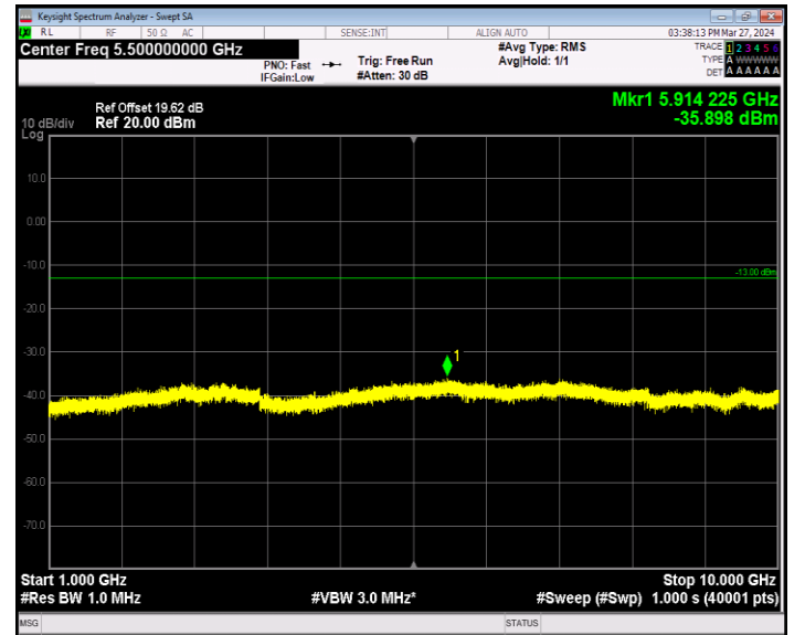
Band5_10MHz_64QAM_20600_1RB#0_1000~10000_1000~1000 0
