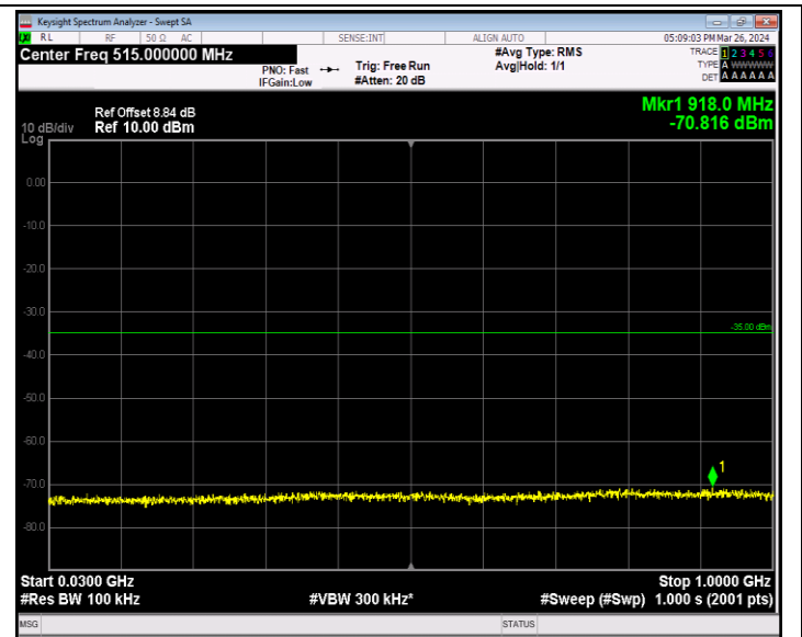
Band7_5MHz_64QAM_21100_1RB#0_30~1000_30~1000
