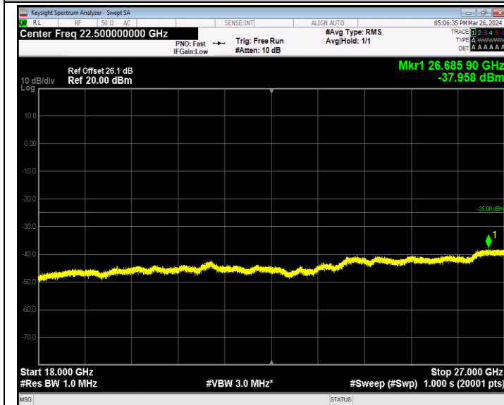
Band7_5MHz_QPSK_20775_1RB#0_18000~27000_18000~2700
