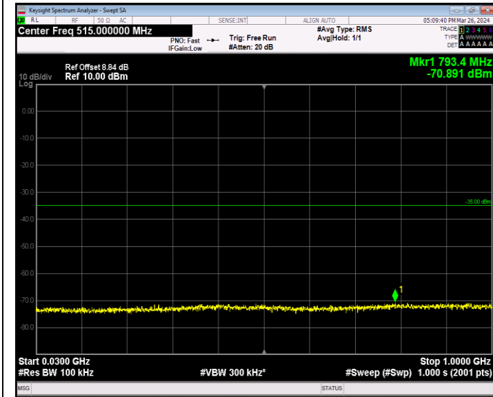
Band7_5MHz_QPSK_21425_1RB#0_30~1000_30~1000
