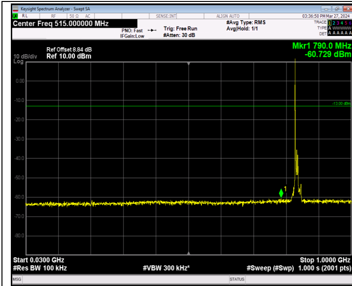
Band5_10MHz_64QAM_20525_1RB#0_30~1000_30~1000
