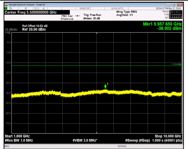
Band12_1.4MHz_QPSK_23173_1RB#0_1000~10000_1000~10000
