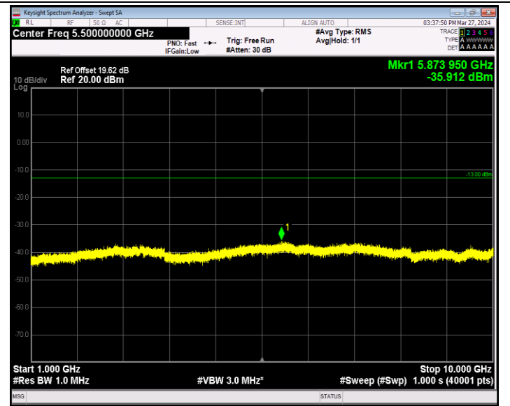
Band5_10MHz_16QAM_20600_1RB#0_1000~10000_1000~1000 0
