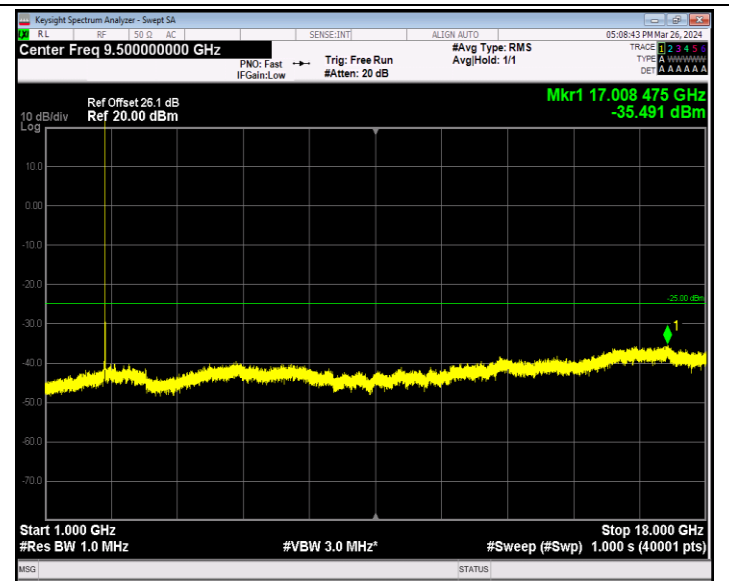
Band7_5MHz_16QAM_21100_1RB#0_1000~18000_1000~18000
