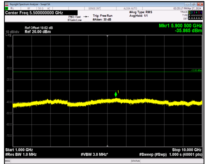
Band5_10MHz_64QAM_20450_1RB#0_1000~10000_1000~1000 0
