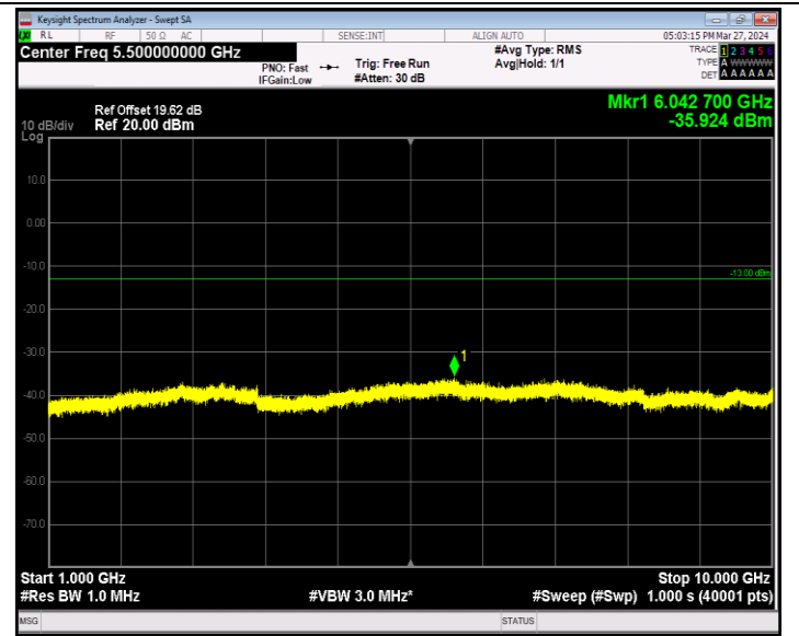
Band12_1.4MHz_QPSK_23095_1RB#0_1000~10000_1000~10000
