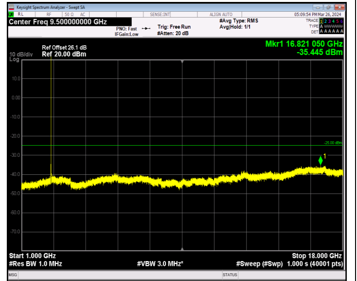
Band7_5MHz_QPSK_21425_1RB#0_1000~18000_1000~18000
