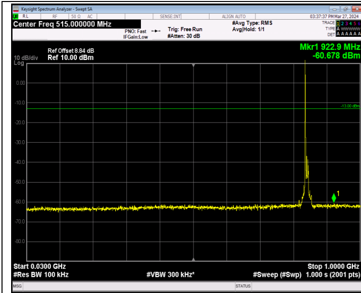
Band5_10MHz_16QAM_20600_1RB#0_30~1000_30~1000
