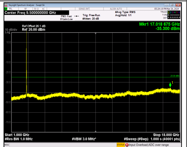
Band7_20MHz_QPSK_21100_1RB#0_1000~18000_1000~18000
