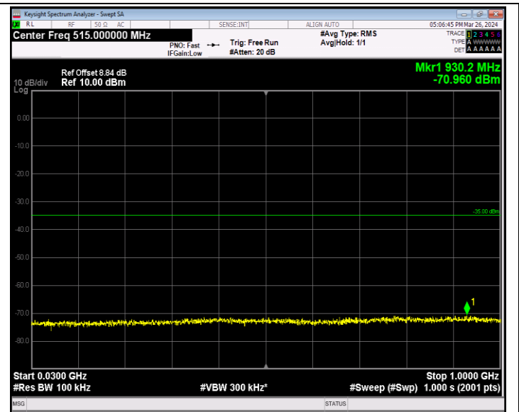
Band7_5MHz_16QAM_20775_1RB#0_30~1000_30~1000
