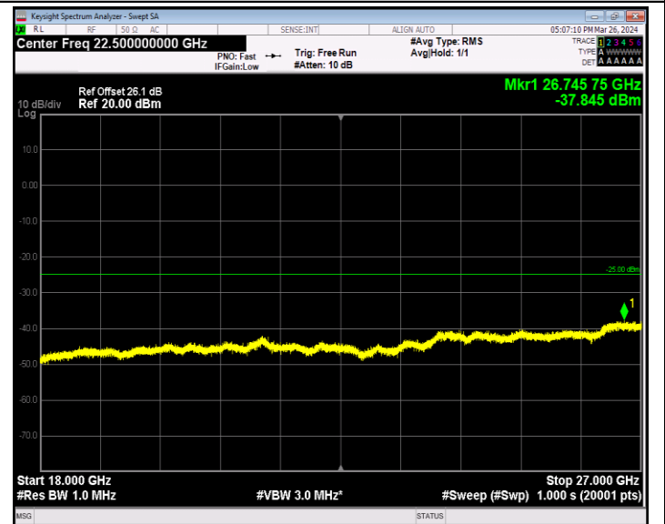
Band7_5MHz_16QAM_20775_1RB#0_18000~27000_18000~27000 00
