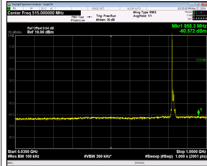
Band5_10MHz_64QAM_20450_1RB#0_30~1000_30~1000
