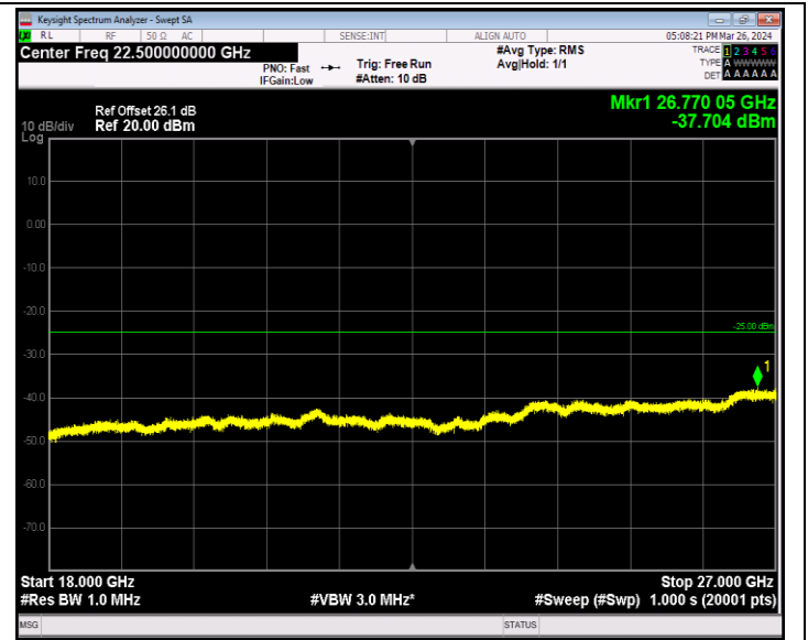
Band7_5MHz_QPSK_21100_1RB#0_18000~27000_18000~27000 0
