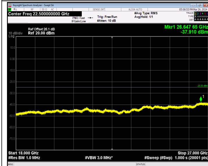
Band7_5MHz_16QAM_21100_1RB#0_18000~27000_18000~27000 00
