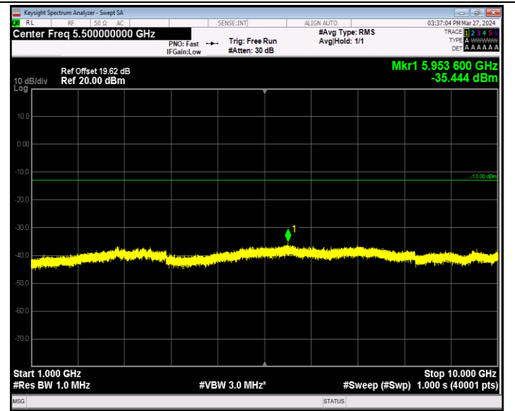
Band5_10MHz_64QAM_20525_1RB#0_1000~10000_1000~1000 0
