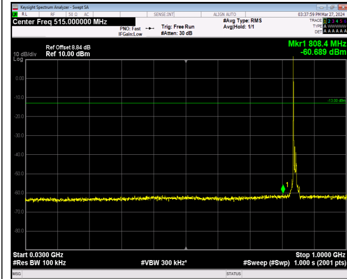
Band5_10MHz_64QAM_20600_1RB#0_30~1000_30~1000
