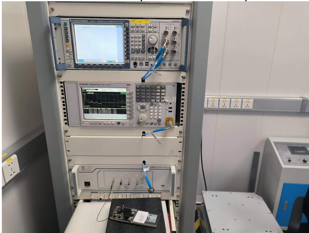
Conducted method(For 5G NR)
