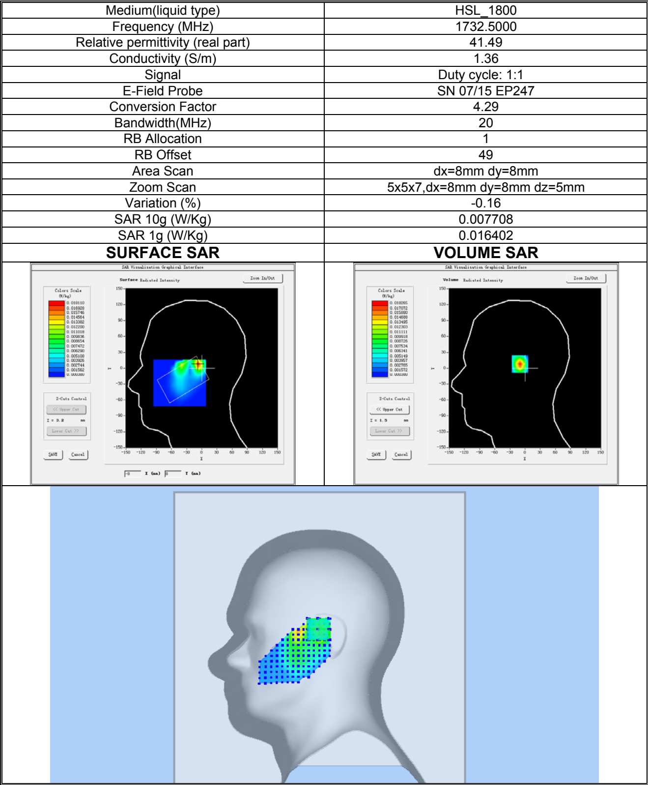
Plot 13:LTE BAND4, Middle channel (Right Head Cheek) Product Description:Mobile Phone Test Date: 2019-10-18
