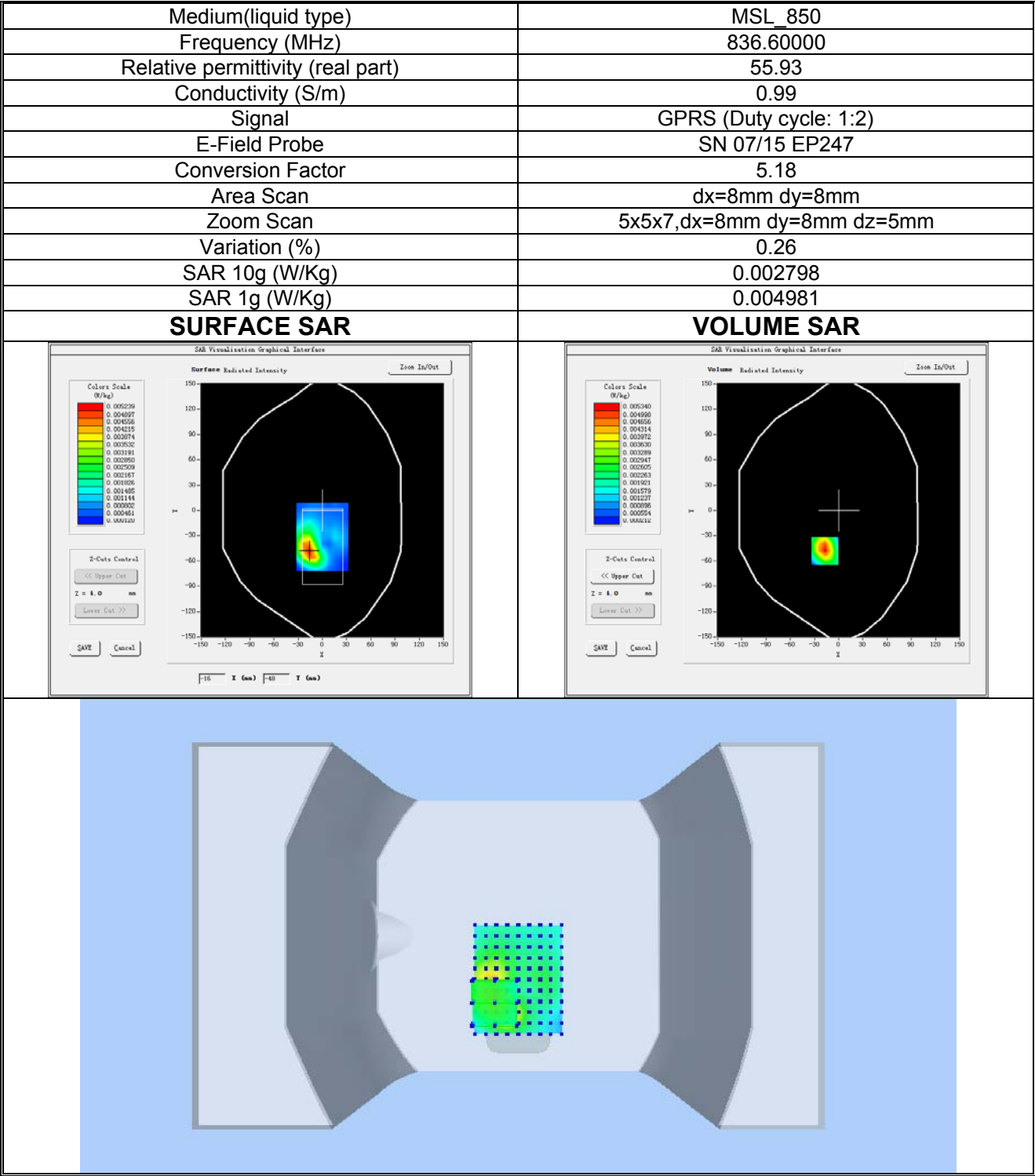
Plot 2: GPRS850MHz, Middle channel (Body-worn/Hotspot, Back Surface) Product Description:Mobile Phone Test Date: 2019-10-14
