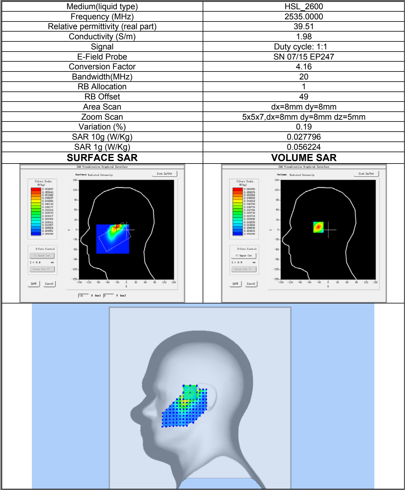
Plot 17:LTE BAND7, Middle channel (Right Head Cheek) Product Description:Mobile Phone Test Date: 2019-10-16
