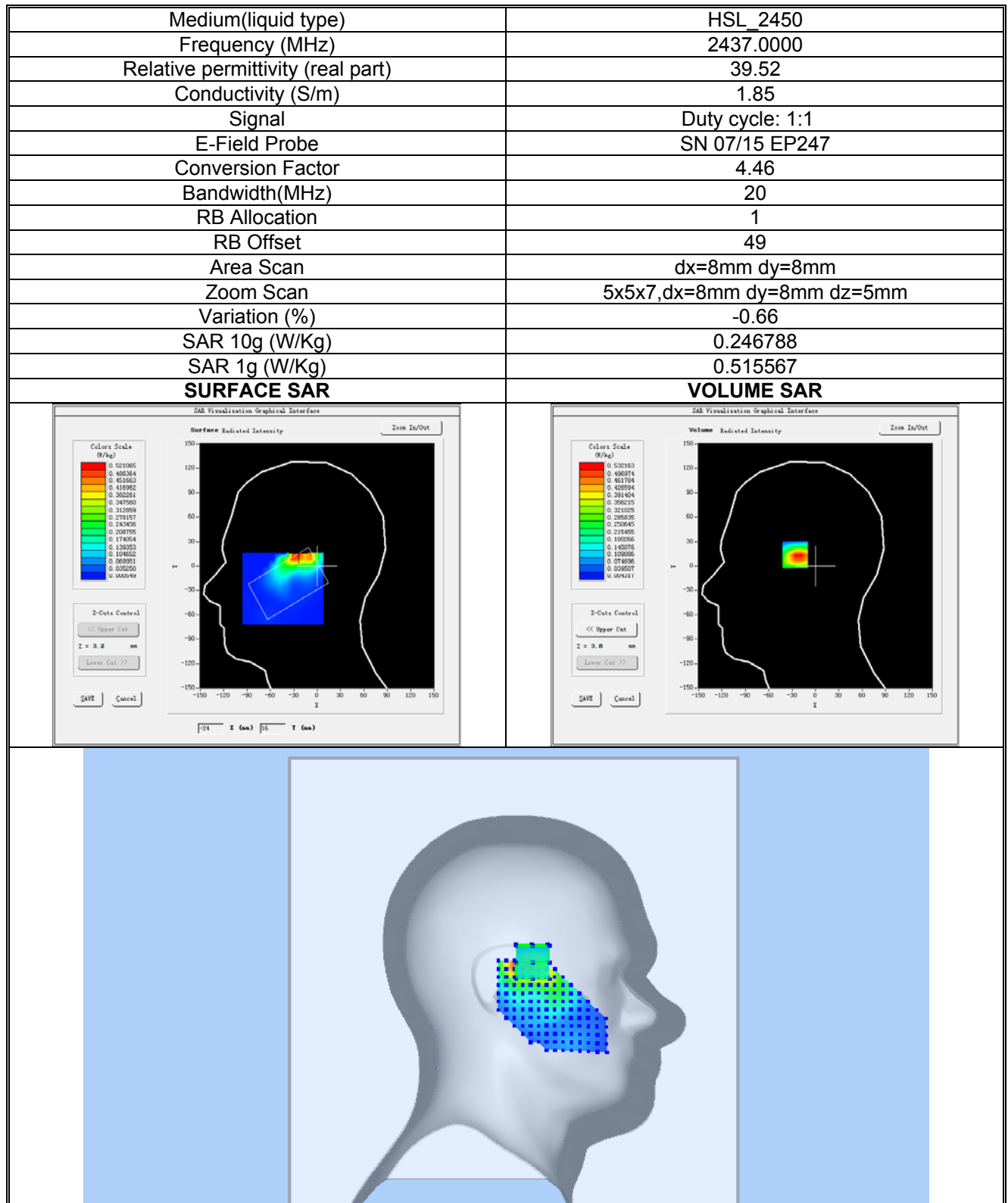
Plot 19:802.11b, Mid channel (Left Head Cheek) Product Description:Mobile Phone Test Date: 2019-10-15
