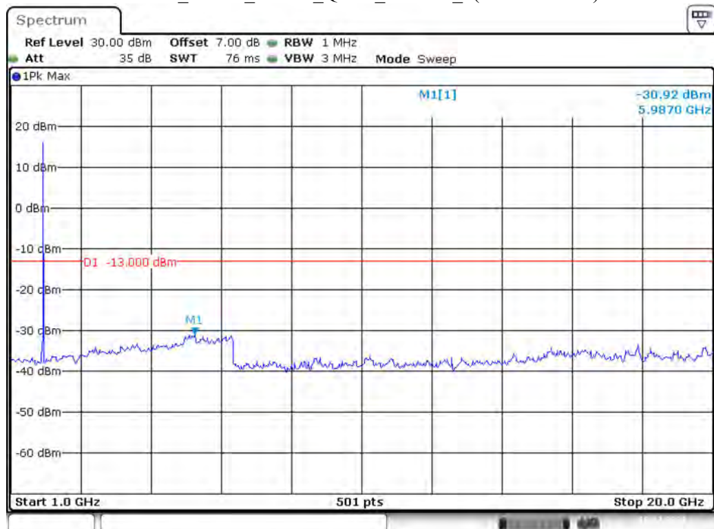
Band 2_5 MHz_Middle_QPSK_RB25#0_2(1GHz-20GHz)
