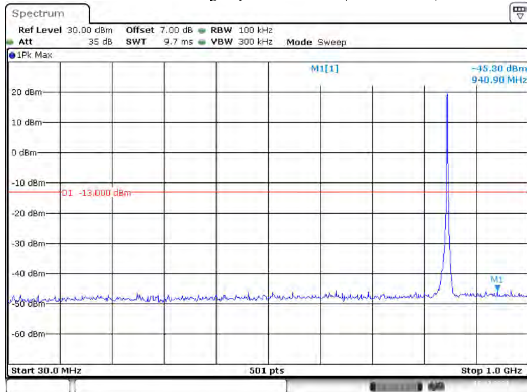
Band 5_3 MHz_High_QPSK_RB15#0_1(30MHz-1GHz)
