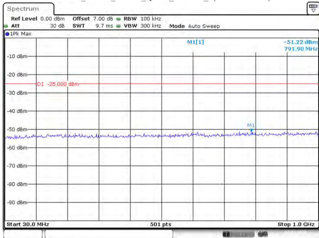
Band 41_5 MHz_Middle_QPSK_RB25#0_1(30MHz-1GHz)
