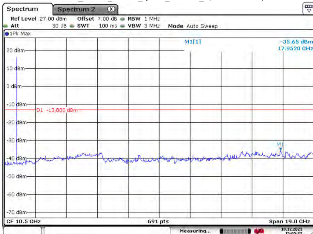
Band 4_3 MHz_Middle_QPSK_RB15#0_2(1GHz-20GHz)
