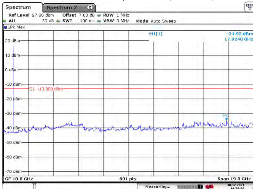
Band 4_1.4 MHz_Middle_QPSK_RB6#0_2(1GHz-20GHz)
