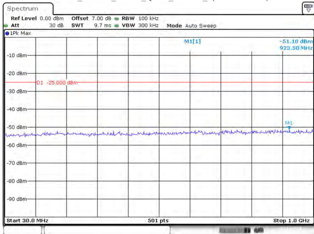
Band 38_10 MHz_Middle_QPSK_RB50#0_1(30MHz-1GHz)
