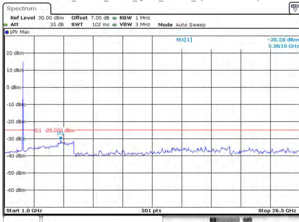
Band 41_15 MHz_Middle_QPSK_RB75#0_2(1GHz-26.5GHz)
