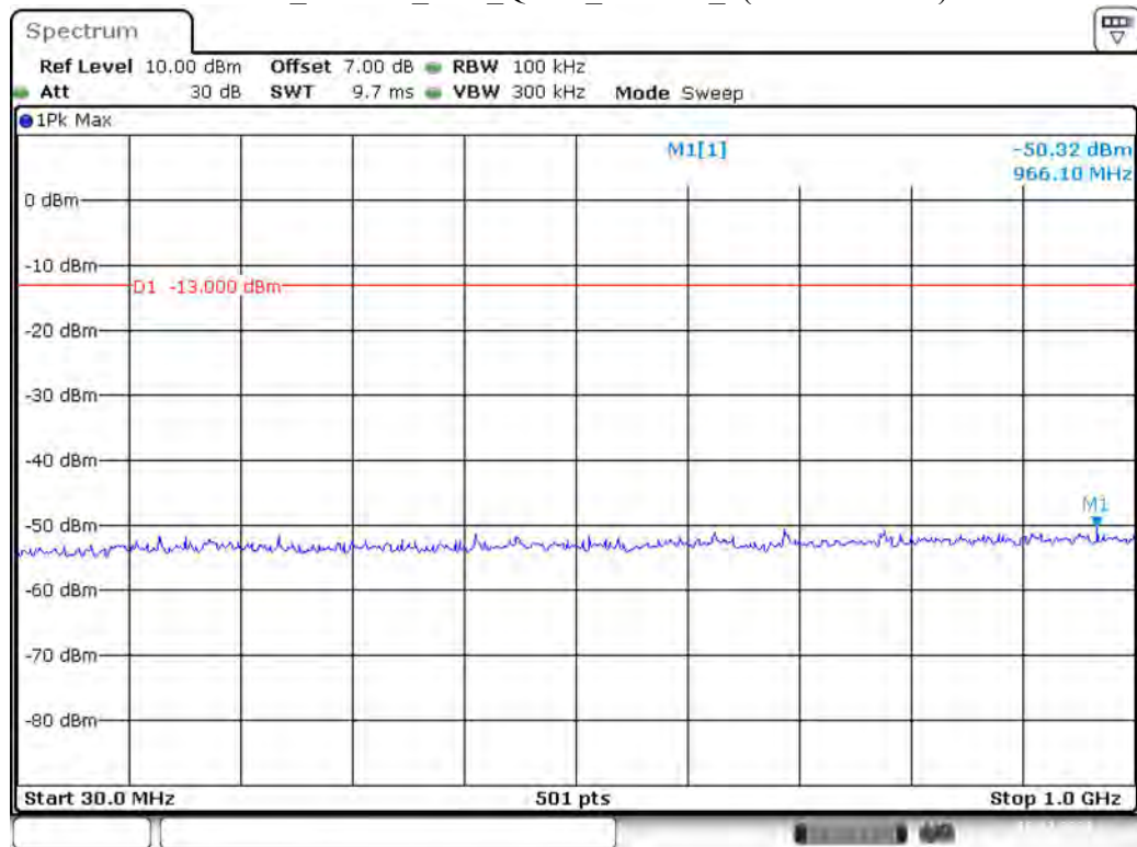
Band 4_10 MHz_Low_QPSK_RB50#0_1(30MHz-1GHz)
