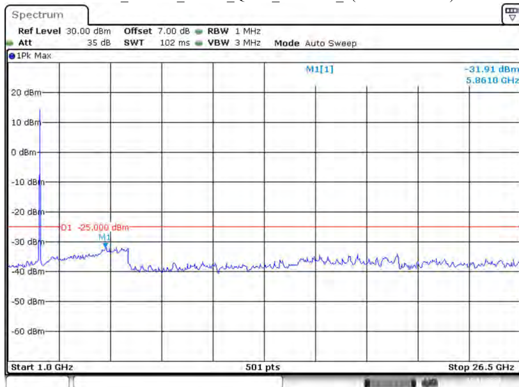
Band 41_20 MHz_Middle_QPSK_RB100#0_2(1GHz-26.5GHz)
