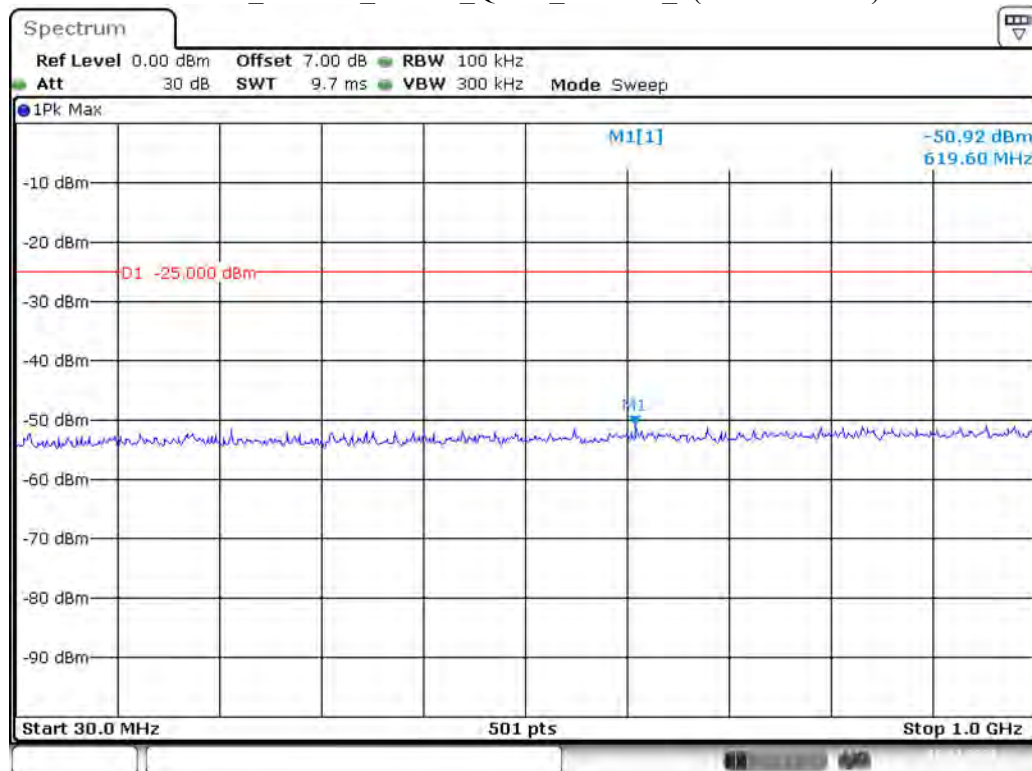
Band 7_10 MHz_Middle_QPSK_RB50#0_1(30MHz-1GHz)
