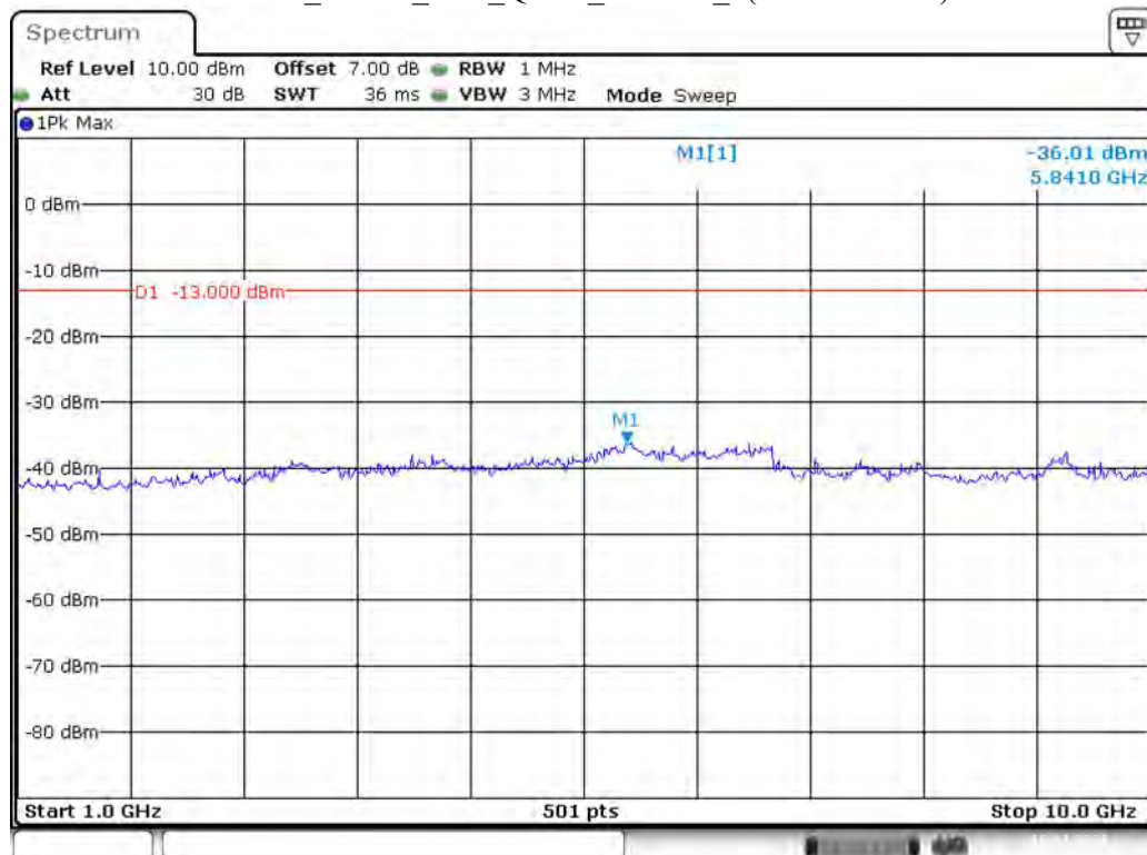
Band 5_5 MHz_Low_QPSK_RB25#0_2(1GHz-10GHz)
