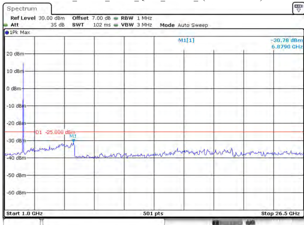
Band 38_15 MHz_Middle_QPSK_RB75#0_2(1GHz-26.5GHz)
