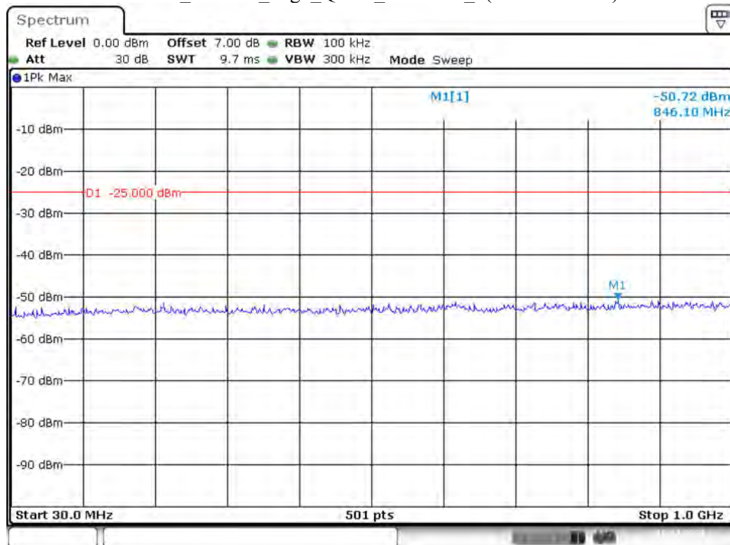
Band 7_20 MHz_High_QPSK_RB100#0_1(30MHz-1GHz)
