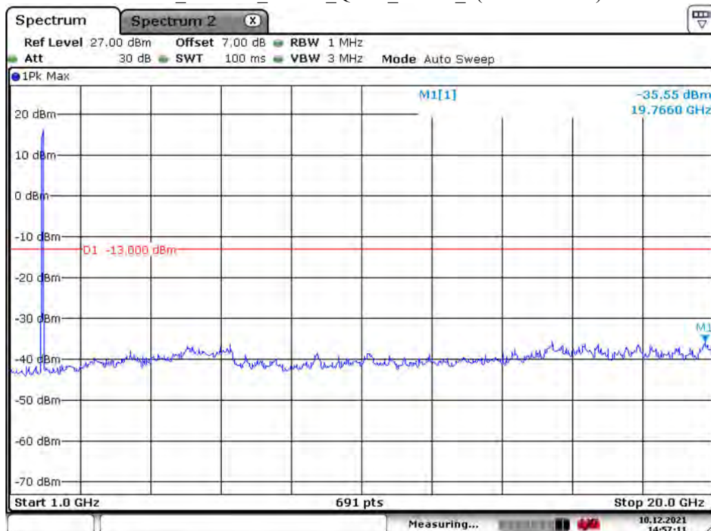
Band 2_1.4 MHz_Middle_QPSK_RB6#0_2(1GHz-20GHz)
