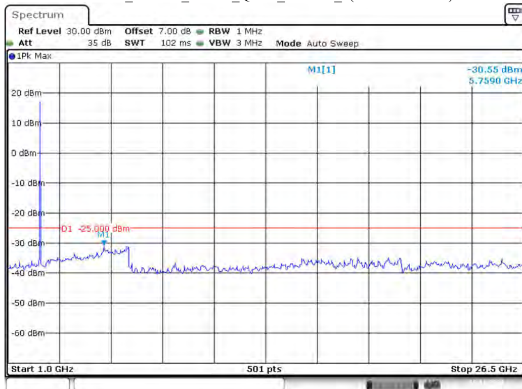
Band 41_10 MHz_Middle_QPSK_RB50#0_2(1GHz-26.5GHz)
