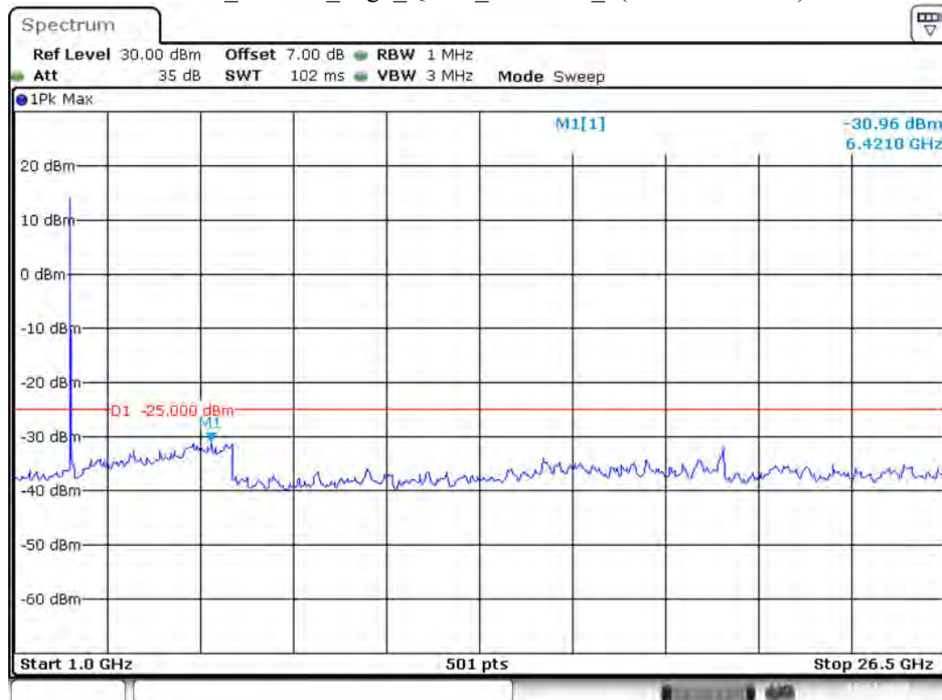
Band 7_20 MHz_High_QPSK_RB100#0_2(1GHz-26.5GHz)
