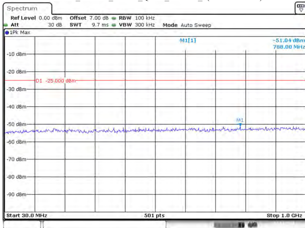
Band 41_15 MHz_Middle_QPSK_RB75#0_1(30MHz-1GHz)
