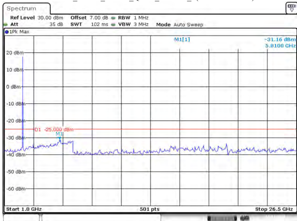
Band 41_5 MHz_Middle_QPSK_RB25#0_2(1GHz-26.5GHz)
