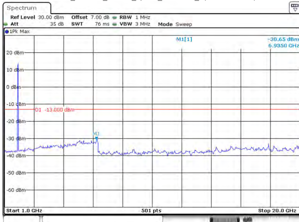
Band 2_20 MHz_Middle_QPSK_RB100#0_2(1GHz-20GHz)
