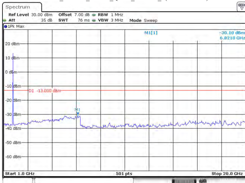
Band 4_15 MHz_Middle_QPSK_RB75#0_2(1GHz-20GHz)
