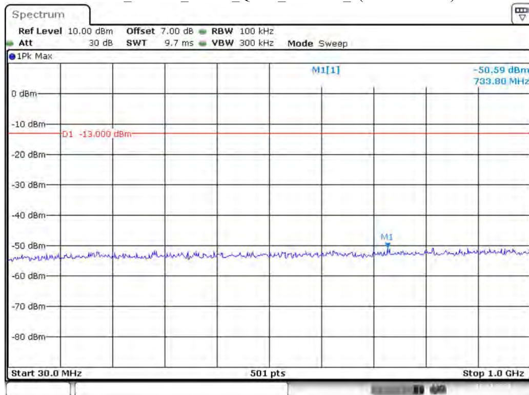
Band 2_20 MHz_Middle_QPSK_RB100#0_1(30MHz-1GHz)
