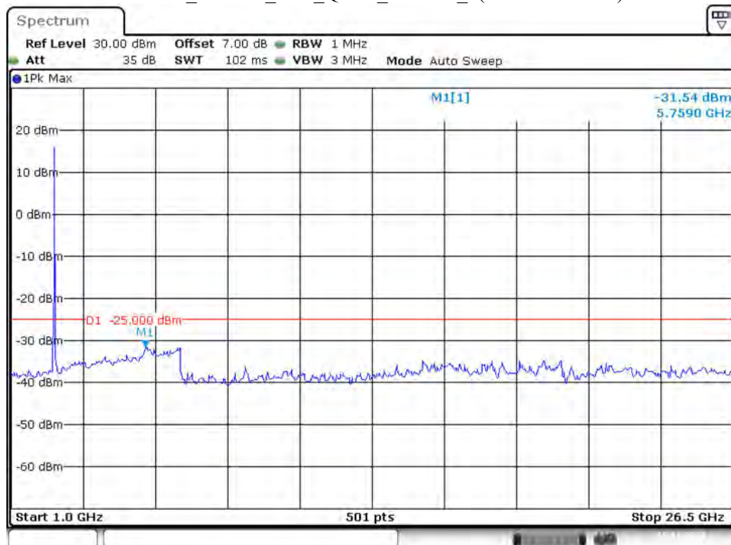
Band 41_15 MHz_Low_QPSK_RB75#0_2(1GHz-26.5GHz)
