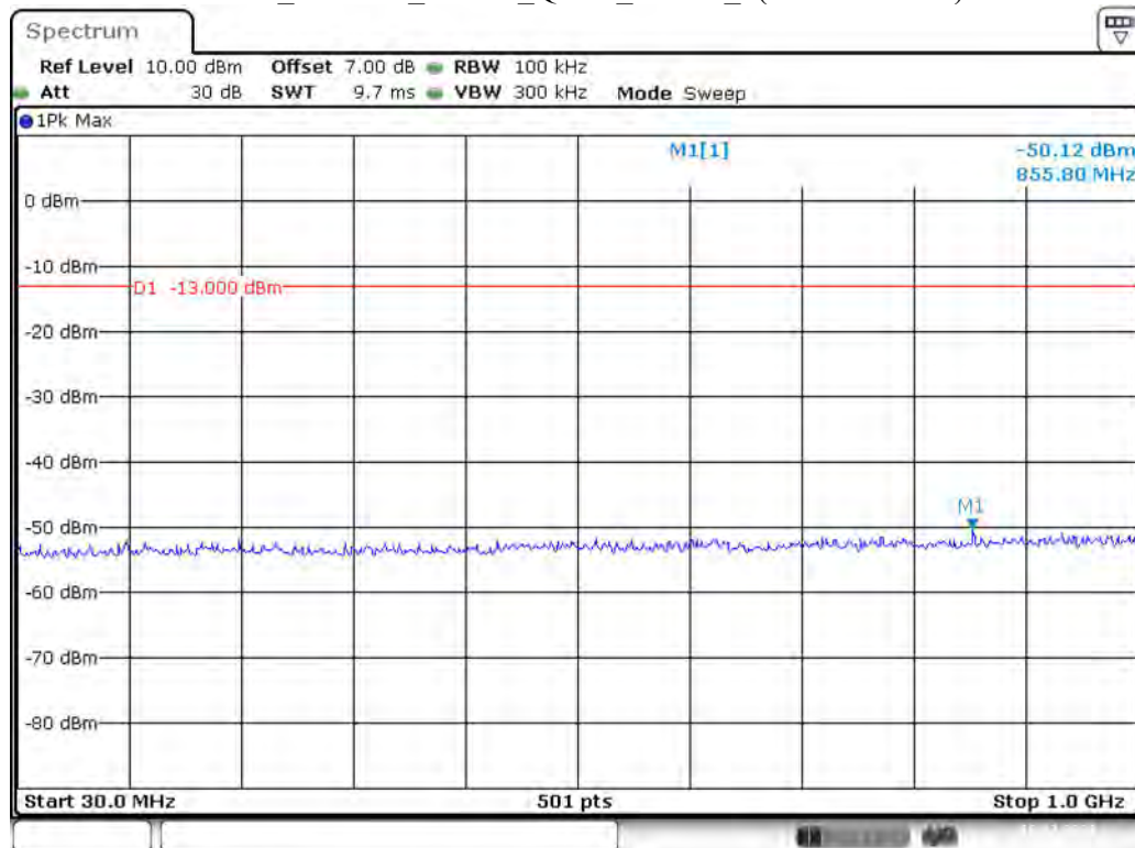
Band 4_1.4 MHz_Middle_QPSK_RB6#0_1(30MHz-1GHz)
