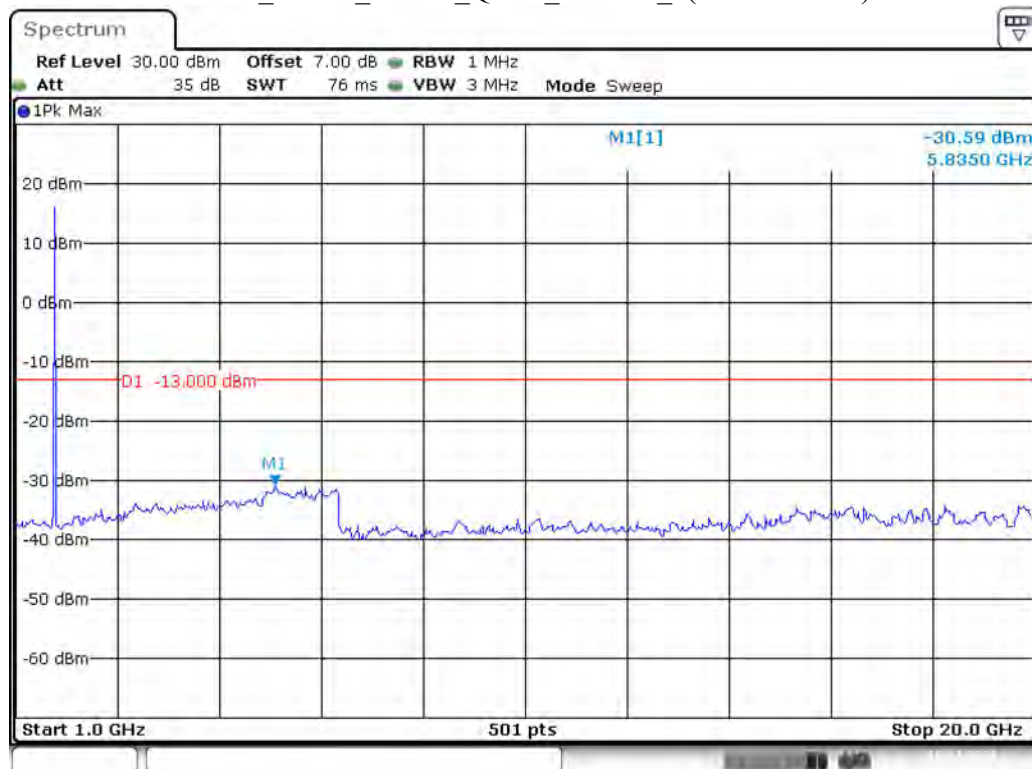
Band 4_5 MHz_Middle_QPSK_RB25#0_2(1GHz-20GHz)
