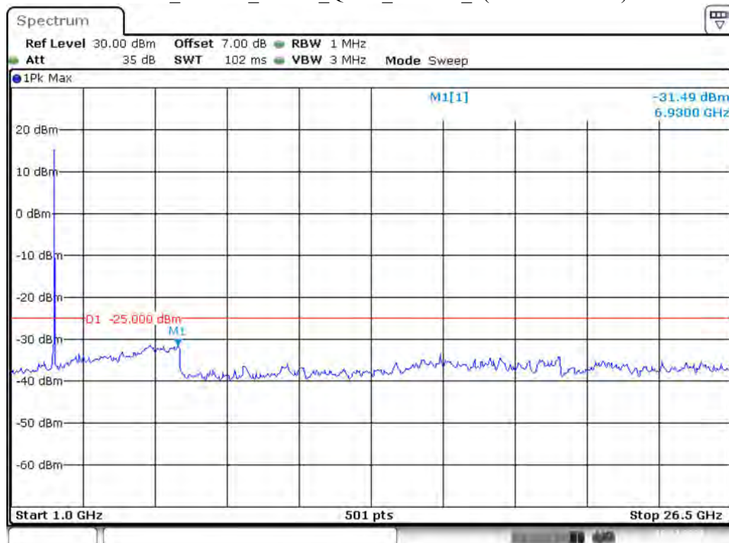
Band 7_10 MHz_Middle_QPSK_RB50#0_2(1GHz-26.5GHz)
