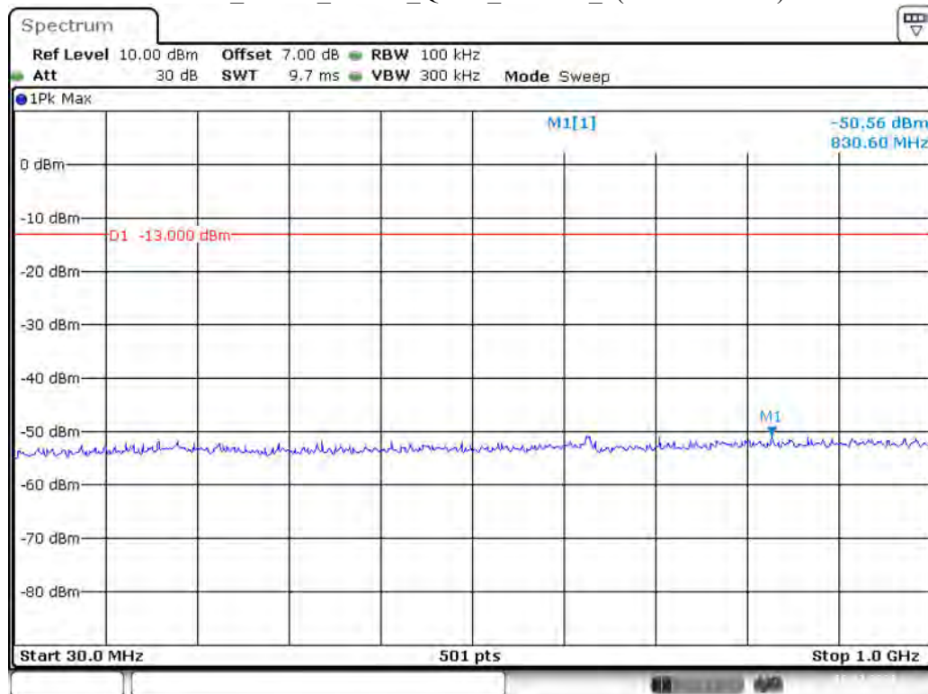
Band 4_3 MHz_Middle_QPSK_RB15#0_1(30MHz-1GHz)
