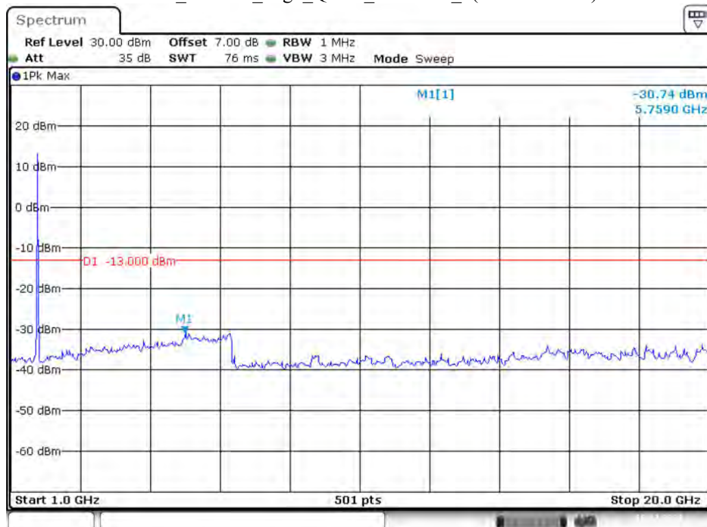
Band 4_20 MHz_High_QPSK_RB100#0_2(1GHz-20GHz)
