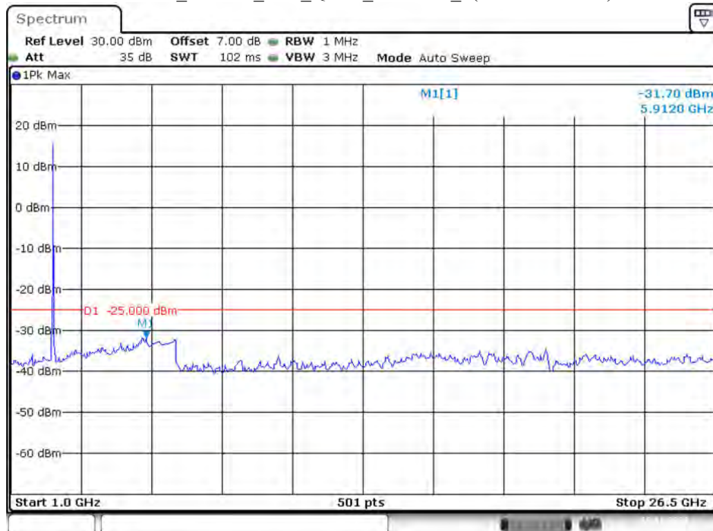
Band 41_20 MHz_Low_QPSK_RB100#0_2(1GHz-26.5GHz)
