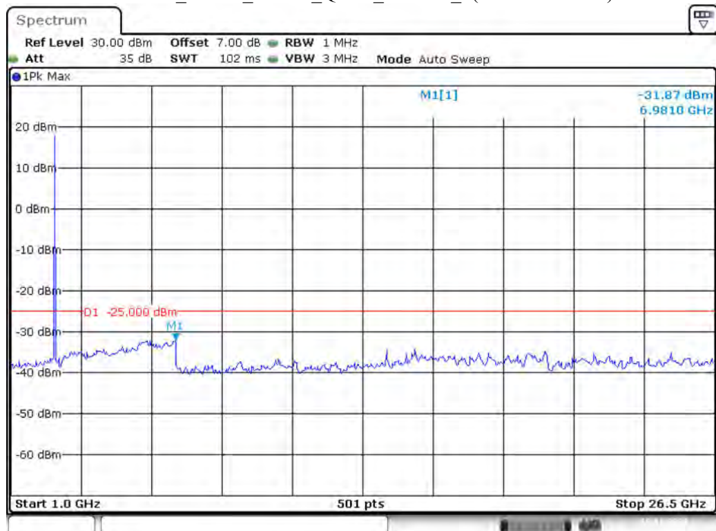
Band 38_5 MHz_Middle_QPSK_RB25#0_2(1GHz-26.5GHz)
