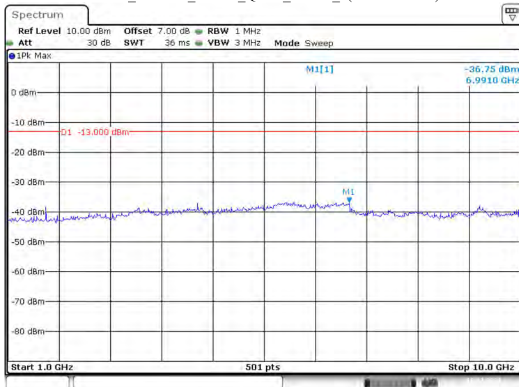
Band 5_1.4 MHz_Middle_QPSK_RB6#0_2(1GHz-10GHz)
