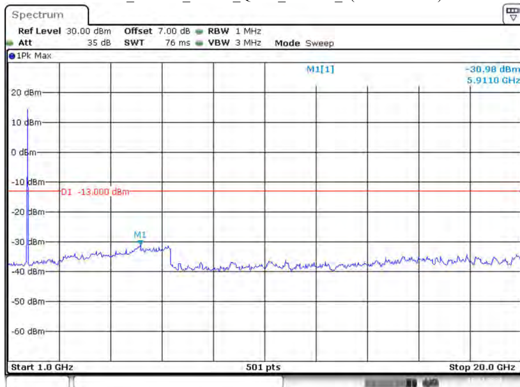
Band 4_10 MHz_Middle_QPSK_RB50#0_2(1GHz-20GHz)
