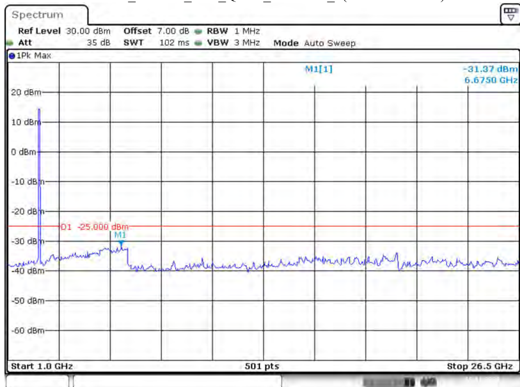
Band 38_20 MHz_Low_QPSK_RB100#0_2(1GHz-26.5GHz)
