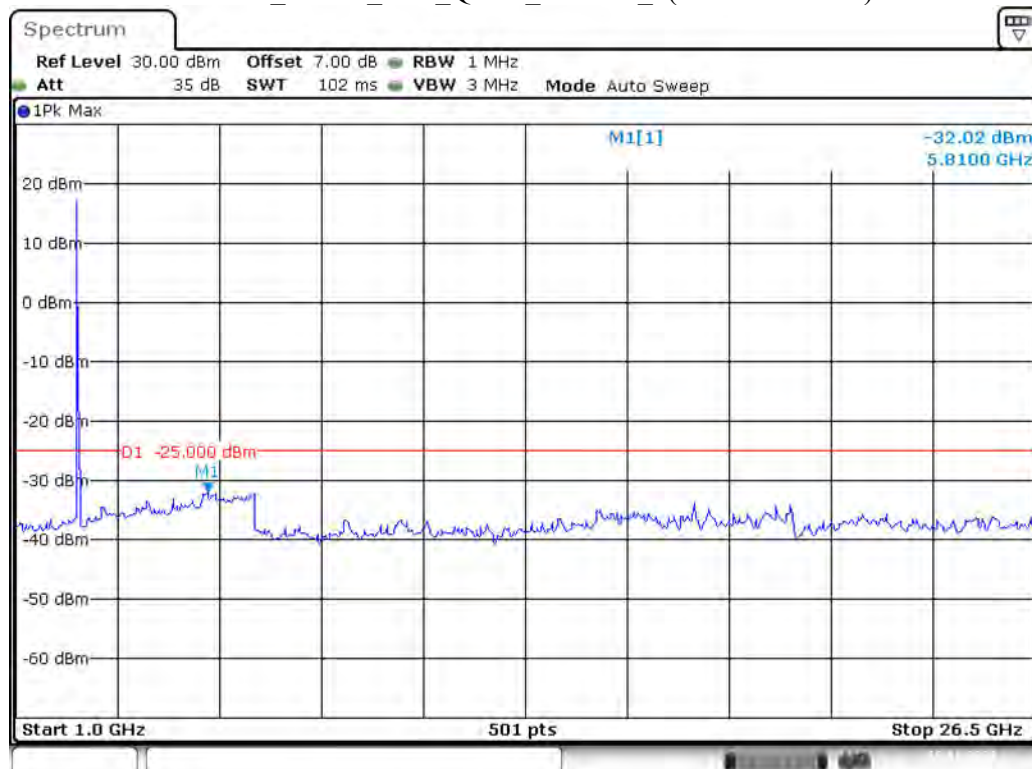
Band 38_5 MHz_Low_QPSK_RB25#0_2(1GHz-26.5GHz)
