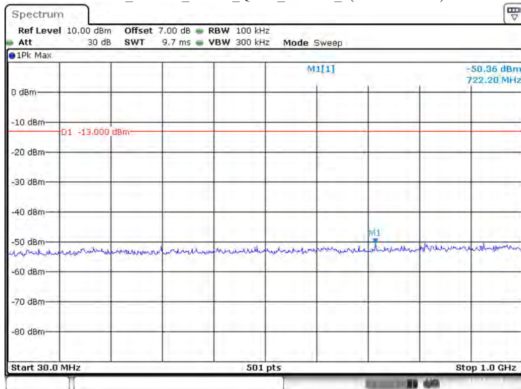
Band 4_15 MHz_Middle_QPSK_RB75#0_1(30MHz-1GHz)
