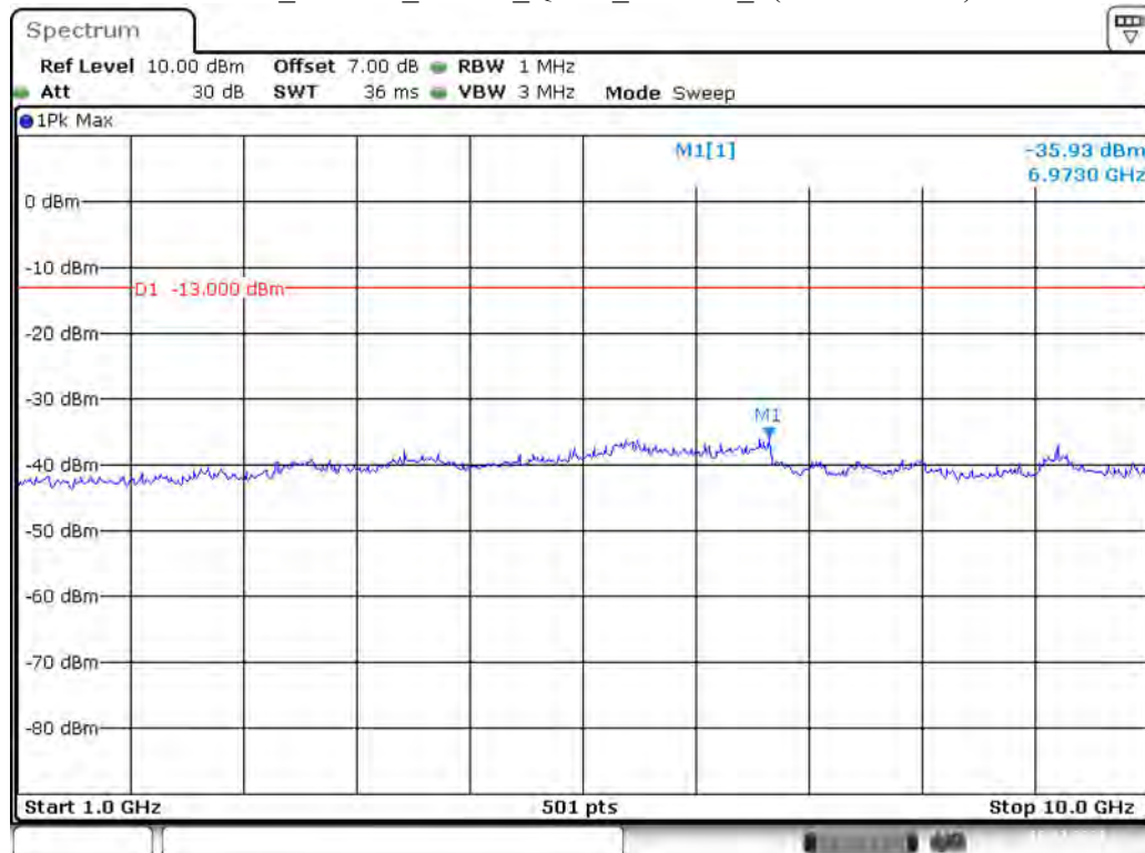
Band 5_10 MHz_Middle_QPSK_RB50#0_2(1GHz-10GHz)
