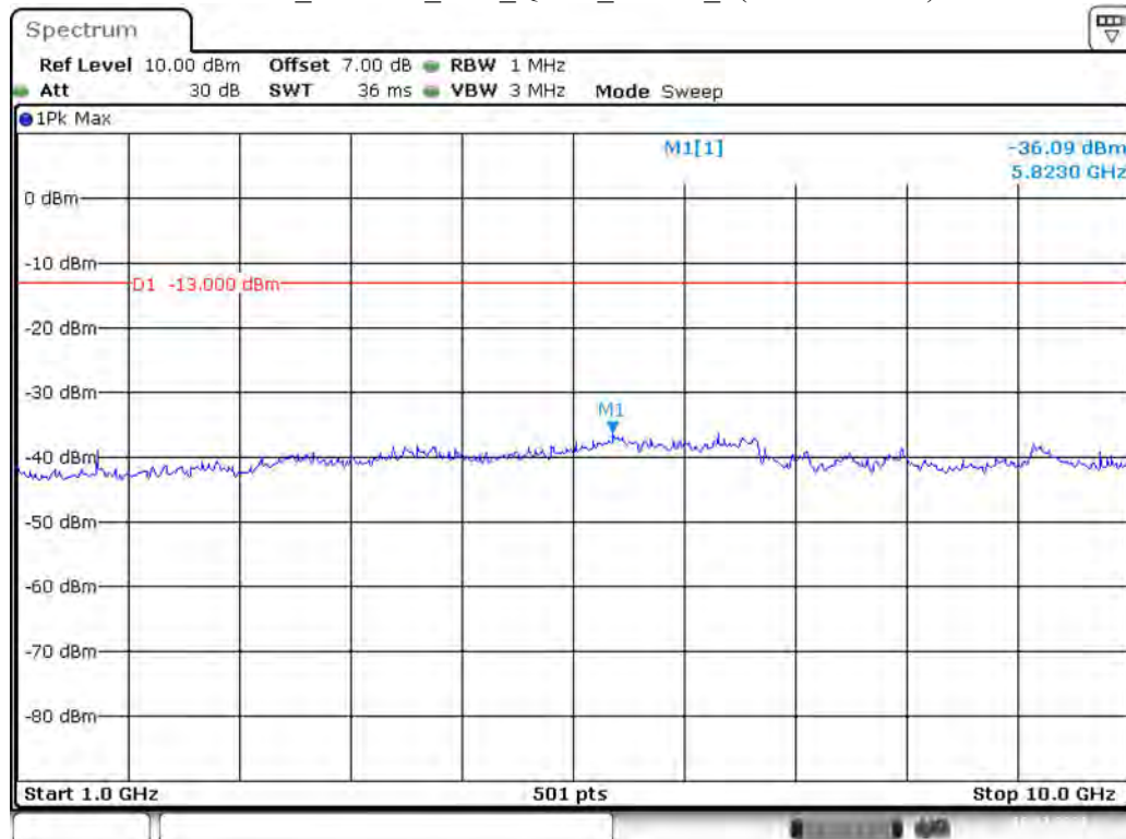
Band 5_1.4 MHz_Low_QPSK_RB6#0_2(1GHz-10GHz)
