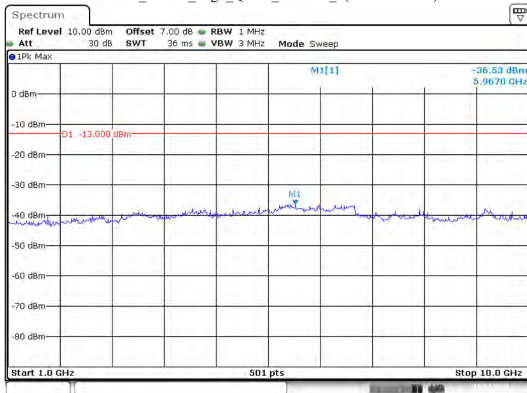
Band 5_3 MHz_High_QPSK_RB15#0_2(1GHz-10GHz)
