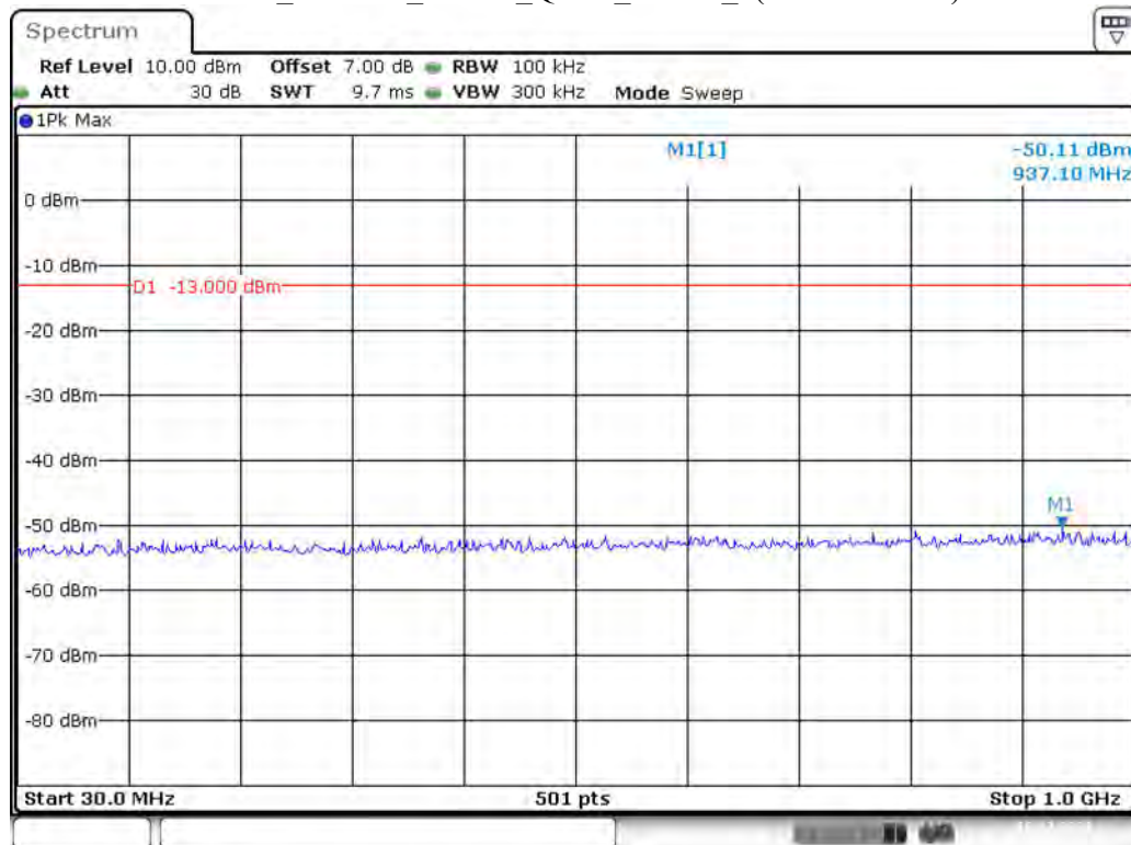
Band 2_1.4 MHz_Middle_QPSK_RB6#0_1(30MHz-1GHz)
