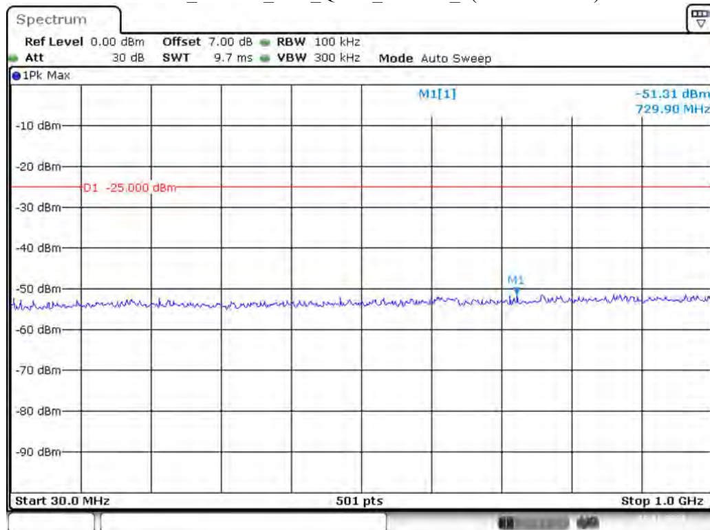
Band 41_15 MHz_Low_QPSK_RB75#0_1(30MHz-1GHz)
