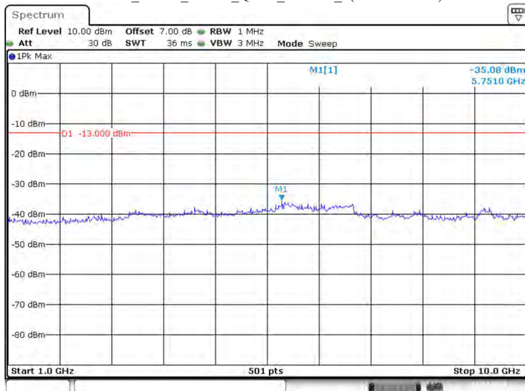
Band 5_5 MHz_Middle_QPSK_RB25#0_2(1GHz-10GHz)
