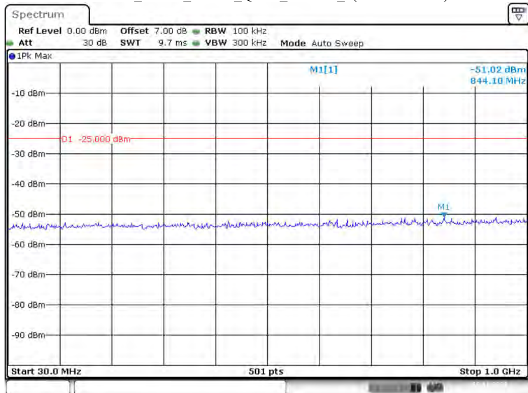
Band 38_5 MHz_Middle_QPSK_RB25#0_1(30MHz-1GHz)
