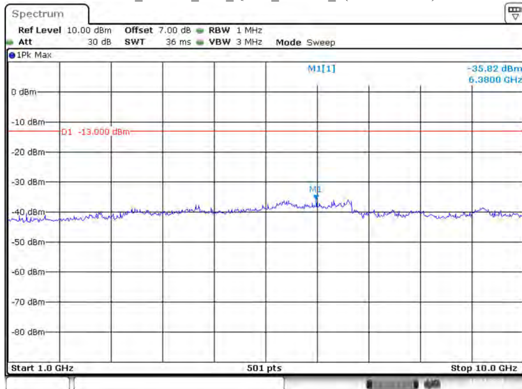
Band 5_10 MHz_Low_QPSK_RB50#0_2(1GHz-10GHz)
