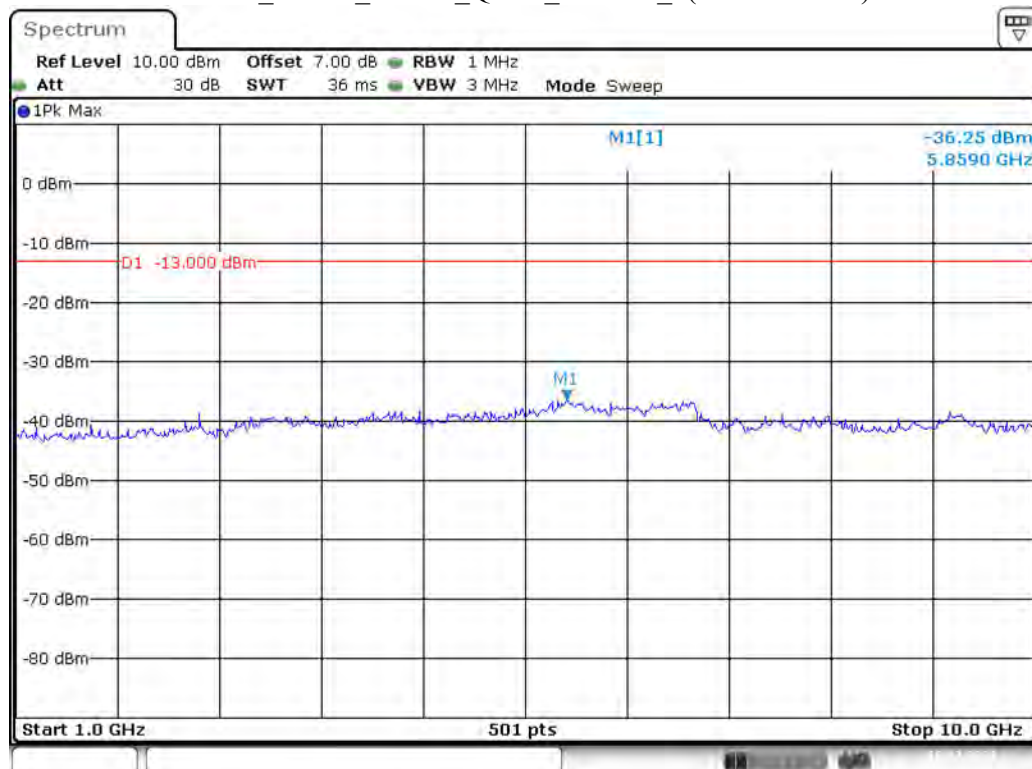
Band 5_3 MHz_Middle_QPSK_RB15#0_2(1GHz-10GHz)
