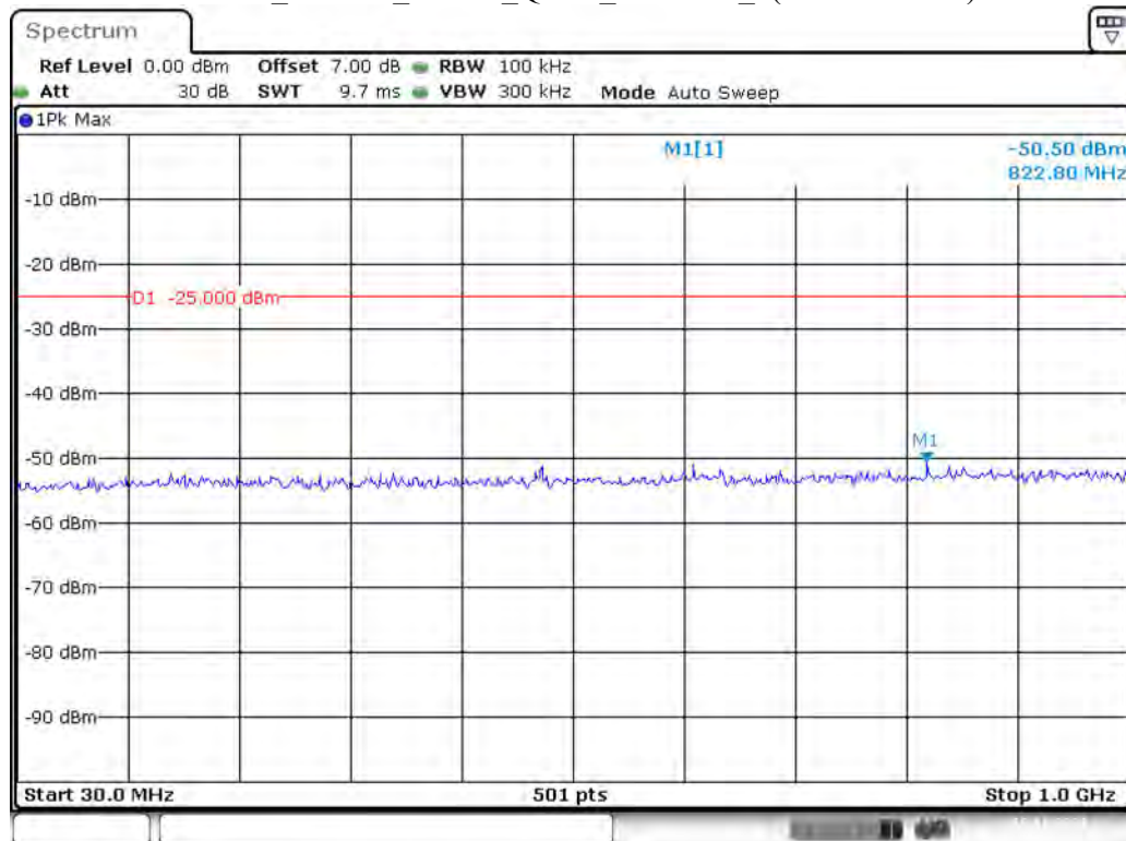
Band 41_20 MHz_Middle_QPSK_RB100#0_1(30MHz-1GHz)
