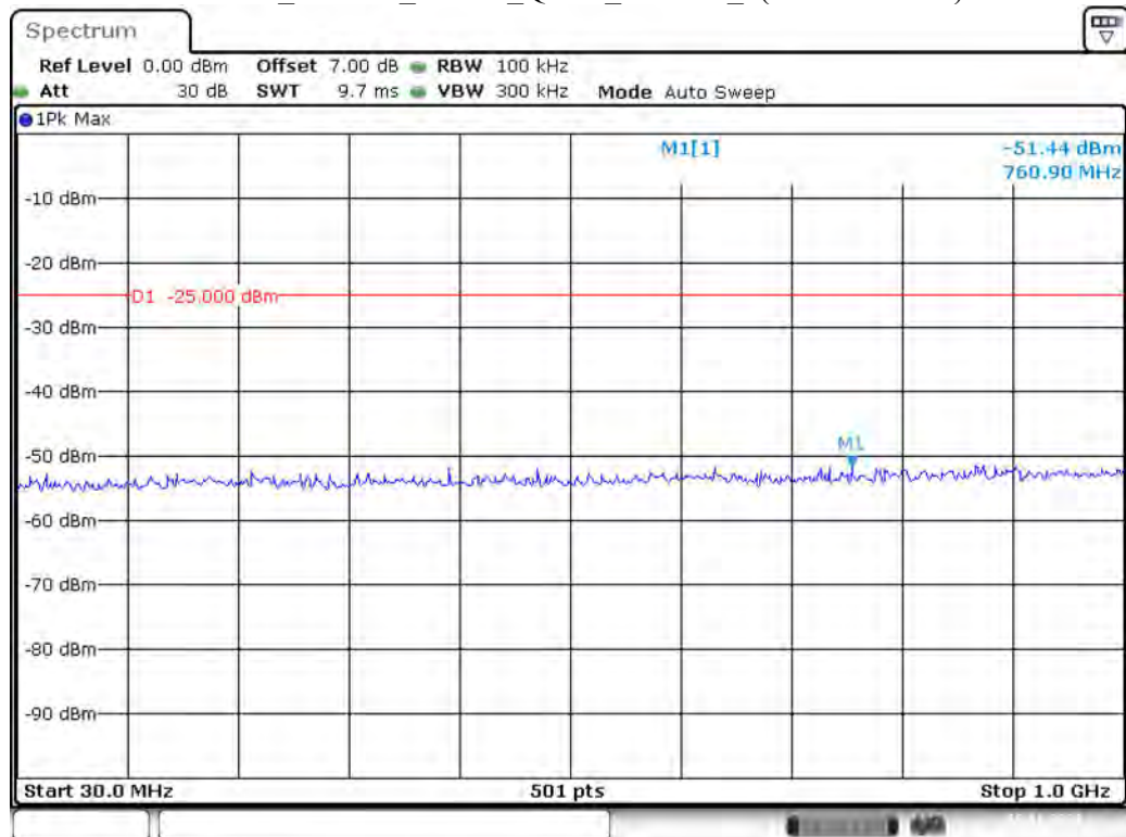
Band 38_15 MHz_Middle_QPSK_RB75#0_1(30MHz-1GHz)
