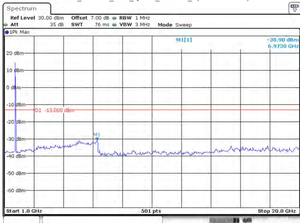
Band 4_10 MHz_Low_QPSK_RB50#0_2(1GHz-20GHz)
