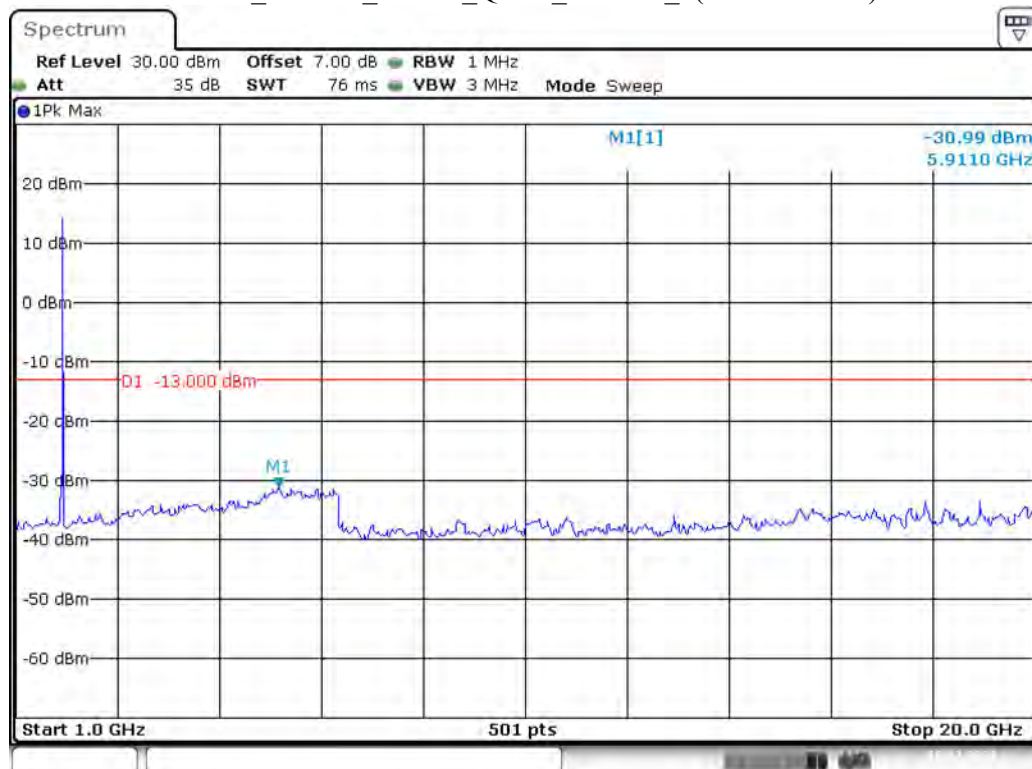
Band 2_10 MHz_Middle_QPSK_RB50#0_2(1GHz-20GHz)
