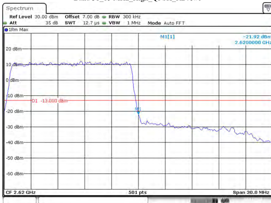
Band 38_15 MHz_High_QPSK_RB75#0
