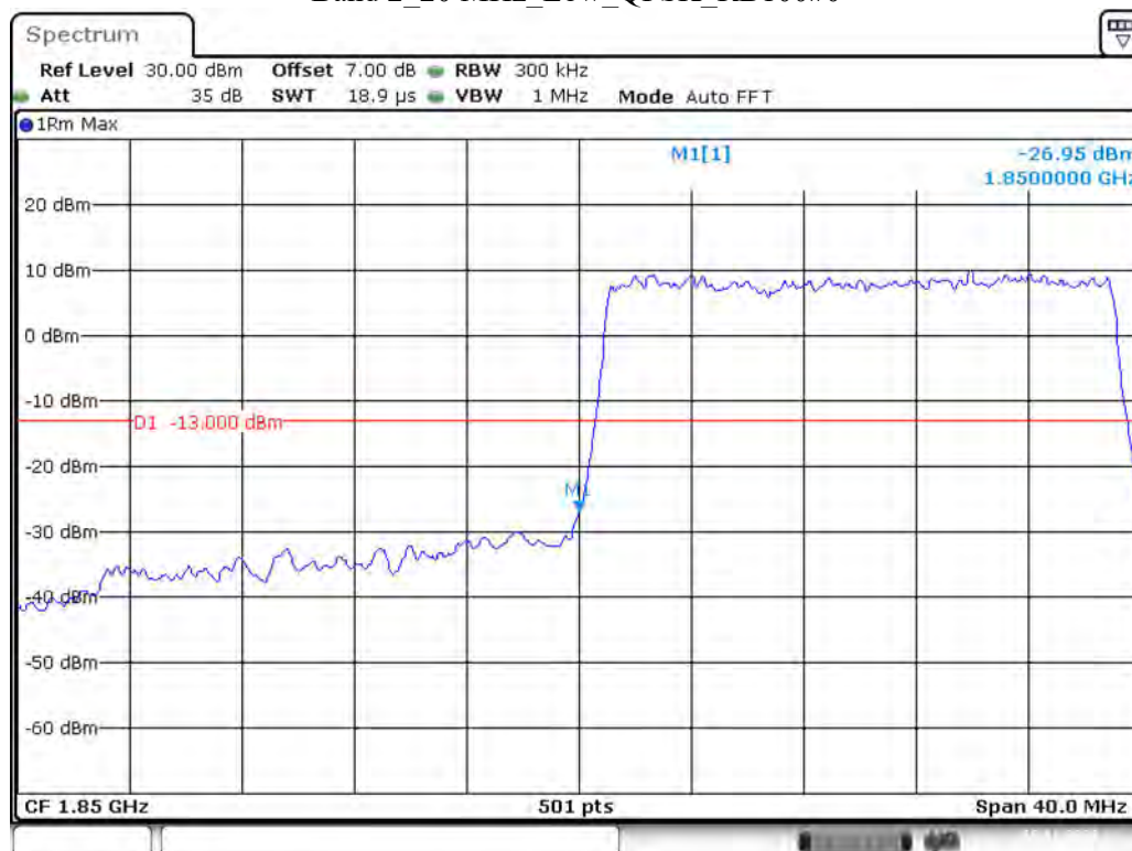
Band 2_20 MHz_Low_QPSK_RB100#0
