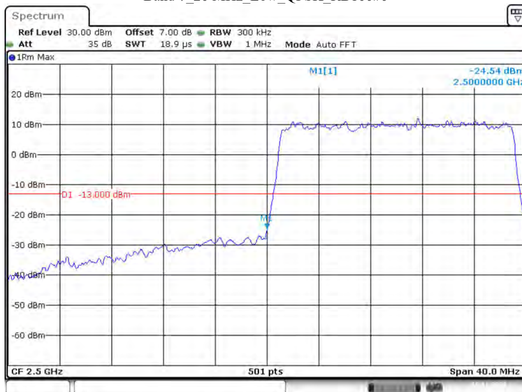
Band 7_20 MHz_Low_QPSK_RB100#0
