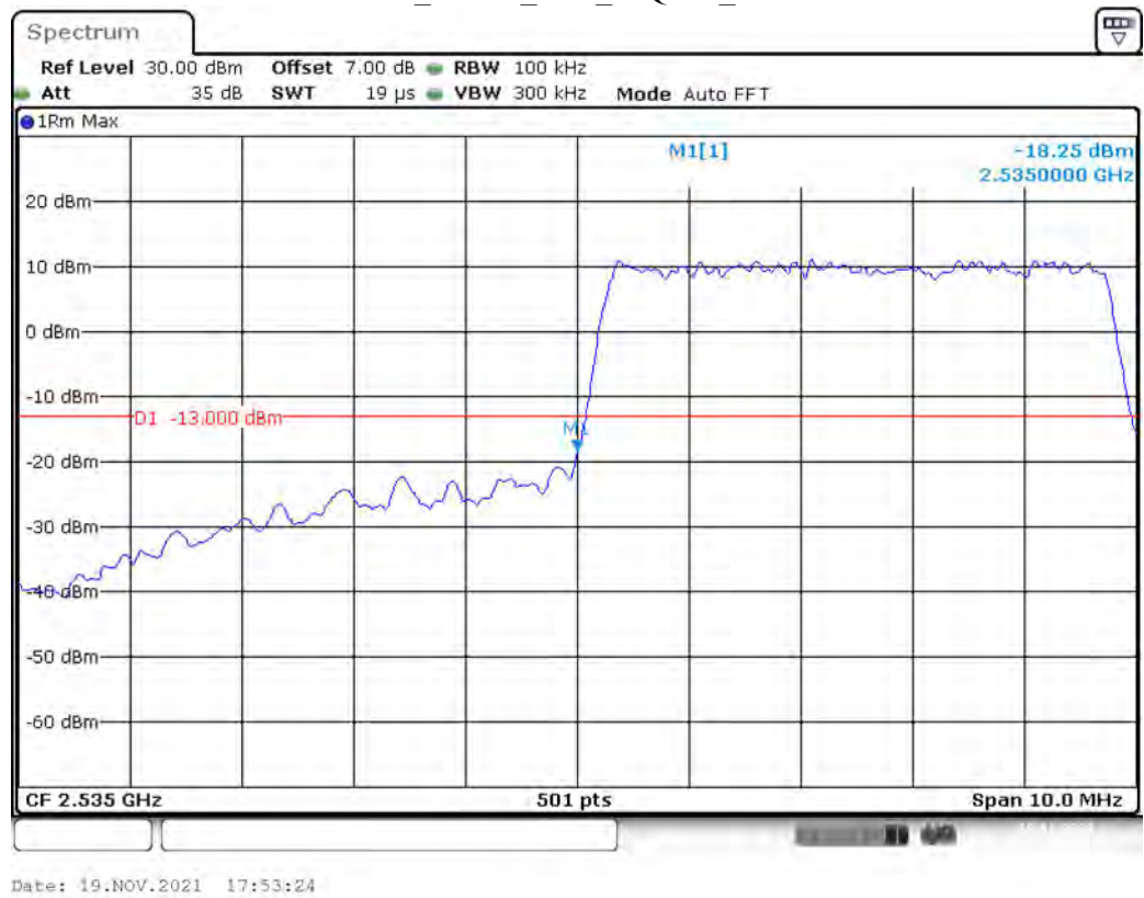
Band 41_5 MHz_Low_16QAM_RB25#0
