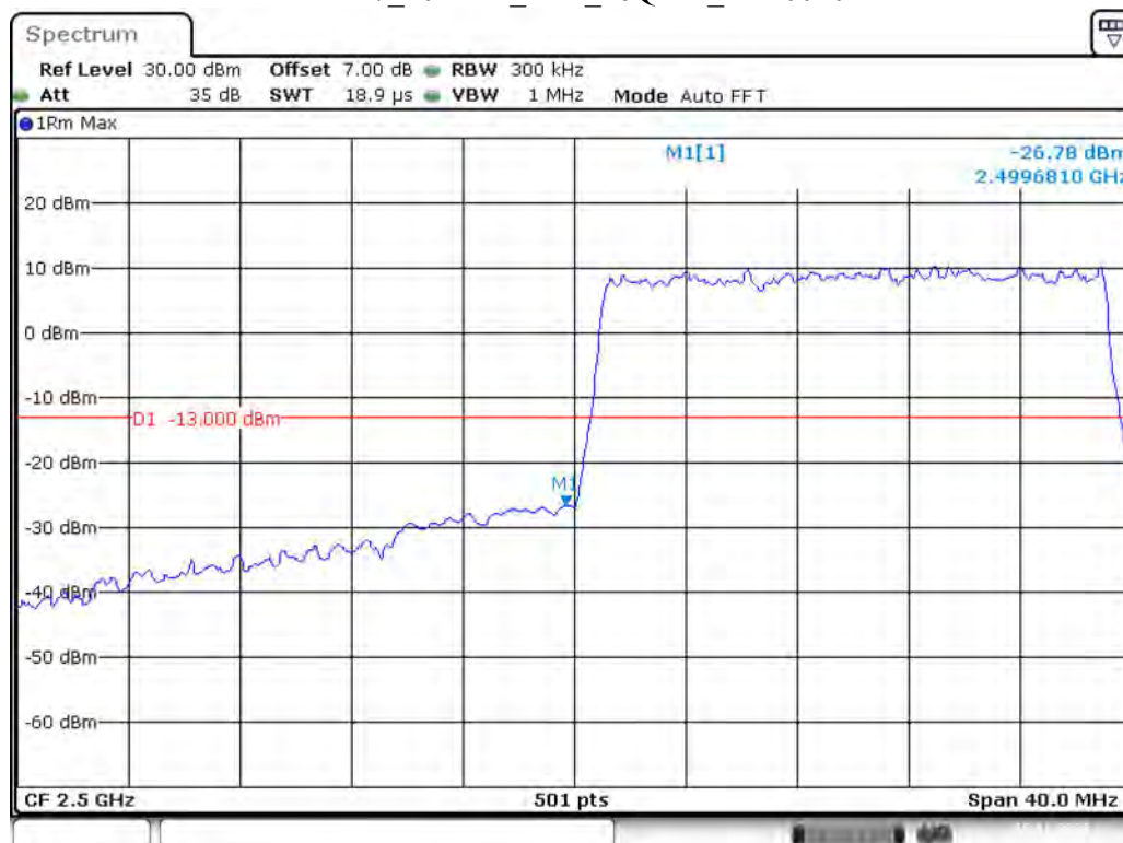
Band 7_20 MHz_Low_16QAM_RB100#0
