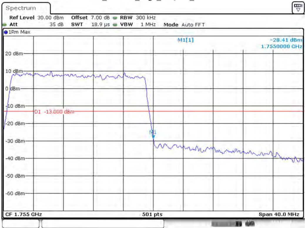
Band 4_20 MHz_High_16QAM_RB100#0
