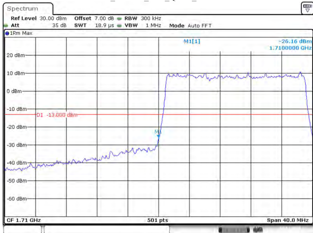
Band 4_20 MHz_Low_QPSK_RB100#0
