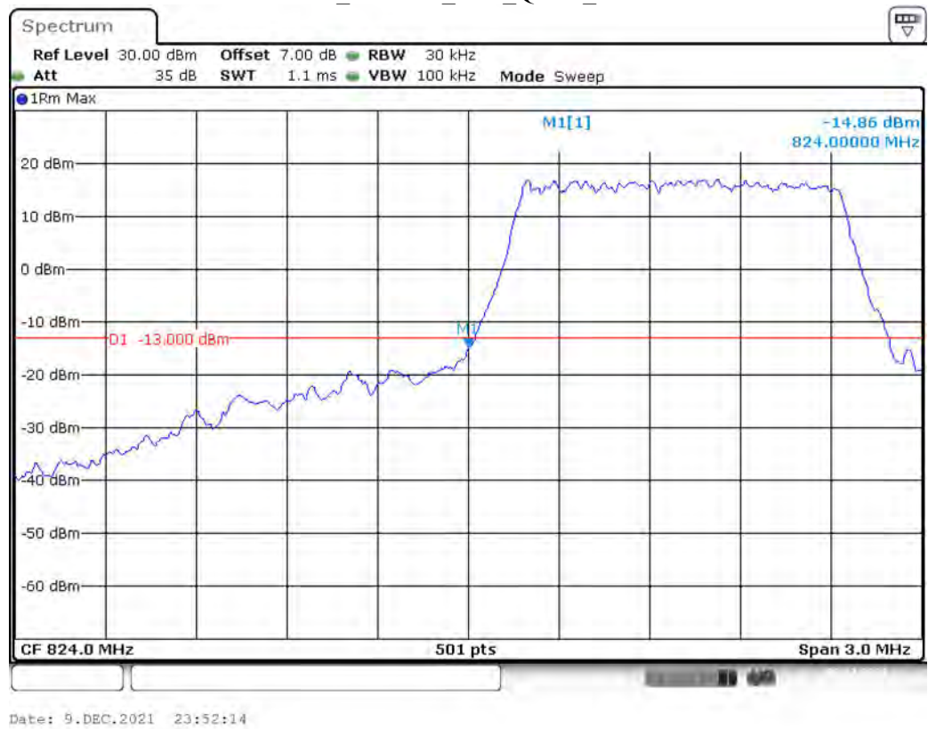
Band 5_1.4 MHz_Low_QPSK_RB6#0
