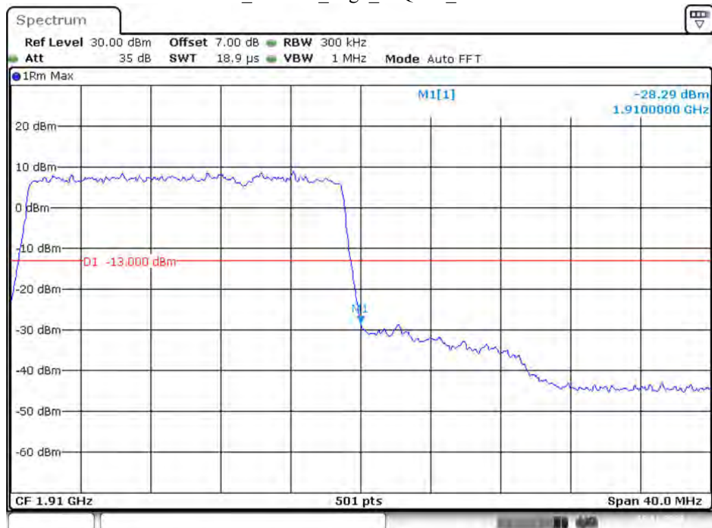
Band 2_20 MHz_High_16QAM_RB100#0
