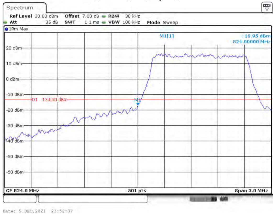
Band 5_1.4 MHz_Low_16QAM_RB6#0
