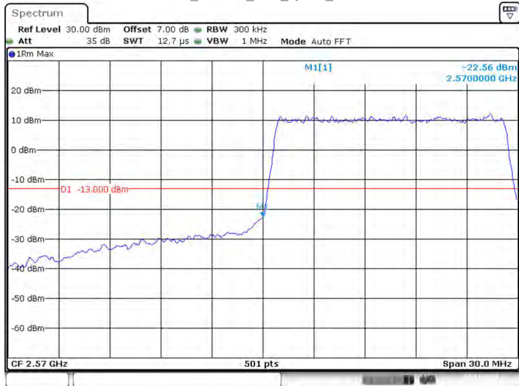
Band 38_15 MHz_Low_QPSK_RB75#0
