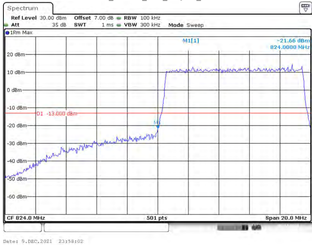
Band 5_10 MHz_Low_16QAM_RB50#0
