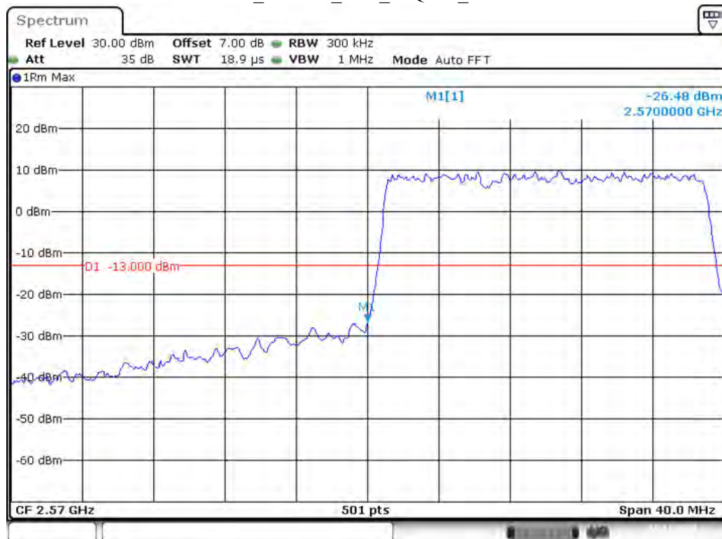
Band 38_20 MHz_Low_16QAM_RB100#0
