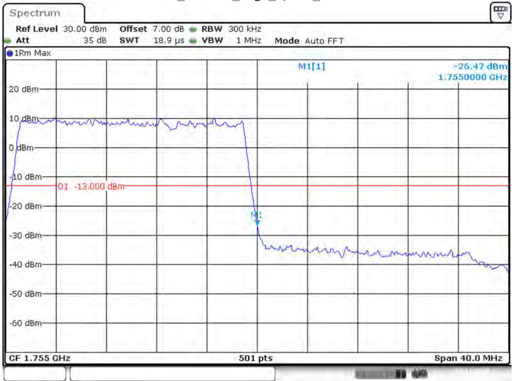
Band 4_20 MHz_High_QPSK_RB100#0
