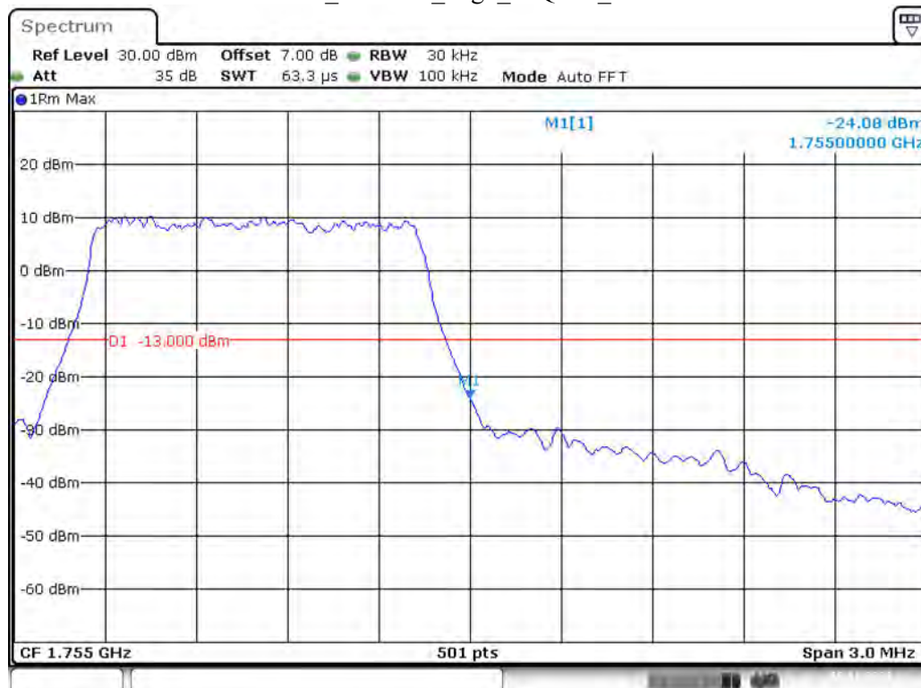
Band 4_1.4 MHz_High_16QAM_RB6#0
