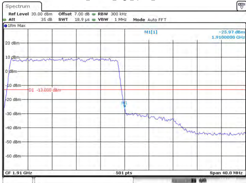
Band 2_20 MHz_High_QPSK_RB100#0
