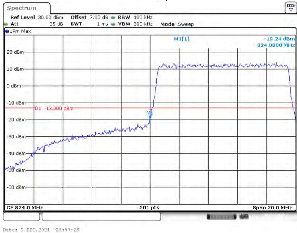
Band 5_10 MHz_Low_QPSK_RB50#0
