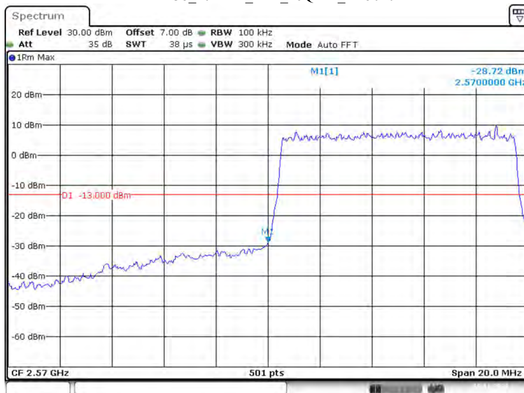
Band 38_10 MHz_Low_16QAM_RB50#0
