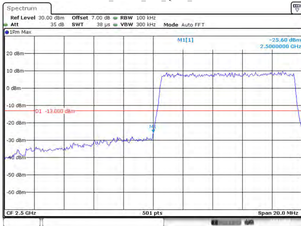
Band 7_10 MHz_Low_QPSK_RB50#0
