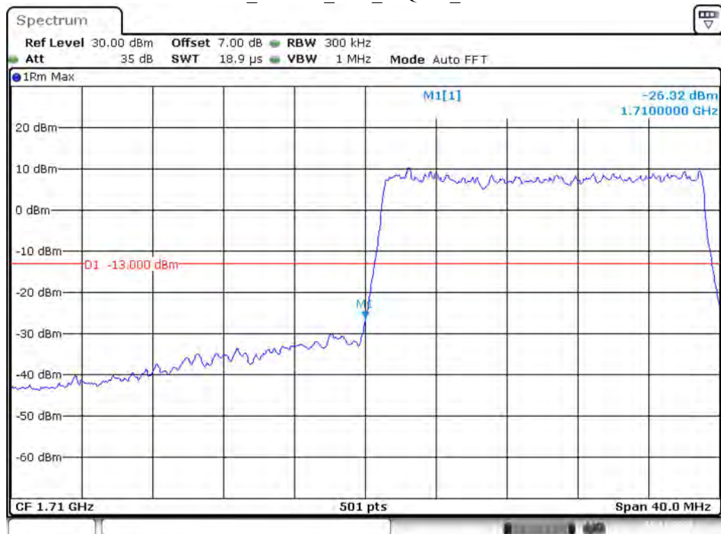
Band 4_20 MHz_Low_16QAM_RB100#0
