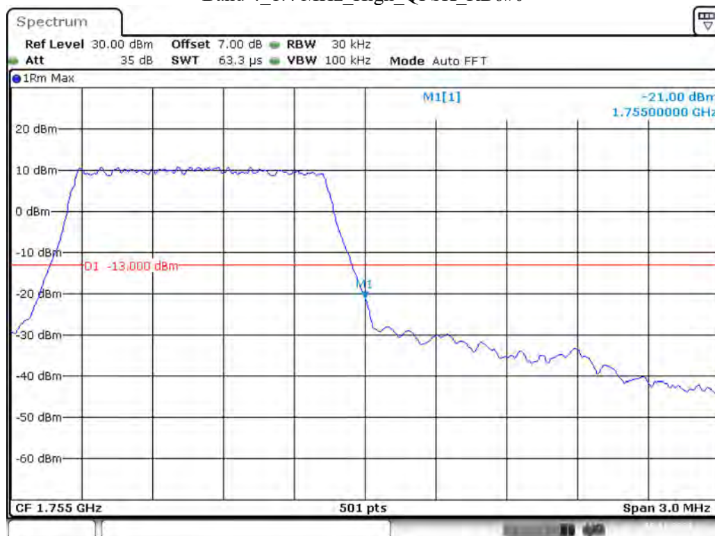
Band 4_1.4 MHz_High_QPSK_RB6#0
