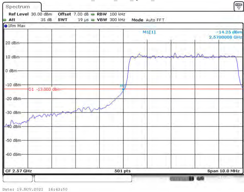
Band 38_5 MHz_Low_QPSK_RB25#0
