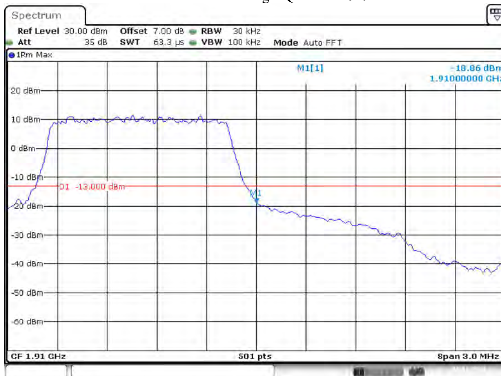
Band 2_1.4 MHz_High_QPSK_RB6#0
