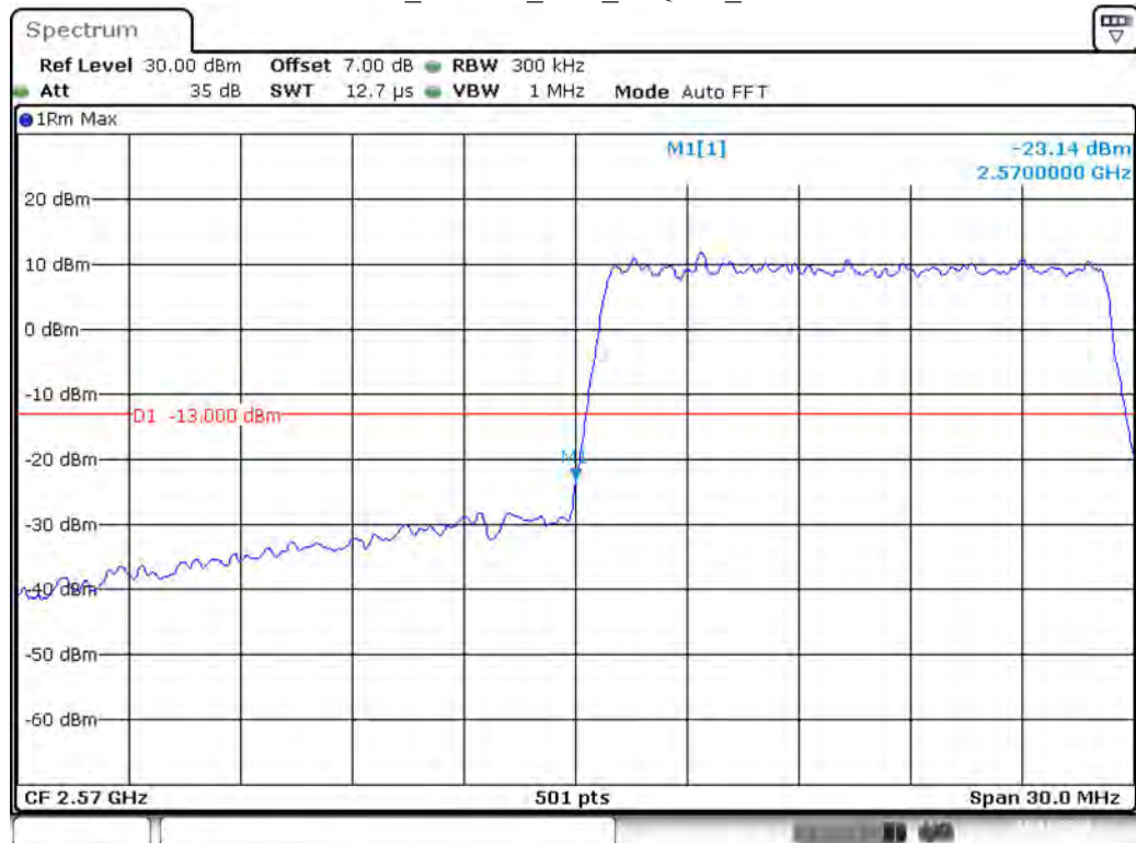
Band 38_15 MHz_Low_16QAM_RB75#0
