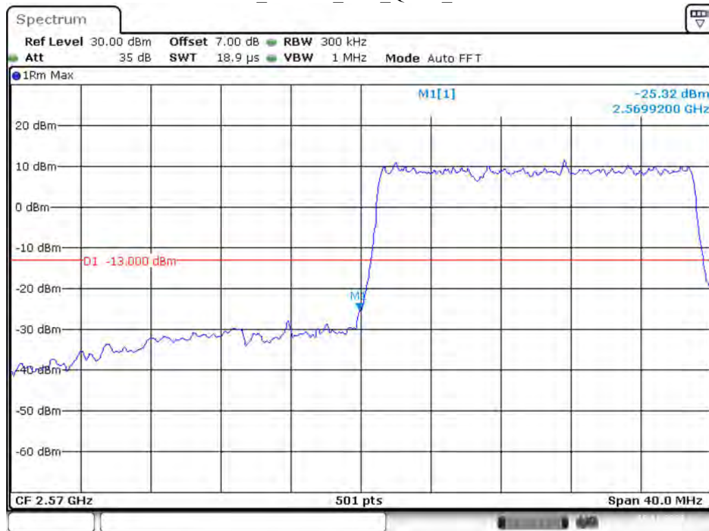
Band 38_20 MHz_Low_QPSK_RB100#0
