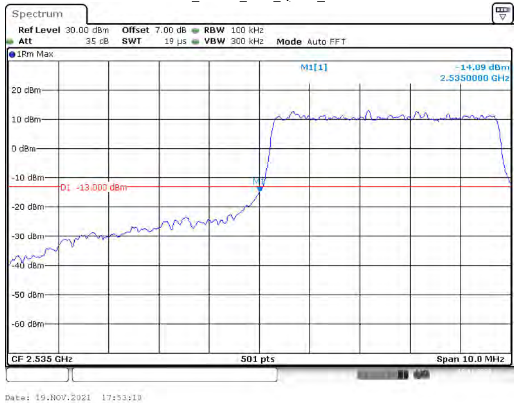
Band 41_5 MHz_Low_QPSK_RB25#0
