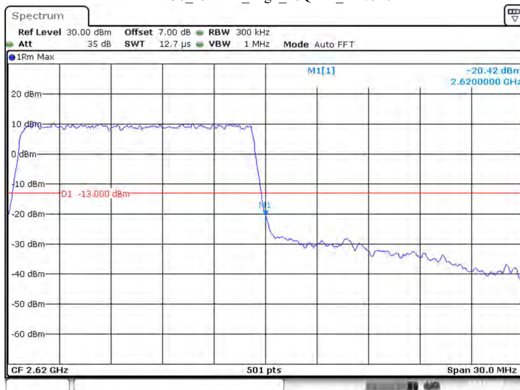
Band 38_15 MHz_High_16QAM_RB75#0
