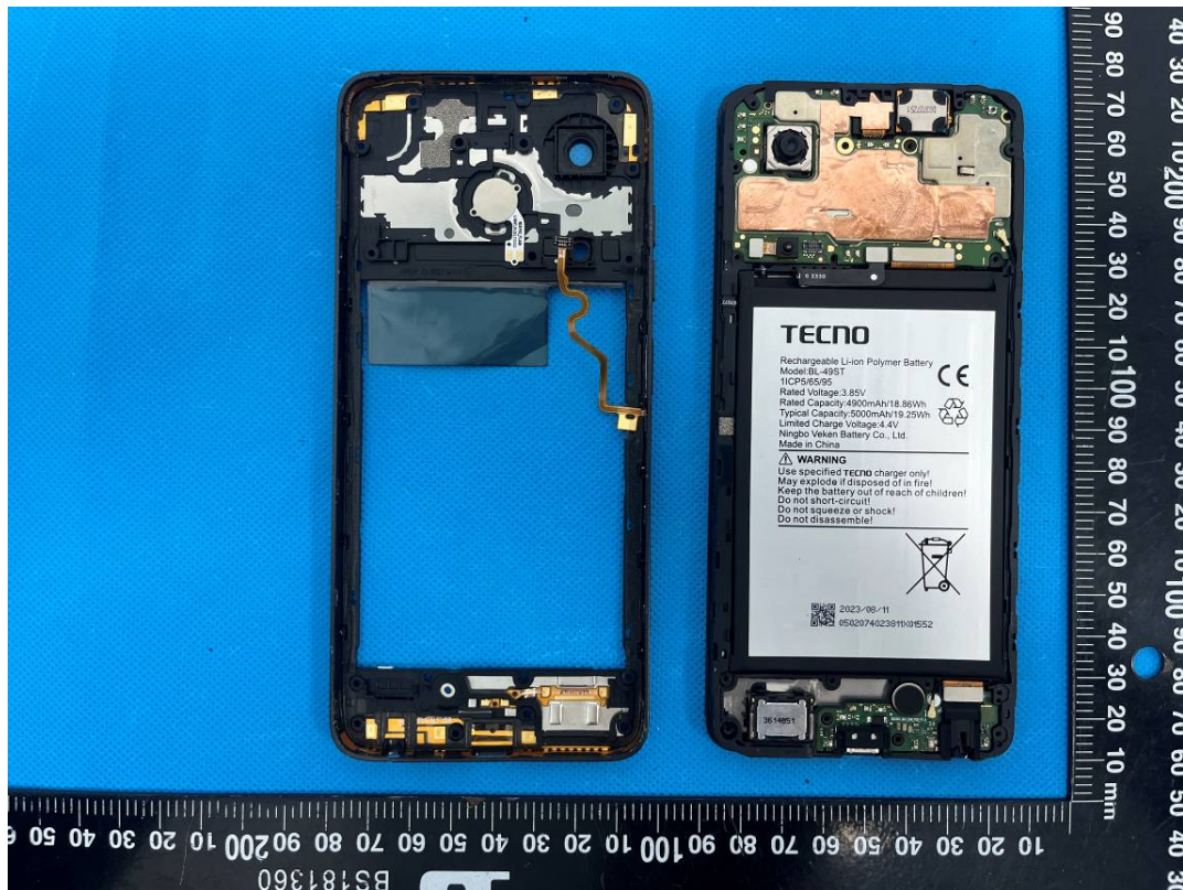
WWAN Main ANT (GSM850/WCDMA B5/LTE B5/12/17)
