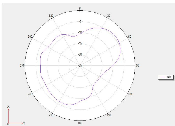
Theta 90 2D
