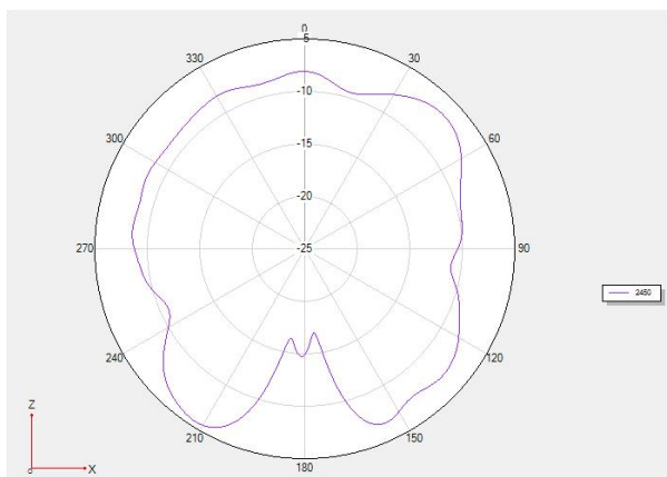
Theta 90 2D
