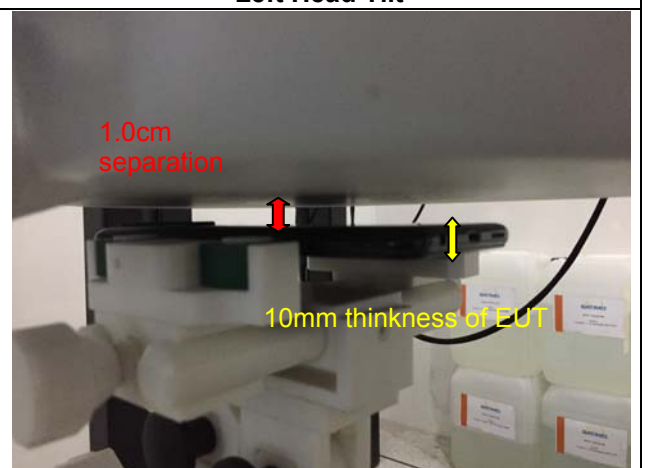
Body-Worn(LCD Down)
