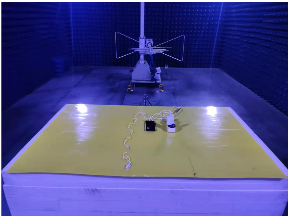
Photo of Radiated Emission Measurement (30MHz-1GHz)
