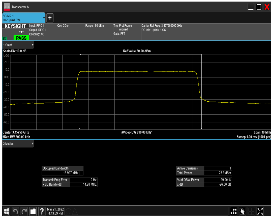
n77(3450-3550) SCS=15kHz DFT_QAM64 BW=15MHz Channel=630500 RB=75@0
