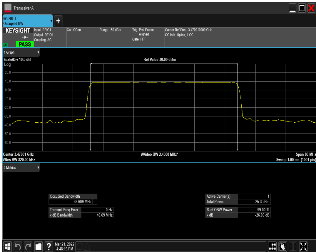
n77(3450-3550) SCS=15kHz DFT_QPSK BW=40MHz Channel=631334 RB=216@0
