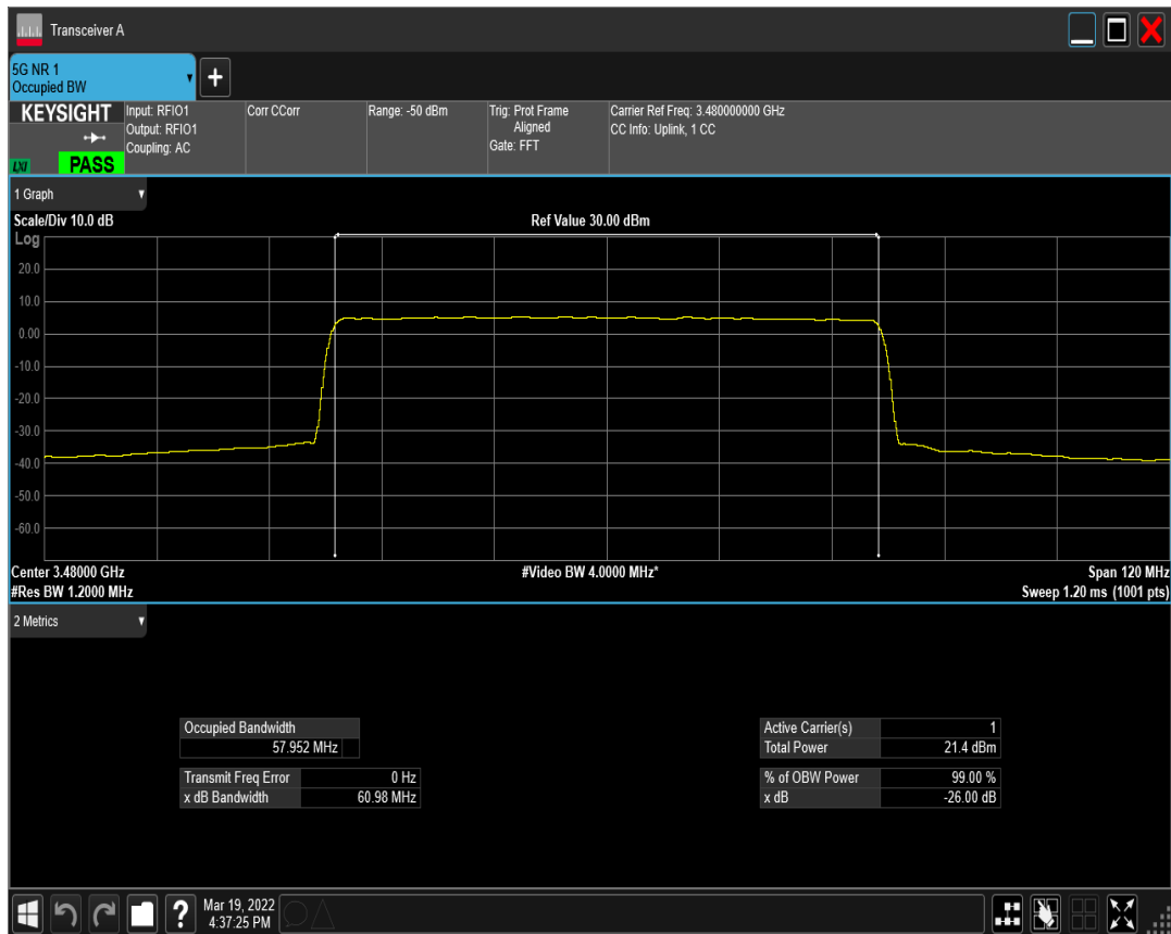
n77(3450-3550) SCS=30kHz CP_QPSK BW=60MHz Channel=632000 RB=162@0
