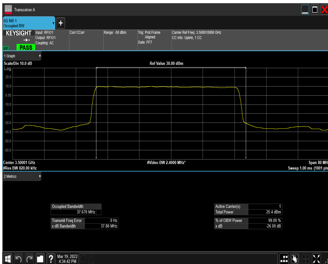
n77(3450-3550) SCS=30kHz DFT_QPSK BW=40MHz Channel=633334 RB=100@0
