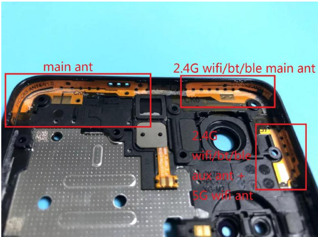
main + 2.4G wifi+bt+ble+5G wifi Antenna
