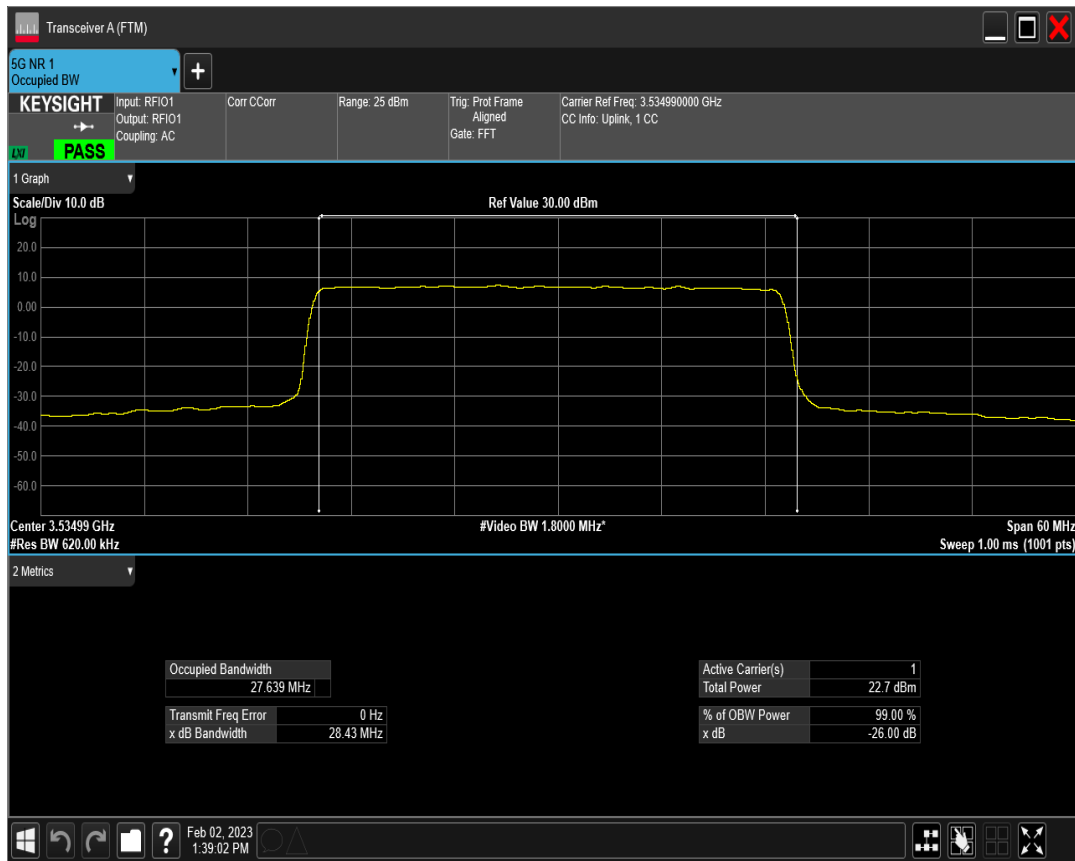
n77(3450-3550) SCS=30kHz CP_QPSK BW=30MHz Channel=635666 RB=78@0
