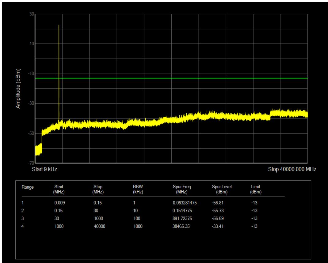
n77(3450-3550) SCS=30kHz DFT_QPSK BW=10MHz Channel=633334 RB=1@23
