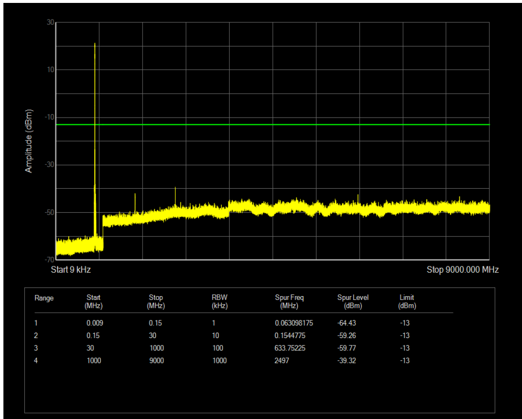
n5 SCS=30kHz DFT_QPSK BW=10MHz Channel=167300 RB=1@23
