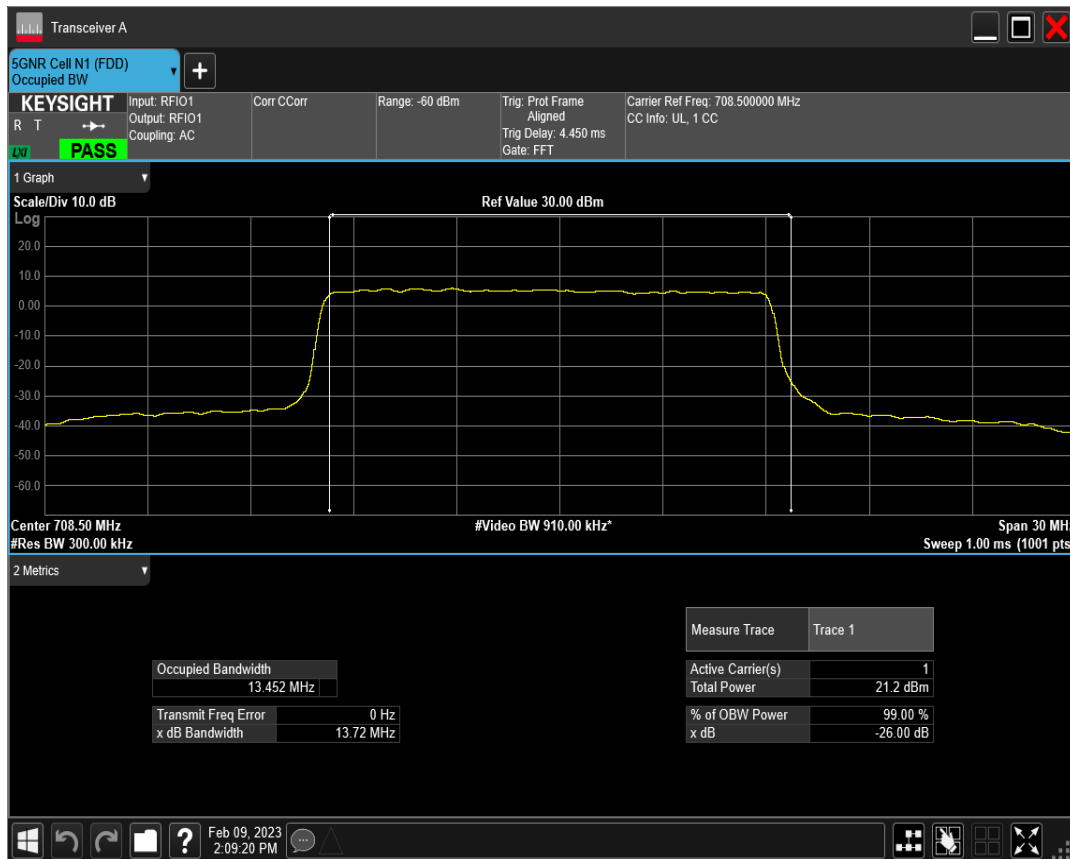
n12 SCS=30kHz DFT_QAM256 BW=15MHz Channel=141700 RB=36@0
