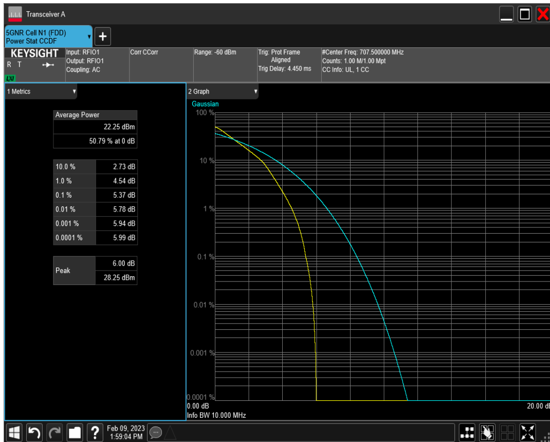
n12 SCS=30kHz DFT_QAM16 BW=10MHz Channel=141500 RB=24@0
