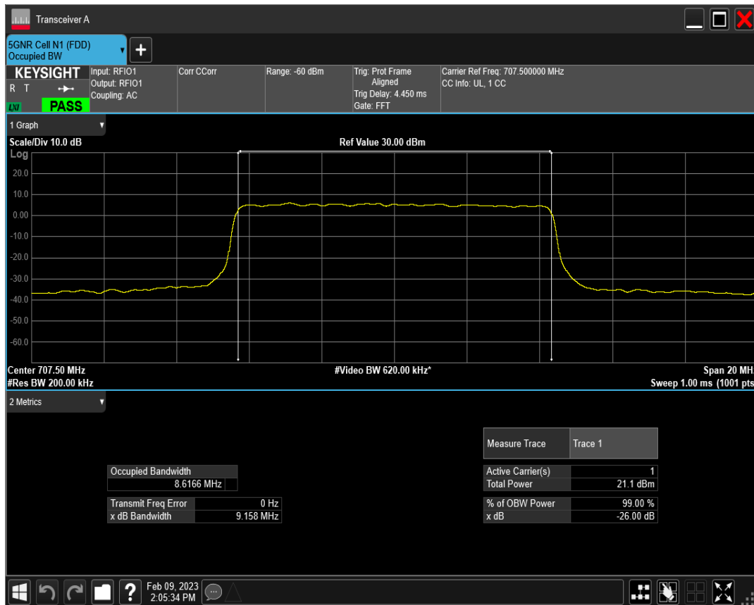
n12 SCS=30kHz DFT_QAM256 BW=10MHz Channel=141500 RB=24@0
