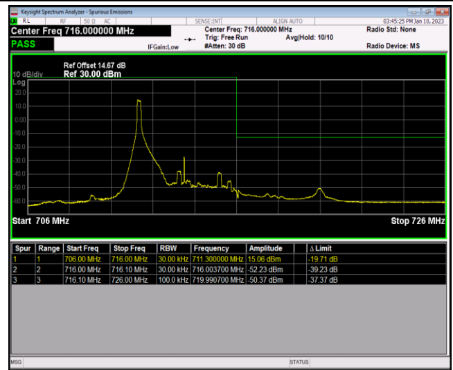
Band17-5MHz-QPSK-23825-25RB#0
