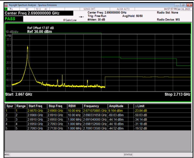
Band41-20MHz-QPSK-41490-100RB#0
