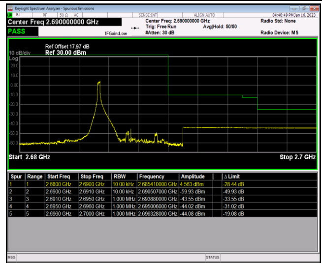
Band41-5MHz-64QAM-41565-25RB#0
