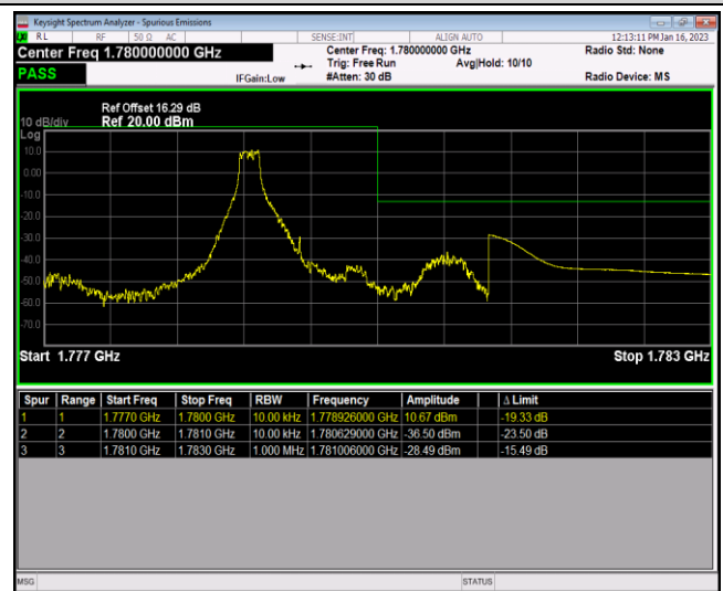
Band66-1.4MHz-16QAM-132665-6RB#0
