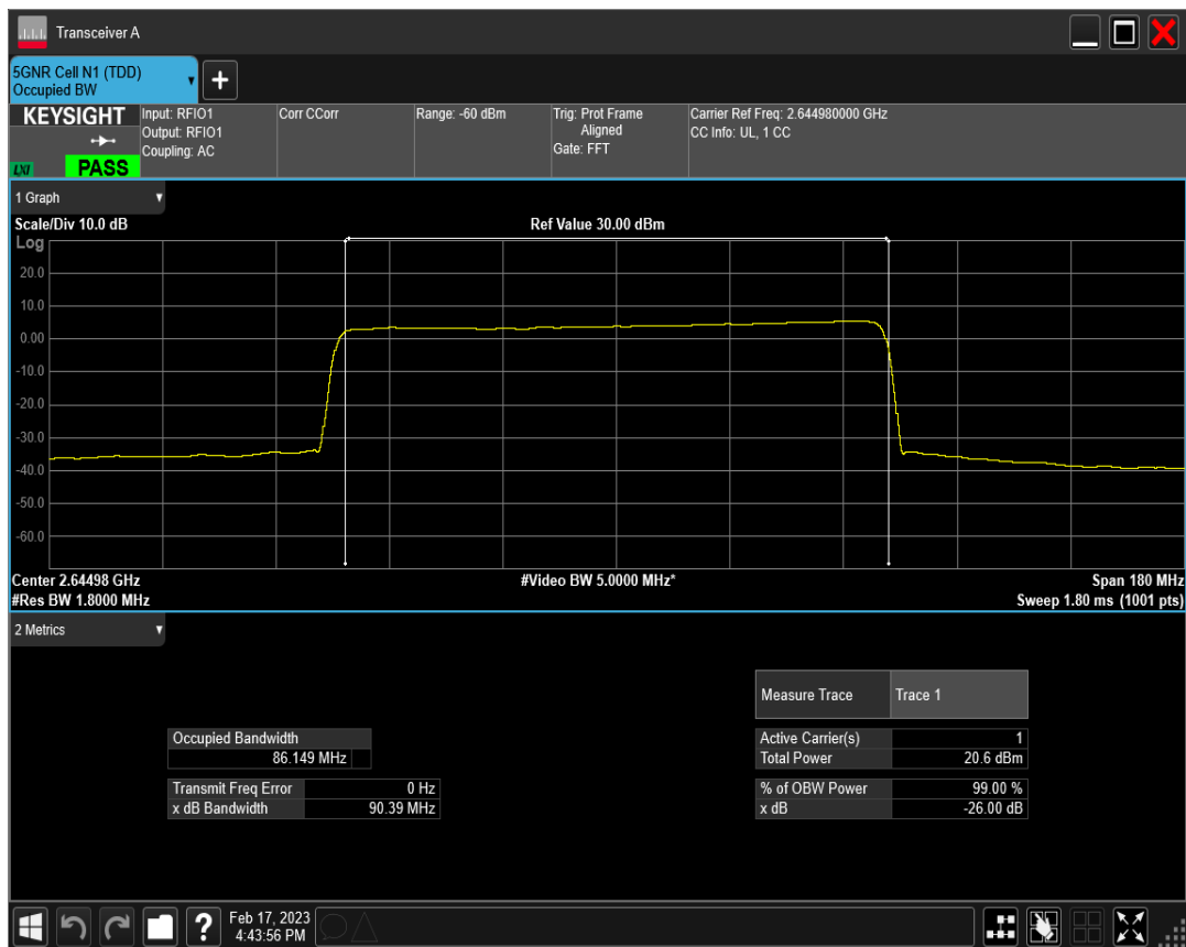
n41 SCS=30kHz CP_QPSK BW=90MHz Channel=528996 RB=245@0
