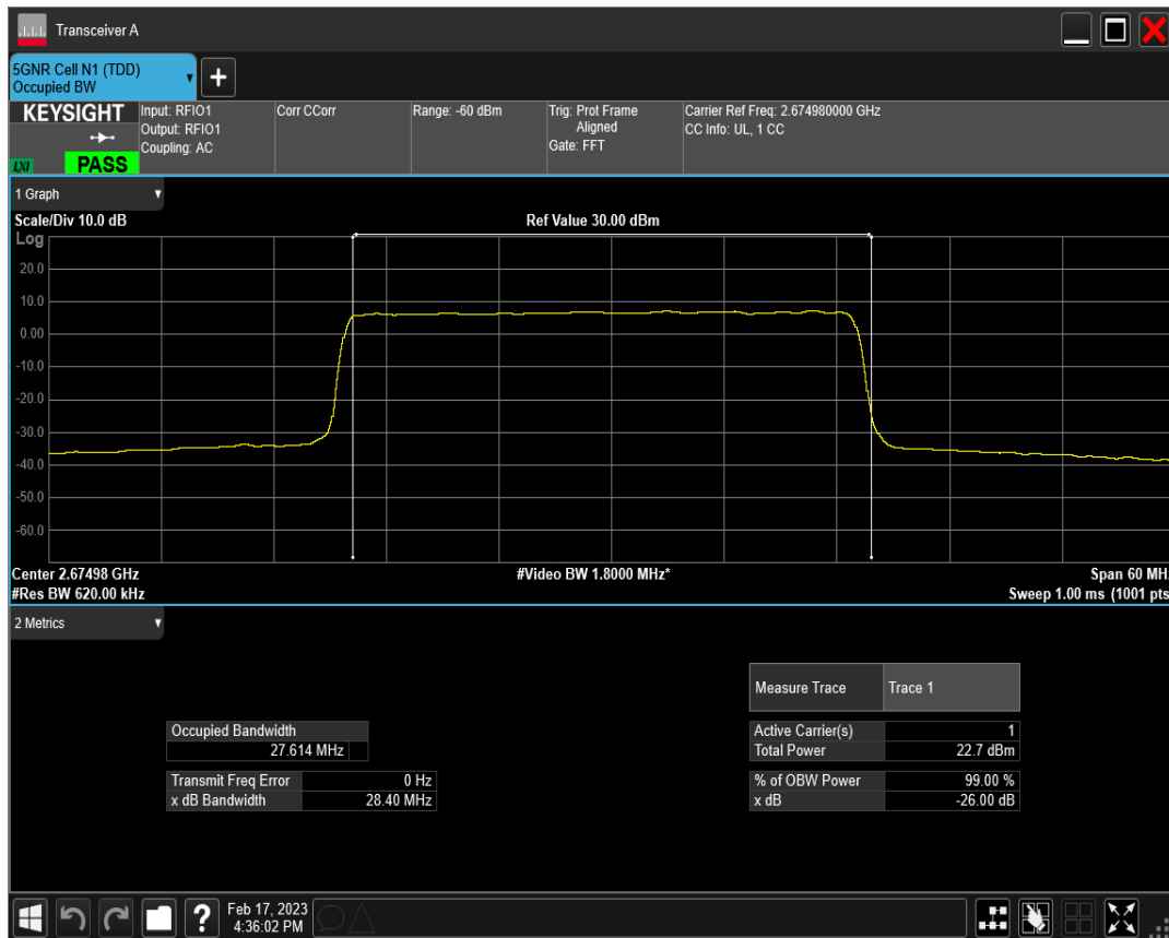
n41 SCS=30kHz DFT_QAM256 BW=30MHz Channel=534996 RB=75@0
