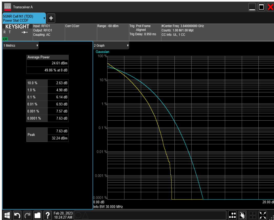
n77(3700-3980) SCS=15kHz DFT_QAM16 BW=30MHz Channel=656000 RB=160@0
