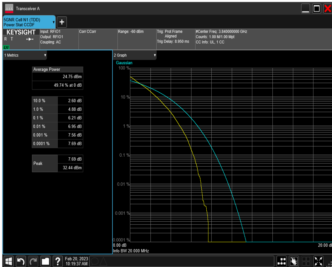
n77(3700-3980) SCS=15kHz DFT_QAM16 BW=15MHz Channel=656000 RB=75@0
