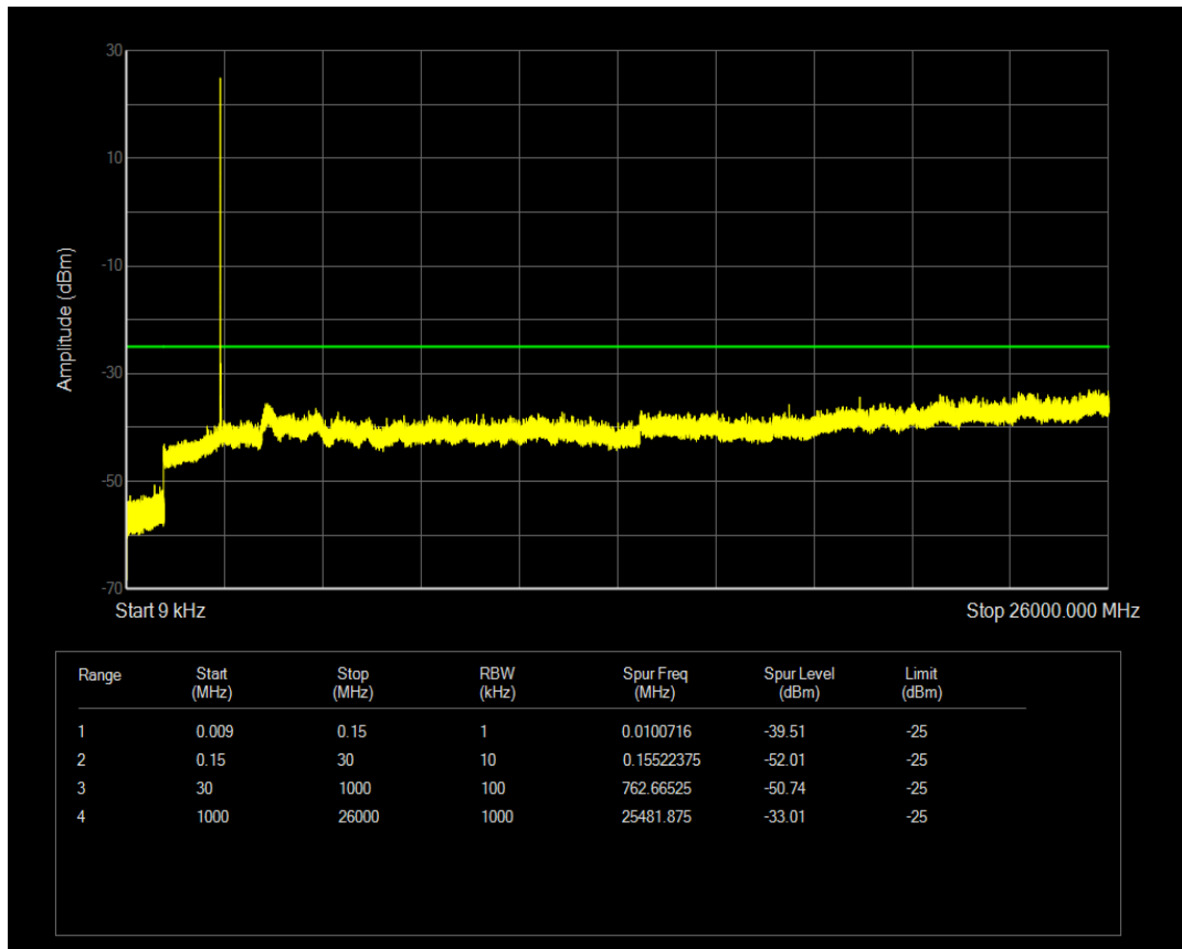
n7 SCS=30kHz DFT_QPSK BW=10MHz Channel=501000 RB=1@23
