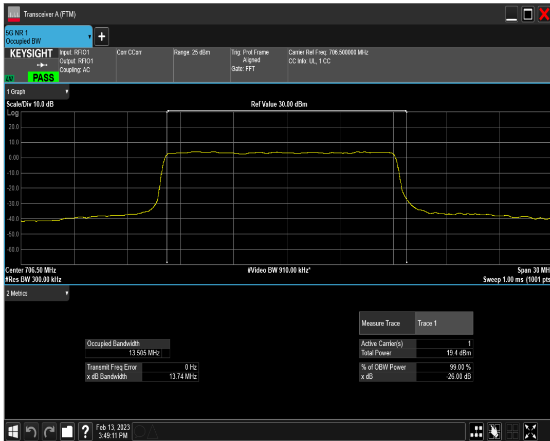
n12 SCS=30kHz CP_QPSK BW=15MHz Channel=141300 RB=38@0
