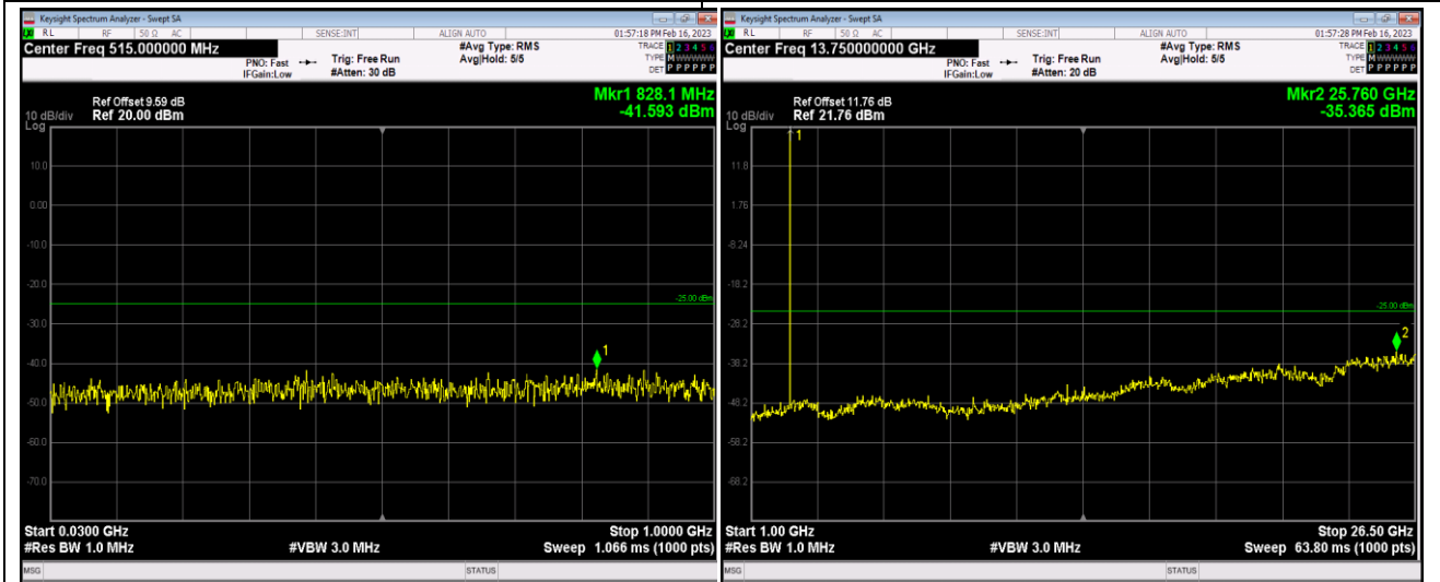
Band7-5MHz-16QAM-21100-1RB#0-Range1:30~1000MHz
