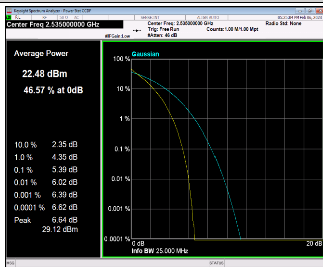
Band7-20MHz-64QAM-21100-100RB#0
