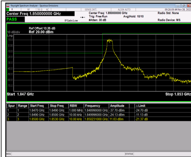
Band2-1.4MHz-64QAM-18607-6RB#0
