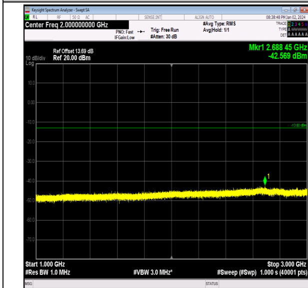
Band26_5MHz_16QAM_26715_1RB#0_1000~3000_1000 ~3000
