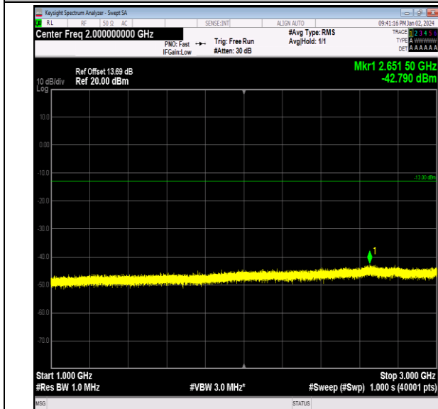
Band26_3MHz_QPSK_26915_1RB#0_1000~3000_1000~3000
