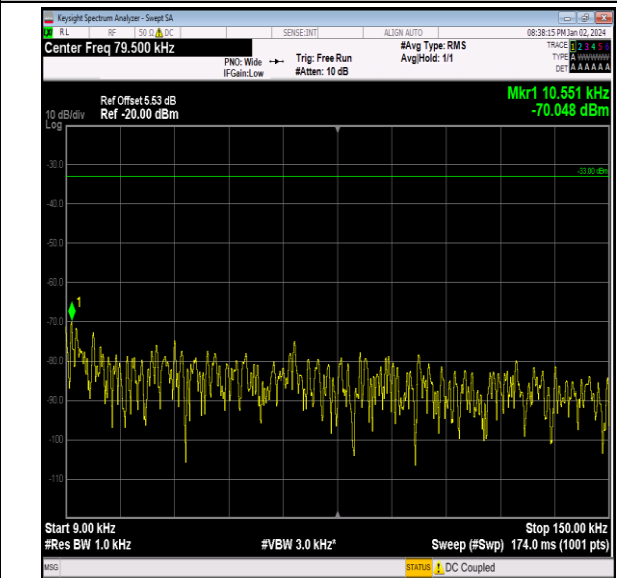
Band26_5MHz_16QAM_26715_1RB#0_0.009~0.15_0.009~0.15
