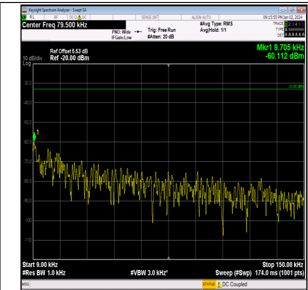
Band26_1.4MHz_16QAM_27033_1RB#0_0.009~0.15_0.0 09~0.15
