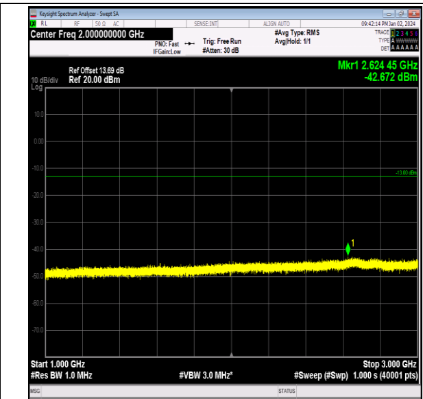
Band26_3MHz_16QAM_26915_1RB#0_1000~3000_1000 ~3000
