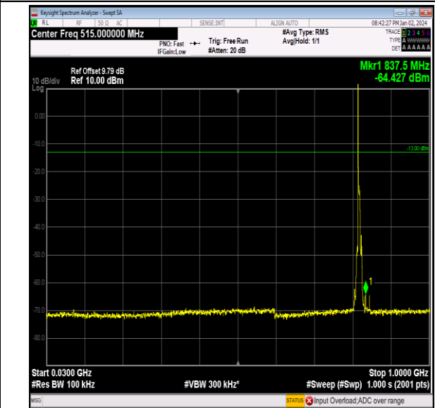
Band26_5MHz_16QAM_26765_1RB#0_30~1000_30~100 0
