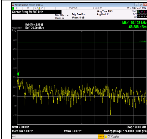
Band26_10MHz_QPSK_26740_1RB#0_0.009~0.15_0.009 ~0.15
