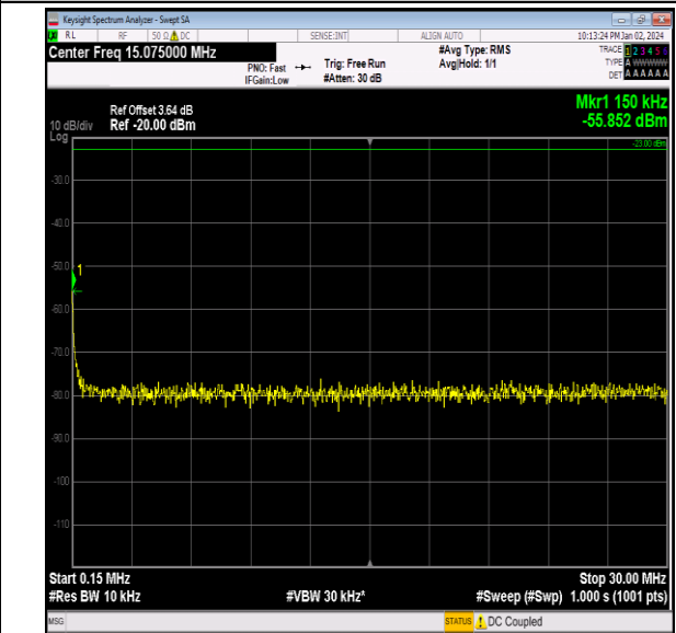
Band26_5MHz_QPSK_27015_1RB#0_0.15~30_0.15~30
