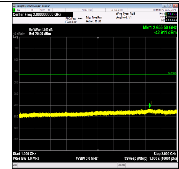
Band26_5MHz_QPSK_26765_1RB#0_1000~3000_1000~3000
