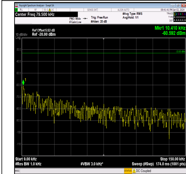
Band26_3MHz_16QAM_26915_1RB#0_0.009~0.15_0.009 ~0.15
