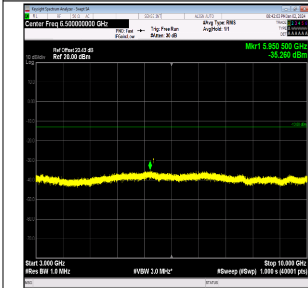
Band26_5MHz_QPSK_26765_1RB#0_3000~10000_3000~10000
