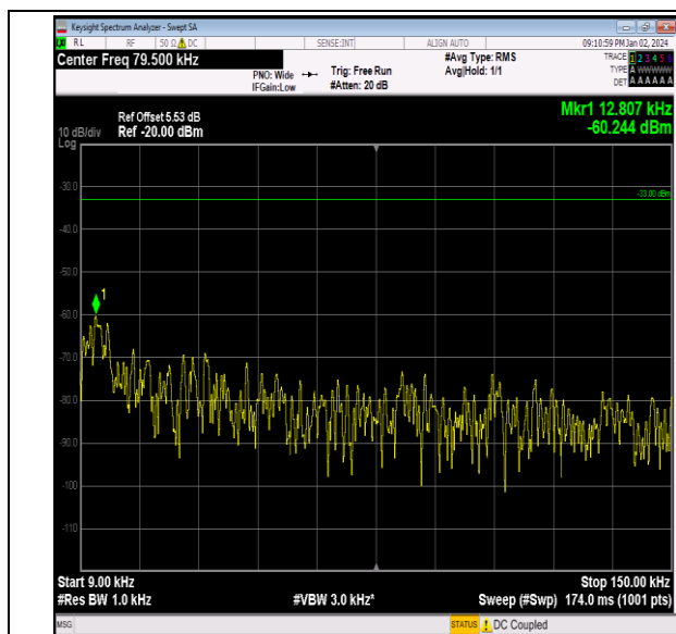
Band26_1.4MHz_QPSK_26797_1RB#0_0.009~0.15_0.00 9~0.15
