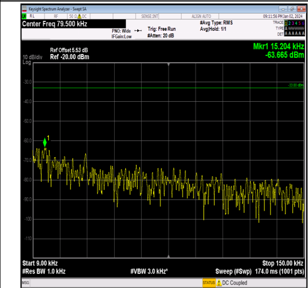
Band26_1.4MHz_16QAM_26797_1RB#0_0.009~0.15_0.0 09~0.15
