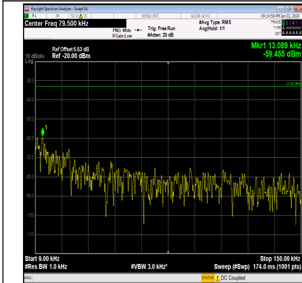
Band26_1.4MHz_QPSK_27033_1RB#0_0.009~0.15_0.00 9~0.15
