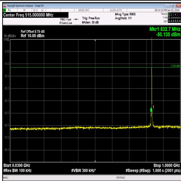
Band26_1.4MHz_16QAM_26915_1RB#0_30~1000_30~1 000
