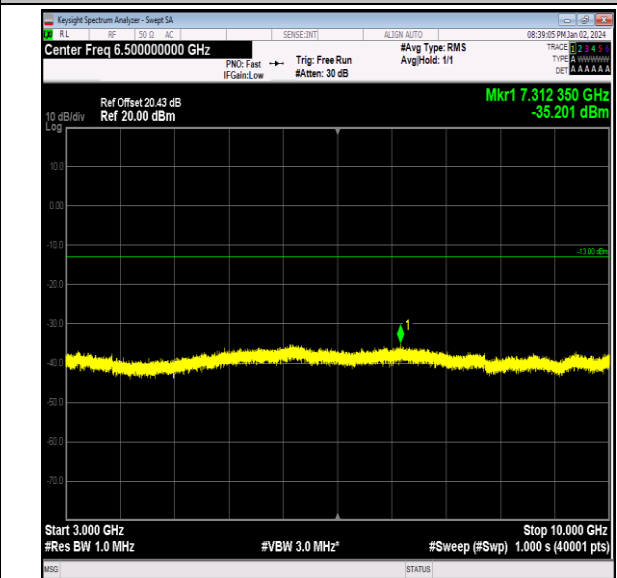
Band26_5MHz_16QAM_26715_1RB#0_3000~10000_3000 0~10000
