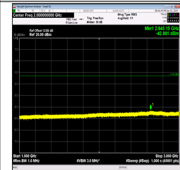
Band26_5MHz_16QAM_26740_1RB#0_1000~3000_1000 ~3000
