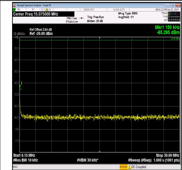
Band26_5MHz_QPSK_26765_1RB#0_0.15~30_0.15~30
