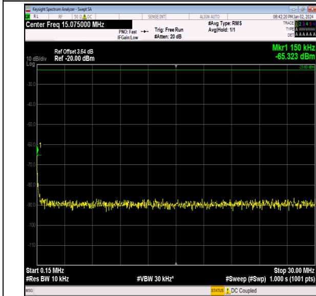
Band26_5MHz_16QAM_26765_1RB#0_0.15~30_0.15~30
