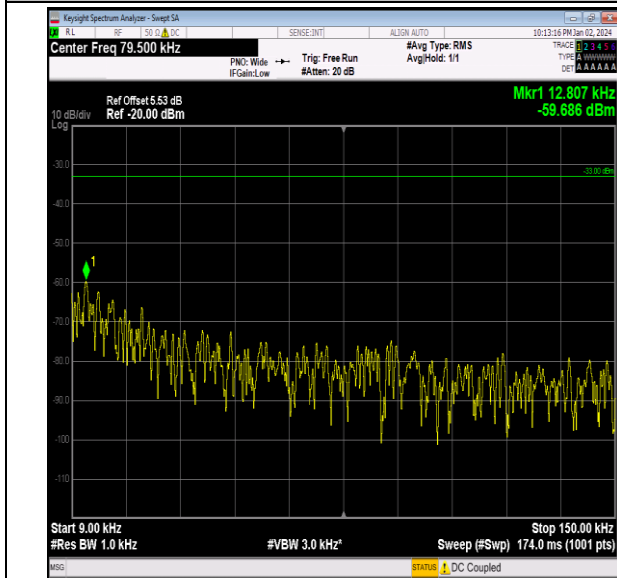
Band26_5MHz_QPSK_27015_1RB#0_0.009~0.15_0.009~0.15
