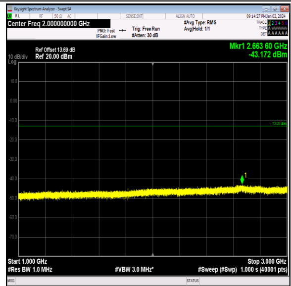
Band26_1.4MHz_16QAM_26915_1RB#0_1000~3000_100 0~3000
