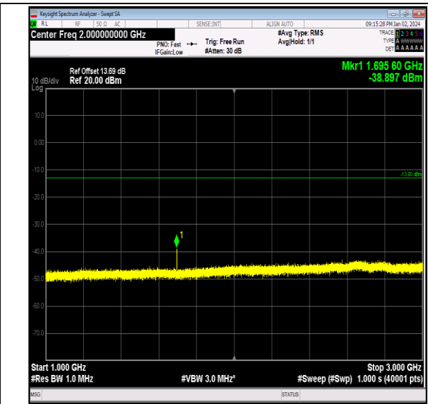
Band26_1.4MHz_QPSK_27033_1RB#0_1000~3000_1000 ~3000
