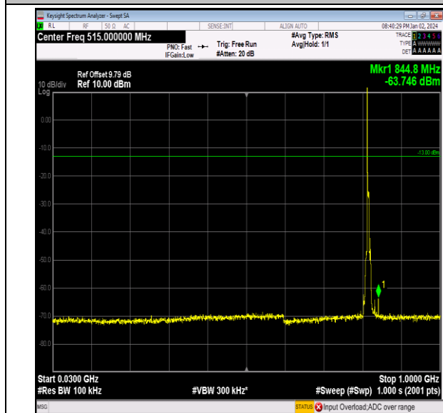
Band26_5MHz_16QAM_26740_1RB#0_30~1000_30~100 0
