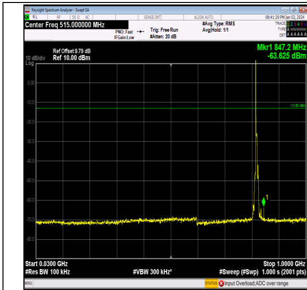
Band26_5MHz_QPSK_26765_1RB#0_30~1000_30~1000
