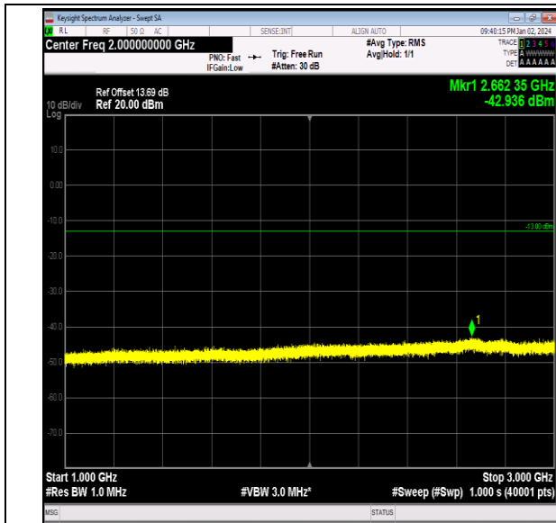
Band26_3MHz_16QAM_26805_1RB#0_1000~3000_1000 ~3000
