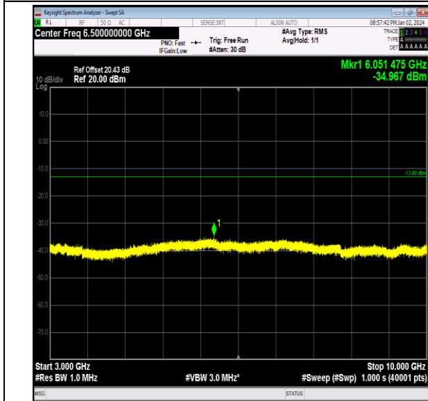
Band26_10MHz_QPSK_26740_1RB#0_3000~10000_300 0~10000
