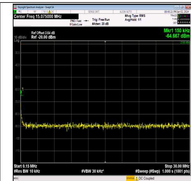
Band26_5MHz_16QAM_26740_1RB#0_0.15~30_0.15~30
