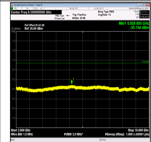
Band26_3MHz_16QAM_27025_1RB#0_3000~10000_3000 0~10000
