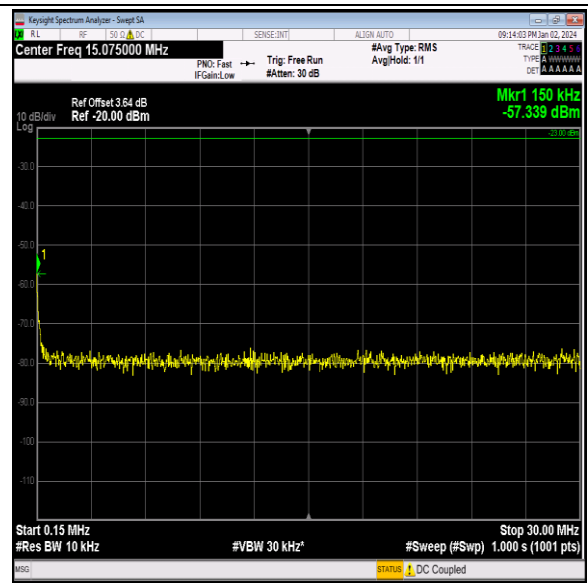
Band26_1.4MHz_16QAM_26915_1RB#0_0.15~30_0.15~ 30
