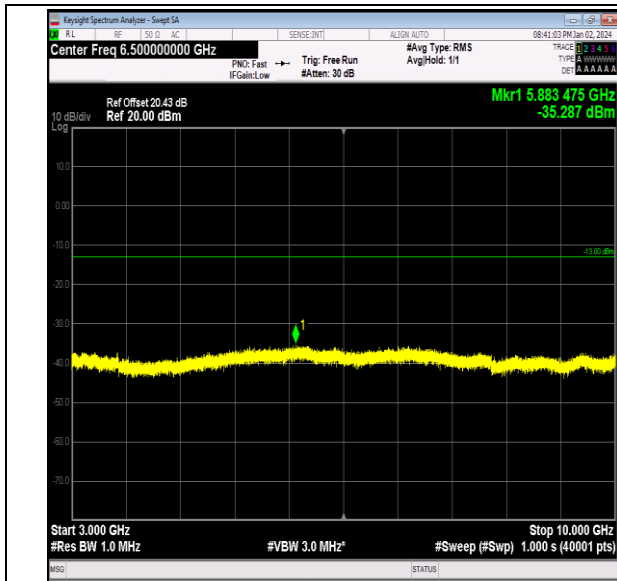
Band26_5MHz_16QAM_26740_1RB#0_3000~10000_300 0~10000
