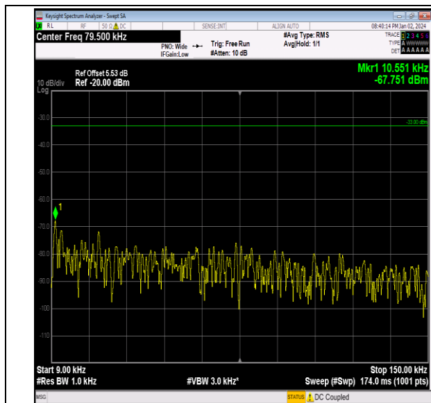
Band26_5MHz_16QAM_26740_1RB#0_0.009~0.15_0.009 ~0.15
