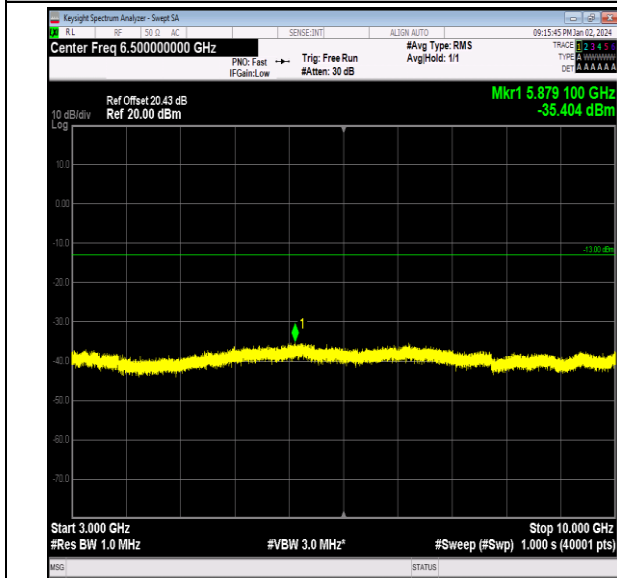
Band26_1.4MHz_QPSK_27033_1RB#0_3000~10000_300 0~10000
