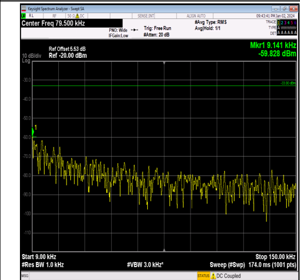
Band26_3MHz_16QAM_27025_1RB#0_0.009~0.15_0.009 ~0.15
