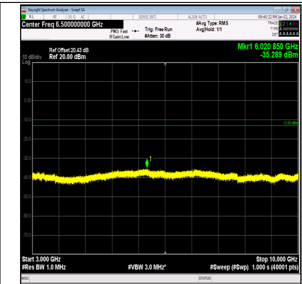
Band26_3MHz_16QAM_26805_1RB#0_3000~10000_300 0~10000
