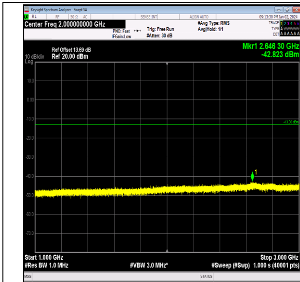
Band26_1.4MHz_QPSK_26915_1RB#0_1000~3000_1000 ~3000
