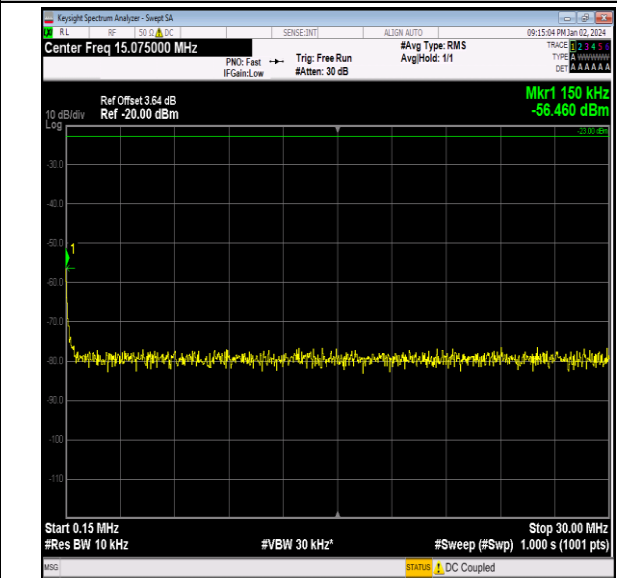
Band26_1.4MHz_QPSK_27033_1RB#0_0.15~30_0.15~30
