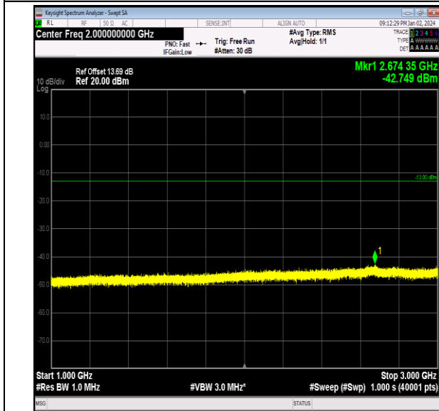
Band26_1.4MHz_16QAM_26797_1RB#0_1000~3000_1000~3000
