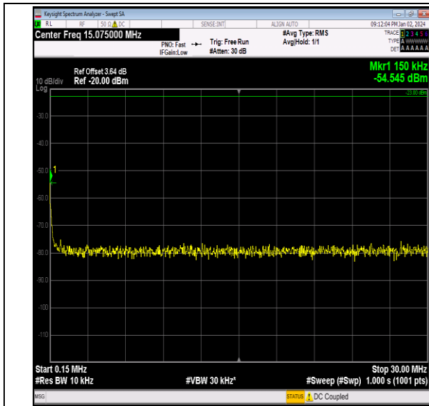
Band26_1.4MHz_16QAM_26797_1RB#0_0.15~30_0.15~30
