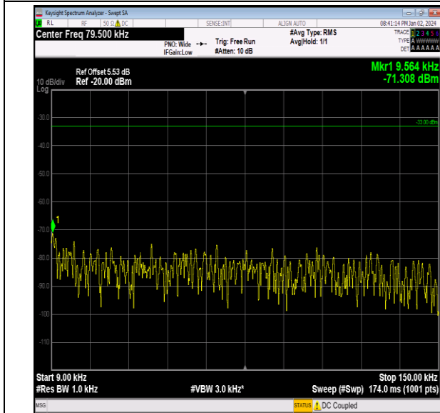
Band26_5MHz_QPSK_26765_1RB#0_0.009~0.15_0.009~0.15
