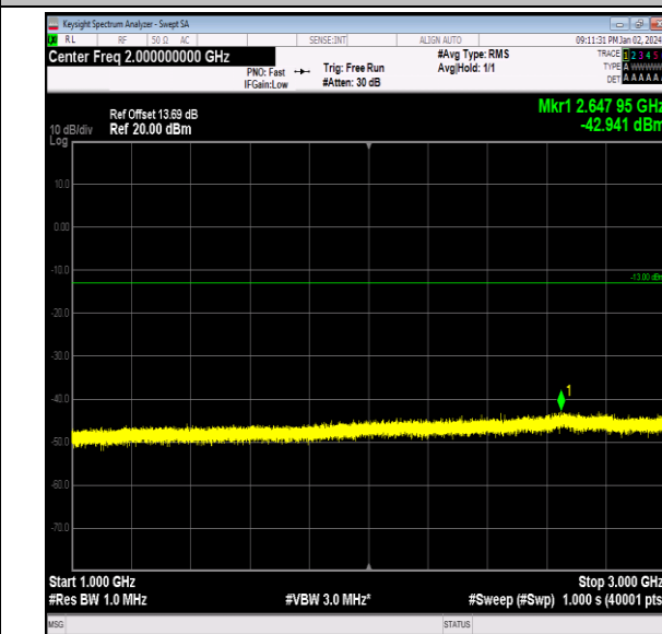
Band26_1.4MHz_QPSK_26797_1RB#0_1000~3000_1000 ~3000
