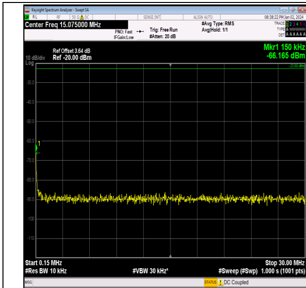
Band26_5MHz_16QAM_26715_1RB#0_0.15~30_0.15~30
