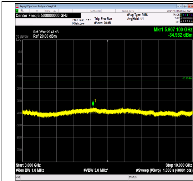
Band26_1.4MHz_16QAM_26915_1RB#0_3000~10000_30 00~10000
