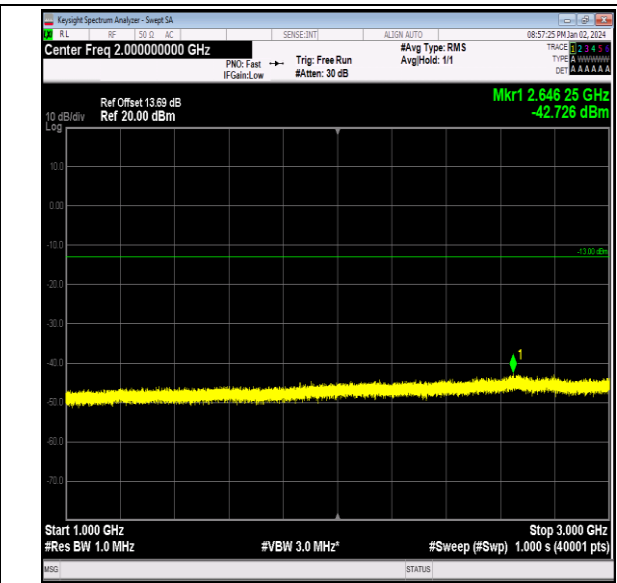
Band26_10MHz_QPSK_26740_1RB#0_1000~3000_1000 ~3000
