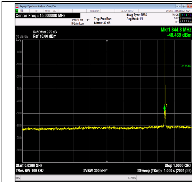
Band26_1.4MHz_QPSK_27033_1RB#0_30~1000_30~100 0
