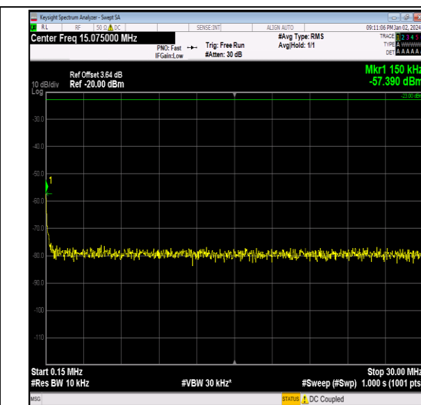
Band26_1.4MHz_QPSK_26797_1RB#0_0.15~30_0.15~30
