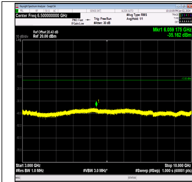
Band26_5MHz_QPSK_26815_1RB#0_3000~10000_3000 ~10000
