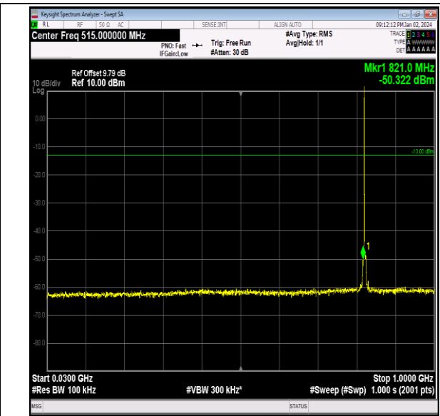
Band26_1.4MHz_16QAM_26797_1RB#0_30~1000_30~1000
