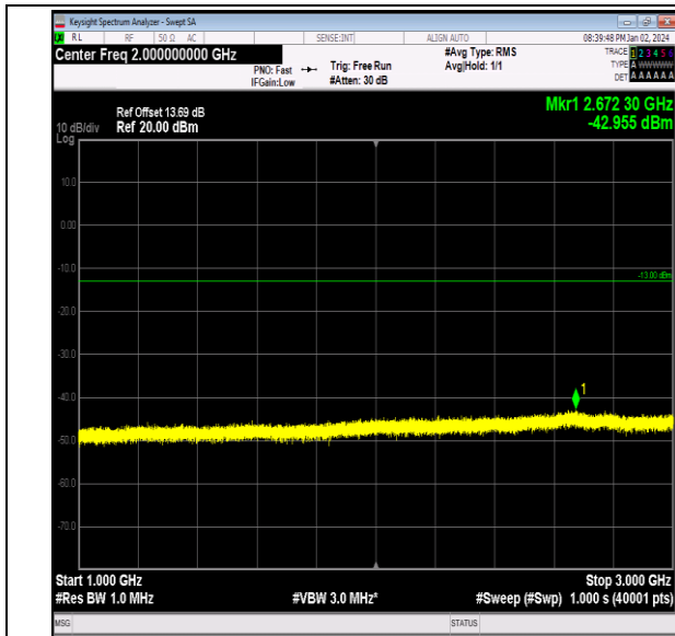
Band26_5MHz_QPSK_26740_1RB#0_1000~3000_1000~3000
