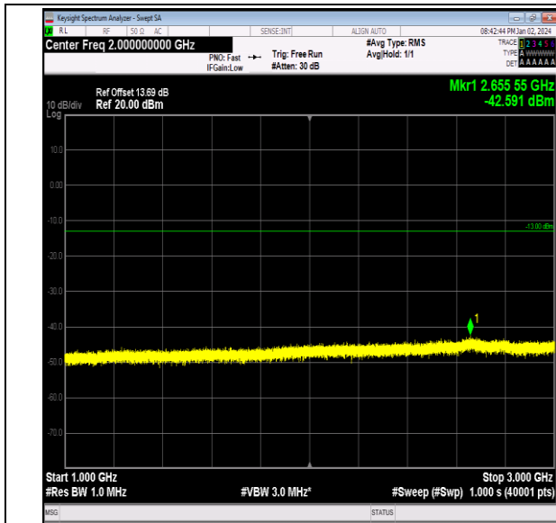
Band26_5MHz_16QAM_26765_1RB#0_1000~3000_1000 ~3000
