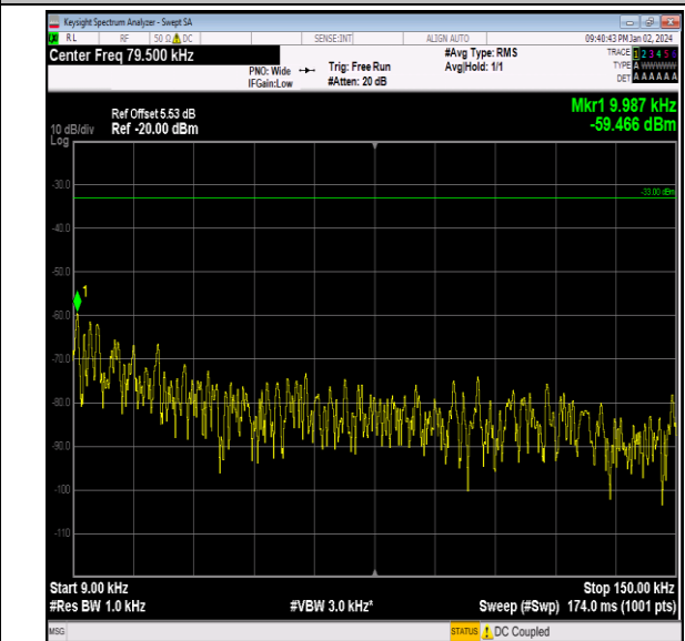
Band26_3MHz_QPSK_26915_1RB#0_0.009~0.15_0.009~0.15
