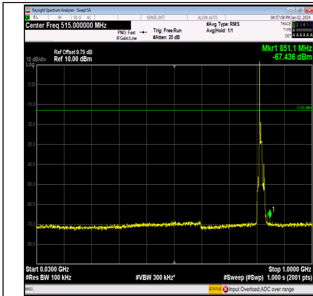
Band26_10MHz_QPSK_26740_1RB#0_30~1000_30~100 0
