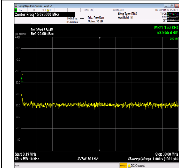
Band26_1.4MHz_16QAM_27033_1RB#0_0.15~30_0.15~ 30
