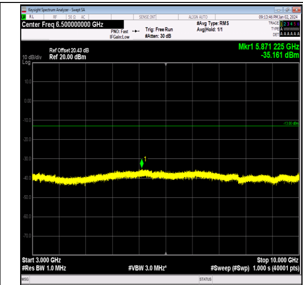
Band26_1.4MHz_QPSK_26915_1RB#0_3000~10000_300 0~10000
