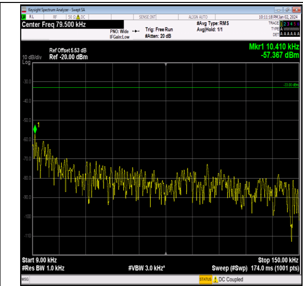
Band26_5MHz_QPSK_26915_1RB#0_0.009~0.15_0.009~ 0.15
