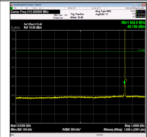
Band26_1.4MHz_16QAM_27033_1RB#0_30~1000_30~1 000
