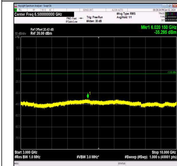
Band26_3MHz_QPSK_26805_1RB#0_3000~10000_3000~10000
