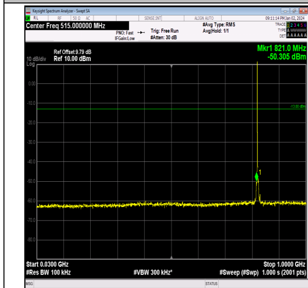
Band26_1.4MHz_QPSK_26797_1RB#0_30~1000_30~100 0
