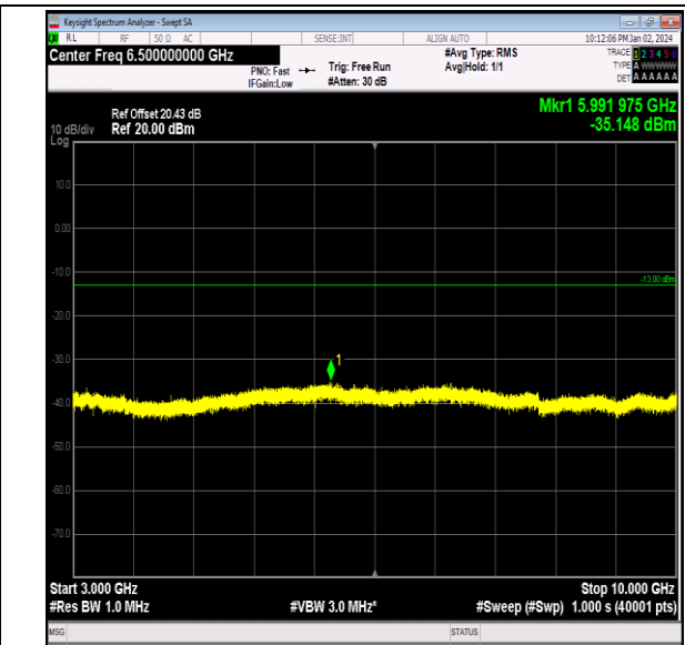
Band26_5MHz_QPSK_26915_1RB#0_3000~10000_3000~10000
