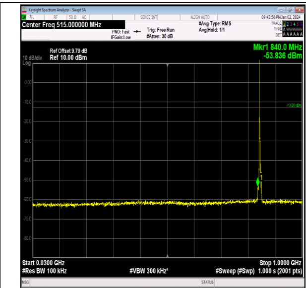
Band26_3MHz_16QAM_27025_1RB#0_30~1000_30~1000 0
