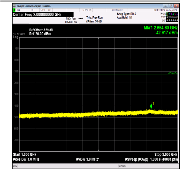
Band26_3MHz_QPSK_27025_1RB#0_1000~3000_1000~3000
