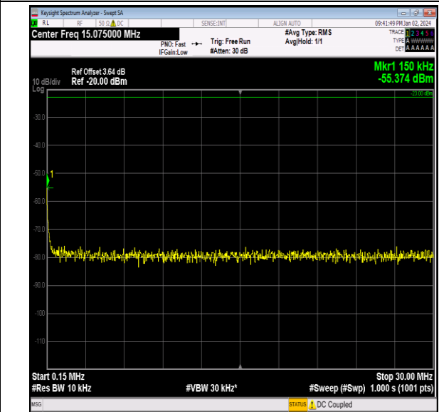
Band26_3MHz_16QAM_26915_1RB#0_0.15~30_0.15~30
