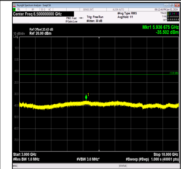
Band26_1.4MHz_16QAM_26797_1RB#0_3000~10000_3000~10000
