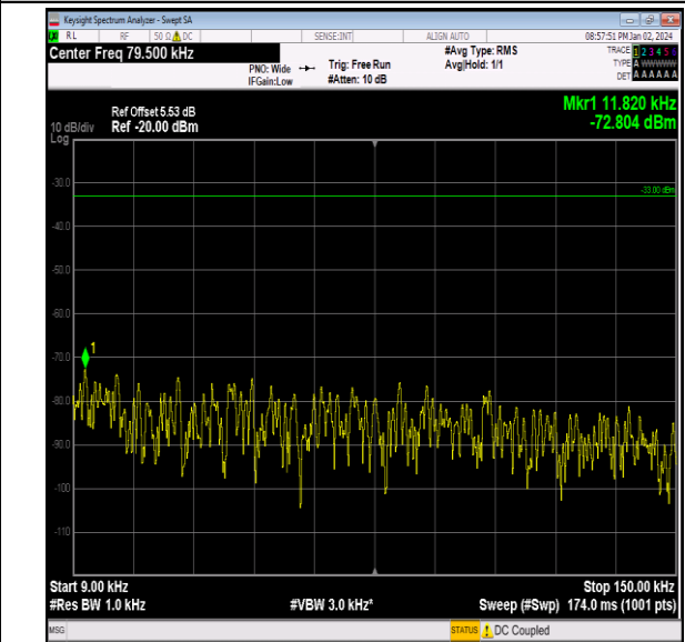
Band26_10MHz_16QAM_26740_1RB#0_0.009~0.15_0.00 9~0.15
