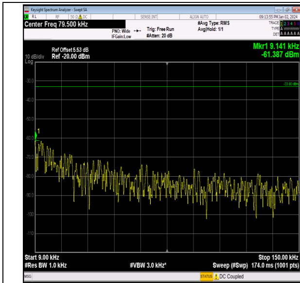
Band26_1.4MHz_16QAM_26915_1RB#0_0.009~0.15_0.0 09~0.15
