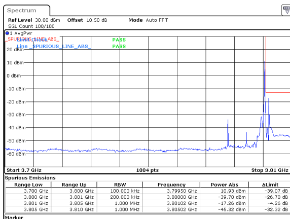
15MHz_15kHz_3792.5MHz_DFT-s-OFDM QPSK_RB1@78&amp;-17.26 dBm
