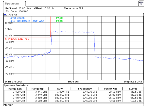
50MHz_30kHz_3475MHz_DFT-s-OFDM QPSK_RB128@0&-35.52 dBm
