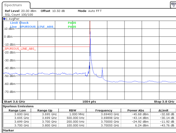
15MHz_15kHz_3707.5MHz_DFT-s-OFDM QPSK_RB1@0&amp;-24.92 dBm
