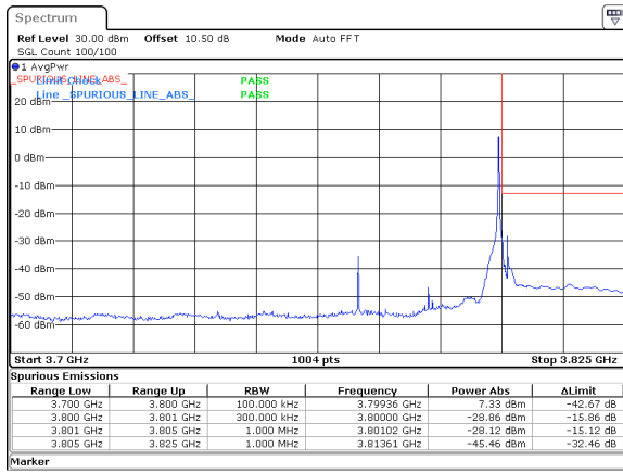
30MHz_15kHz_3785MHz_DFT-s-OFDM QPSK_RB1@159&amp;-28.12 dBm
