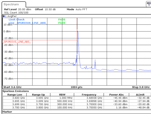
25MHz_30kHz_3712.5MHz_DFT-s-OFDM QPSK_RB1@0&amp;-33.60 dBm
