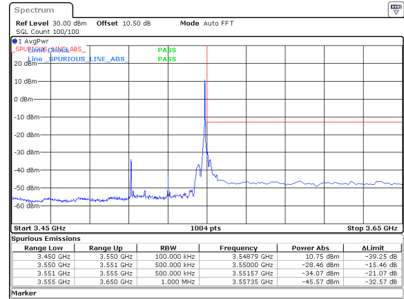
40MHz_30kHz_3530MHz_DFT-s-OFDM QPSK_RB1@105&-28.46 dBm
