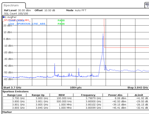
50MHz_30kHz_3775MHz_DFT-s-OFDM QPSK_RB1@132&amp;-39.15 dBm
