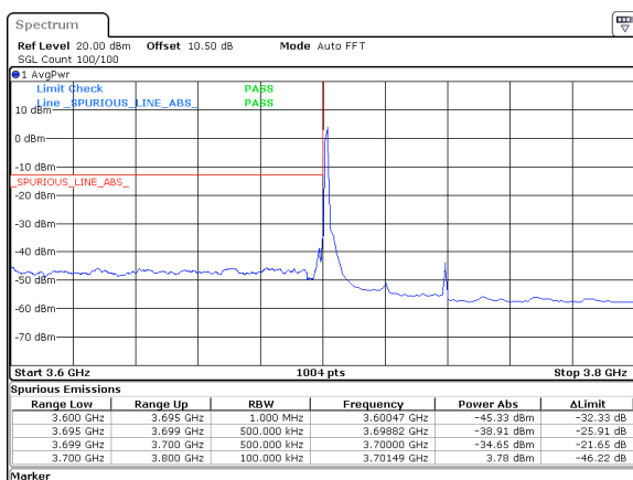
40MHz_15kHz_3720MHz_DFT-s-OFDM QPSK_RB1@0&amp;-34.65 dBm
