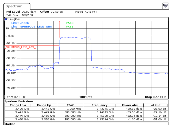
30MHz_15kHz_3465MHz_DFT-s-OFDM QPSK_RB160@0&amp;-32.14 dBm
