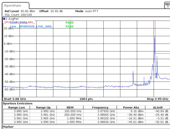
15MHz_15kHz_3972.5MHz_DFT-s-OFDM QPSK_RB1@78&amp;-16.51 dBm
