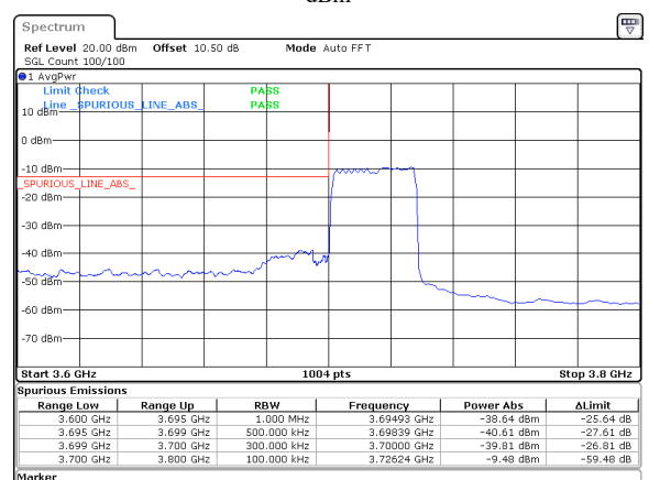
30MHz_30kHz_3715MHz_DFT-s-OFDM QPSK_RB75@0&amp;-38.64 dBm
