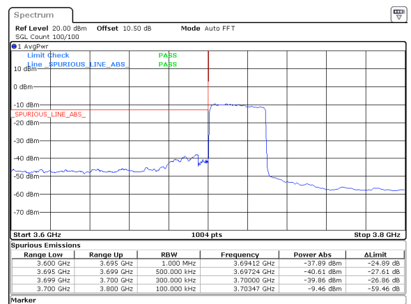
30MHz_15kHz_3715MHz_DFT-s-OFDM QPSK_RB160@0&amp;-37.89 dBm
