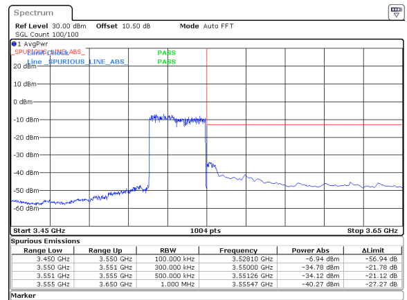
30MHz_15kHz_3535MHz_DFT-s-OFDM QPSK_RB160@0&amp;-34.12 dBm
