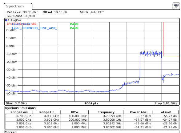
15MHz_15kHz_3792.5MHz_DFT-s-OFDM QPSK_RB75@0&amp;-34.71 dBm
