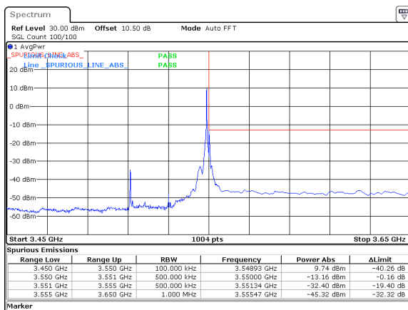
40MHz_30kHz_3530MHz_DFT-s-OFDM QPSK_RB1@105&amp;-13.16 dBm
