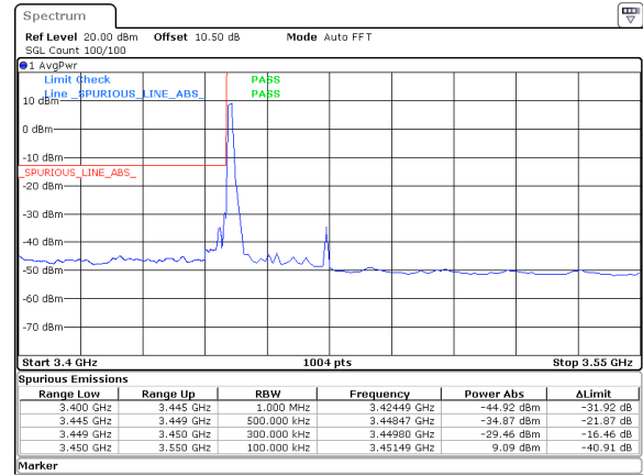
25MHz_30kHz_3462.5MHz_DFT-s-OFDM QPSK_RB1@0&-29.46 dBm
