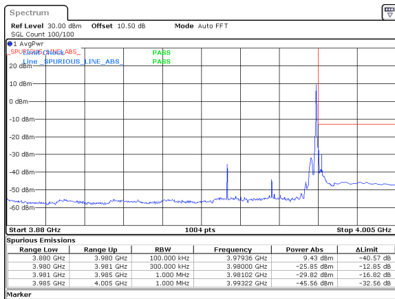
30MHz_15kHz_3965MHz_DFT-s-OFDM QPSK_RB1@159&amp;-25.85 dBm
