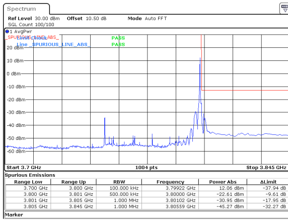
50MHz_15kHz_3775MHz_DFT-s-OFDM QPSK_RB1@269&amp;-22.61 dBm
