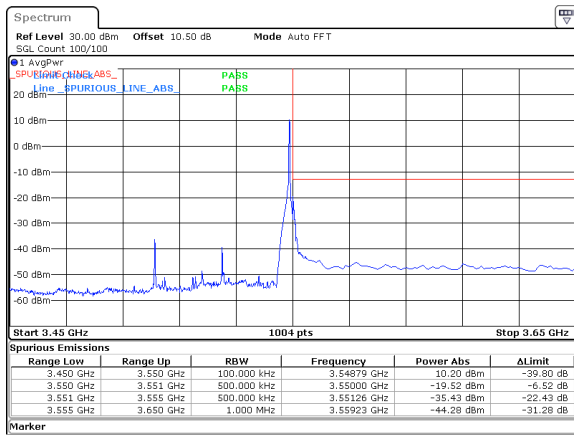
50MHz_30kHz_3525MHz_DFT-s-OFDM QPSK_RB1@132&amp;-19.52 dBm
