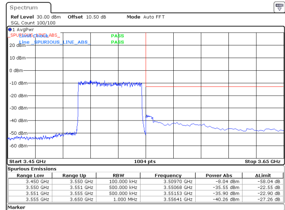
50MHz_30kHz_3525MHz_DFT-s-OFDM QPSK_RB128@0&-35.55 dBm
