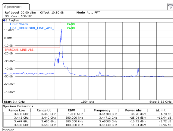
70MHz_30kHz_3485MHz_DFT-s-OFDM QPSK_RB1@0&amp;-16.72 dBm
