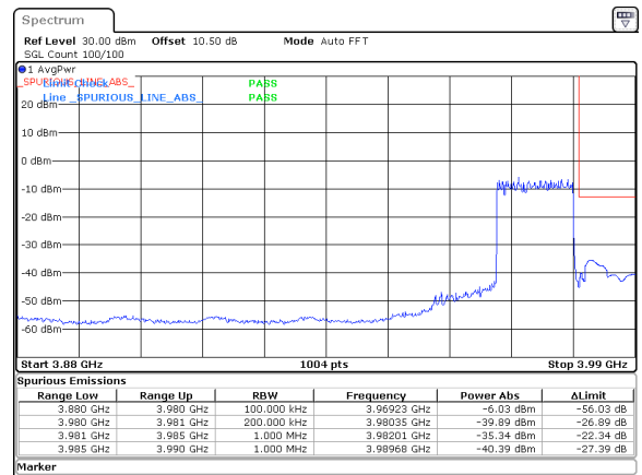
15MHz_15kHz_3972.5MHz_DFT-s-OFDM QPSK_RB75@0&amp;-35.34 dBm
