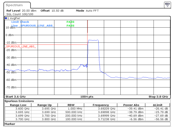
15MHz_30kHz_3707.5MHz_DFT-s-OFDM QPSK_RB36@0&amp;-38.79 dBm
