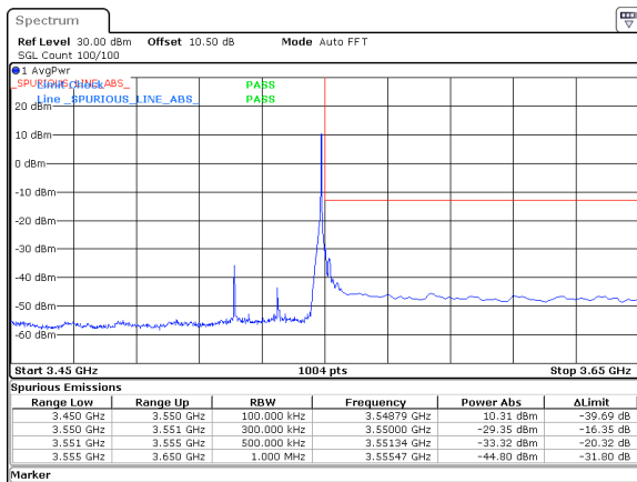
30MHz_30kHz_3535MHz_DFT-s-OFDM QPSK_RB1@77&amp;-29.35 dBm
