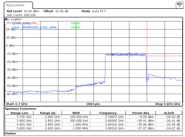
30MHz_15kHz_3785MHz_DFT-s-OFDM QPSK_RB160@0&amp;-35.06 dBm
