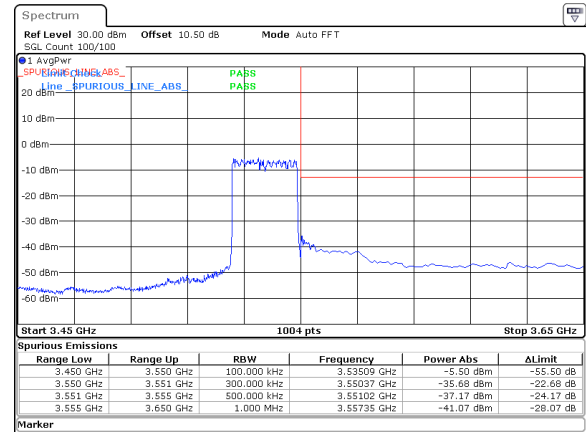
25MHz_30kHz_3537.5MHz_DFT-s-OFDM QPSK_RB64@0&-35.68 dBm
