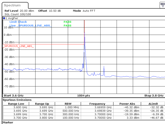
25MHz_15kHz_3712.5MHz_DFT-s-OFDM QPSK_RB1@0&amp;-19.59 dBm
