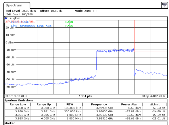
30MHz_15kHz_3965MHz_DFT-s-OFDM QPSK_RB160@0&amp;-35.59 dBm
