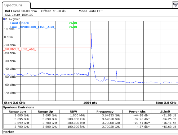
30MHz_15kHz_3715MHz_DFT-s-OFDM QPSK_RB1@0&amp;-29.41 dBm
