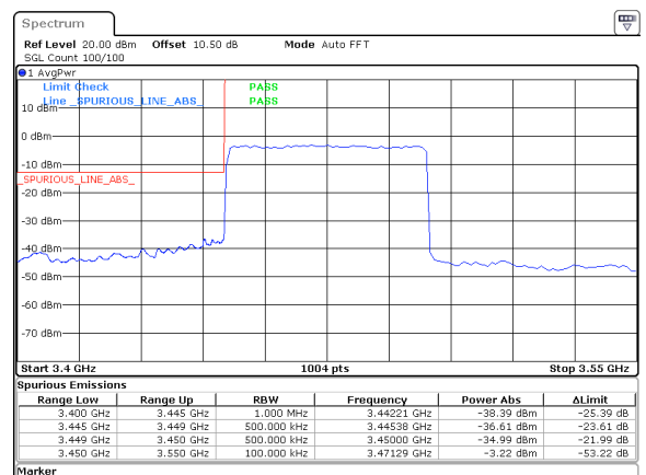
50MHz_15kHz_3475MHz_DFT-s-OFDM QPSK_RB270@0&amp;-34.99 dBm
