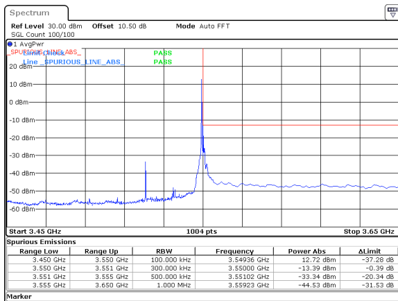
30MHz_15kHz_3535MHz_DFT-s-OFDM QPSK_RB1@159&amp;-13.39 dBm
