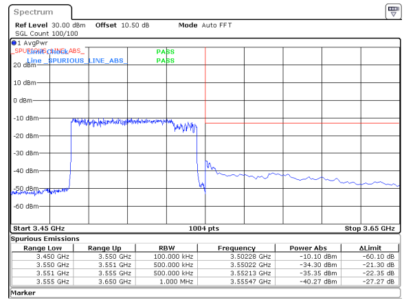
70MHz_30kHz_3515MHz_DFT-s-OFDM QPSK_RB180@0&amp;-34.30 dBm
