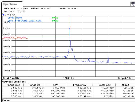
60MHz_30kHz_3730MHz_DFT-s-OFDM QPSK_RB1@0&amp;-31.96 dBm
