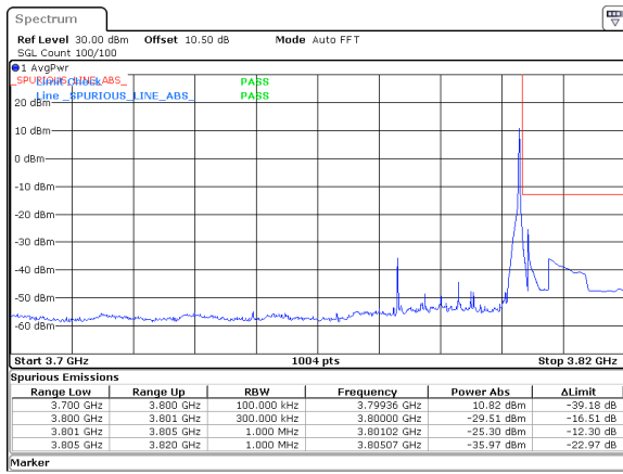
25MHz_15kHz_3787.5MHz_DFT-s-OFDM QPSK_RB1@132&amp;-25.30 dBm
