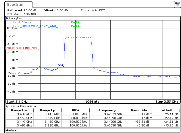
25MHz_30kHz_3462.5MHz_DFT-s-OFDM QPSK_RB64@0&-35.17 dBm
