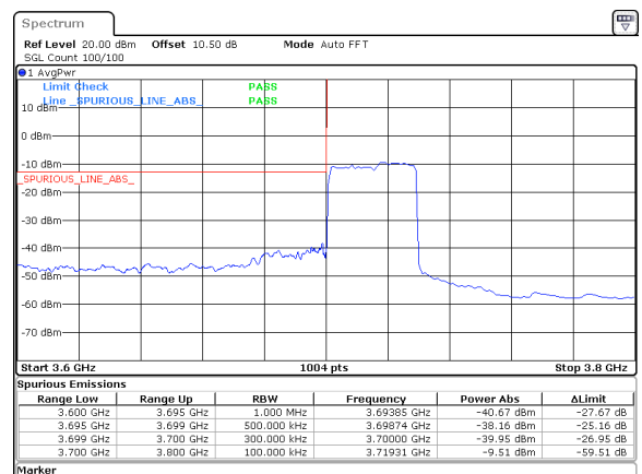
30MHz_15kHz_3715MHz_DFT-s-OFDM QPSK_RB160@0&amp;-38.16 dBm
