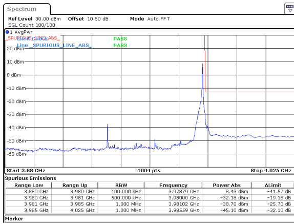
50MHz_30kHz_3955MHz_DFT-s-OFDM QPSK_RB1@132&amp;-32.18 dBm
