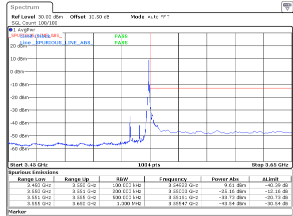
15MHz_30kHz_3542.5MHz_DFT-s-OFDM QPSK_RB1@37&-25.16 dBm
