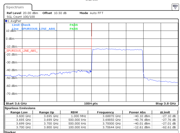
60MHz_30kHz_3730MHz_DFT-s-OFDM QPSK_RB162@0&amp;-40.01 dBm
