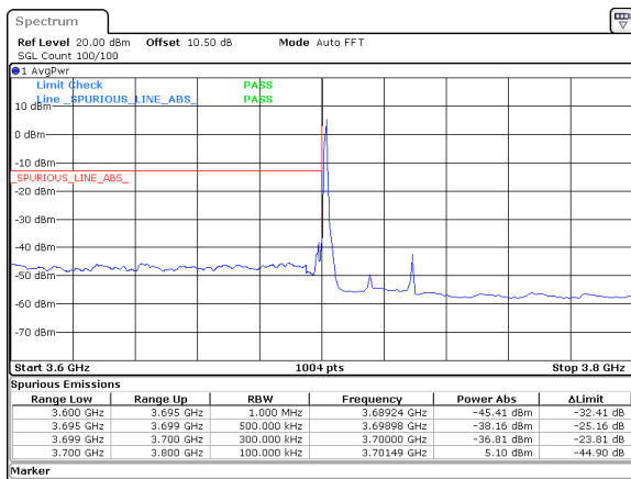
30MHz_30kHz_3715MHz_DFT-s-OFDM QPSK_RB1@0&amp;-36.81 dBm
