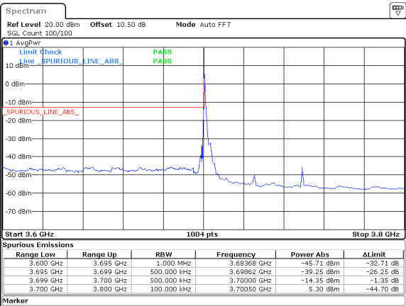
50MHz_15kHz_3725MHz_DFT-s-OFDM QPSK_RB1@0&-14.35 dBm
