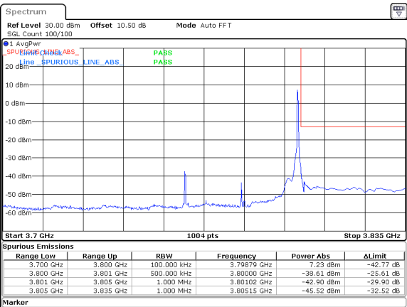
40MHz_30kHz_3780MHz_DFT-s-OFDM QPSK_RB1@105&-38.61 dBm
