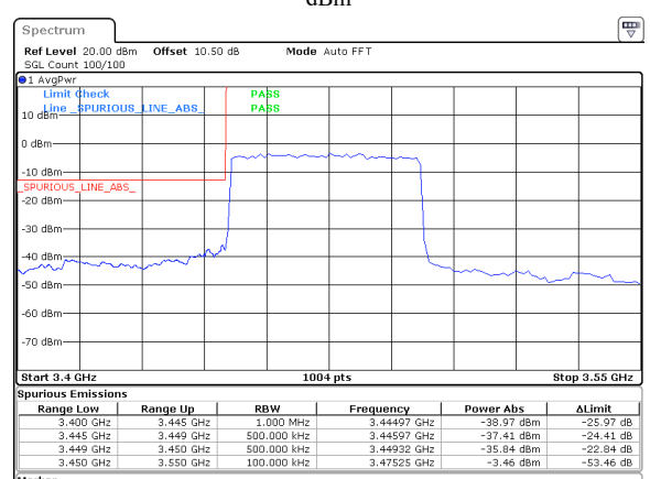
50MHz_30kHz_3475MHz_DFT-s-OFDM QPSK_RB128@0&amp;-35.84 dBm
