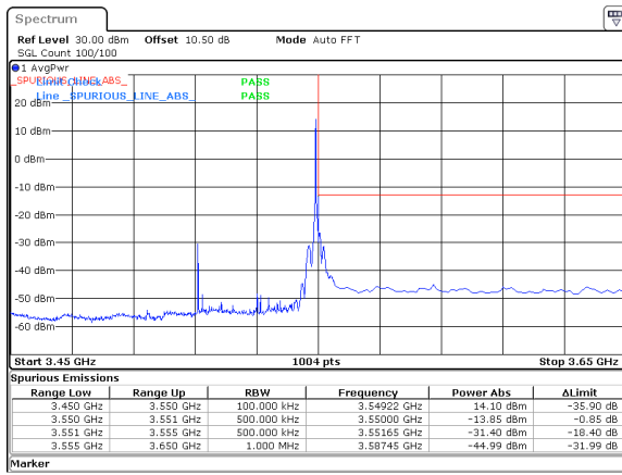
40MHz_15kHz_3530MHz_DFT-s-OFDM QPSK_RB1@215&amp;-13.85 dBm
