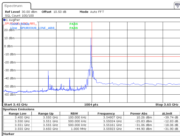
50MHz_15kHz_3525MHz_DFT-s-OFDM QPSK_RB1@269&amp;-25.83 dBm
