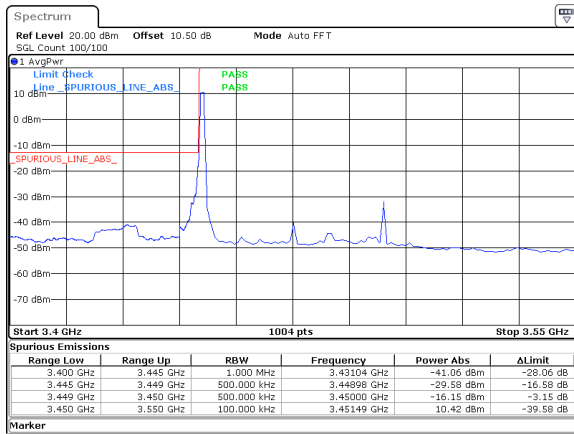
50MHz_15kHz_3475MHz_DFT-s-OFDM QPSK_RB1@0&amp;-16.15 dBm
