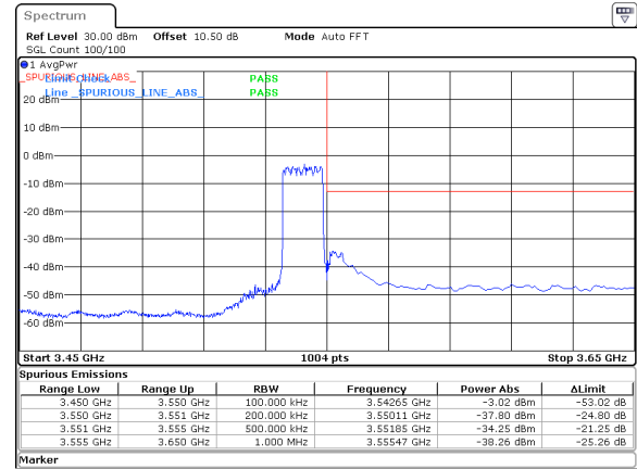
15MHz_30kHz_3542.5MHz_DFT-s-OFDM QPSK_RB36@0&-34.25 dBm
