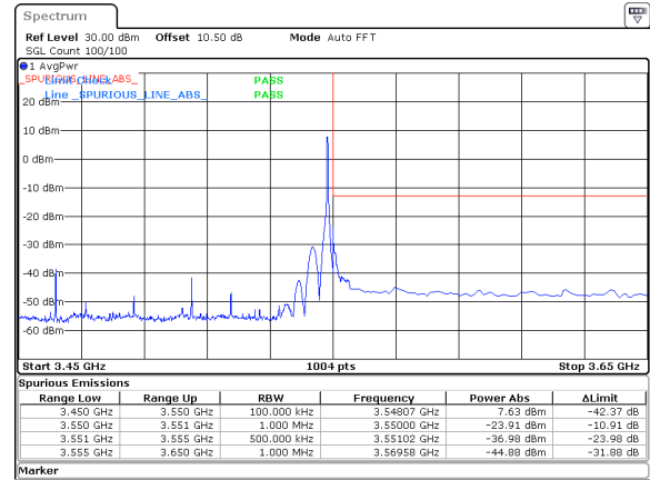
90MHz_30kHz_3505MHz_DFT-s-OFDM QPSK_RB1@244&-23.91 dBm
