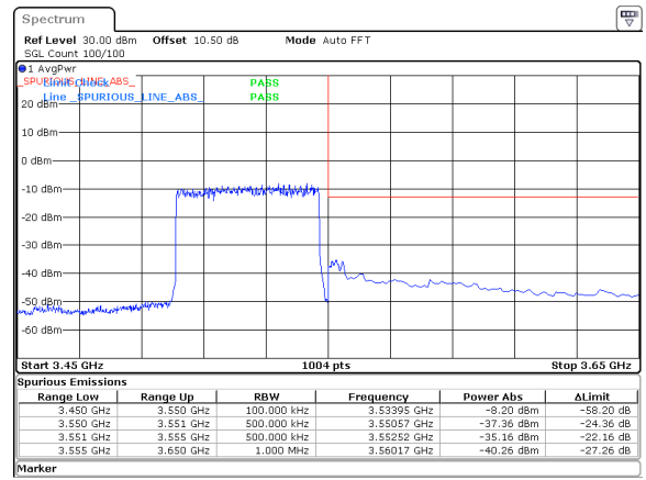
50MHz_30kHz_3525MHz_DFT-s-OFDM QPSK_RB128@0&amp;-35.16 dBm
