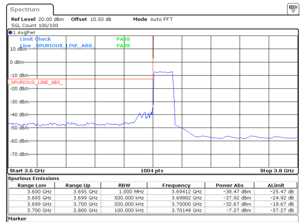
15MHz_15kHz_3707.5MHz_DFT-s-OFDM QPSK_RB75@0&amp;-32.67 dBm
