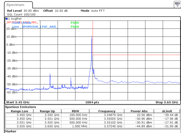
50MHz_30kHz_3525MHz_DFT-s-OFDM QPSK_RB1@132&-30.91 dBm
