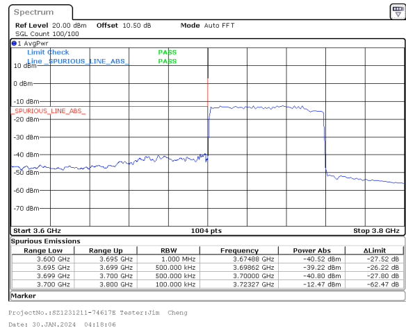
60MHz_30kHz_3730MHz_DFT-s-OFDM QPSK_RB162@0&-39.22 dBm
