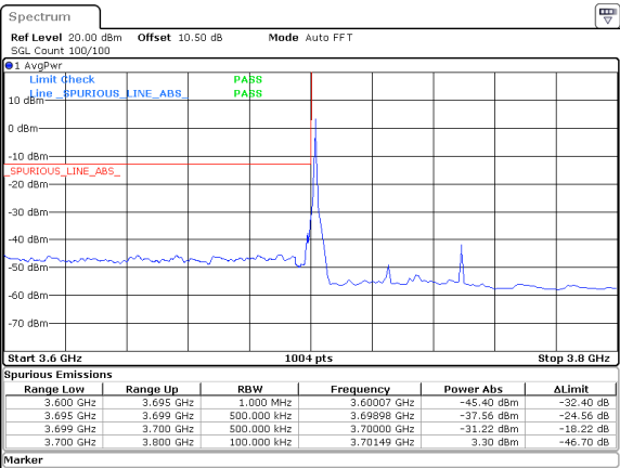
50MHz_30kHz_3725MHz_DFT-s-OFDM QPSK_RB1@0&-31.22 dBm
