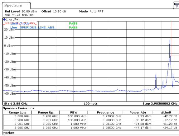
10MHz_30kHz_3975MHz_DFT-s-OFDM QPSK_RB1@23&amp;-30.12 dBm
