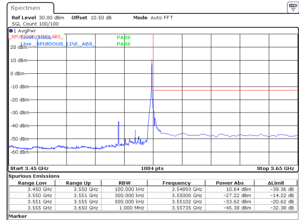
25MHz_30kHz_3537.5MHz_DFT-s-OFDM QPSK_RB1@64&-27.22 dBm
