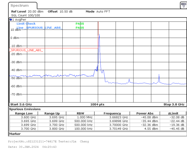
70MHz_30kHz_3735MHz_DFT-s-OFDM QPSK_RB1@0&-32.36 dBm
