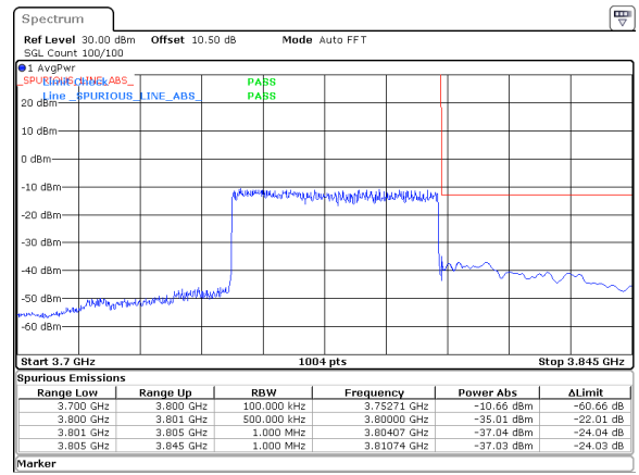
50MHz_15kHz_3775MHz_DFT-s-OFDM QPSK_RB270@0&amp;-35.01 dBm
