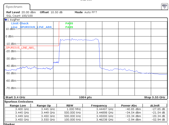
40MHz_30kHz_3470MHz_DFT-s-OFDM QPSK_RB100@0&amp;-33.34 dBm
