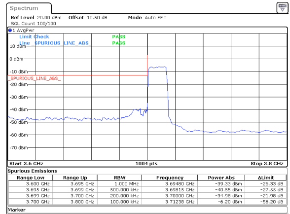
15MHz_15kHz_3707.5MHz_DFT-s-OFDM QPSK_RB75@0&amp;-34.98 dBm
