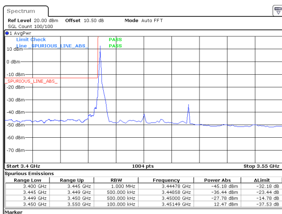
50MHz_30kHz_3475MHz_DFT-s-OFDM QPSK_RB1@0&amp;-27.78 dBm
