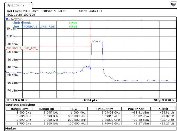
15MHz_30kHz_3707.5MHz_DFT-s-OFDM QPSK_RB36@0&-38.02 dBm
