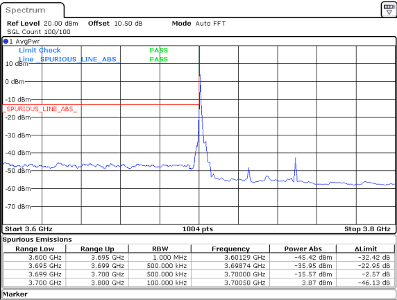
50MHz_15kHz_3725MHz_DFT-s-OFDM QPSK_RB1@0&-15.57 dBm
