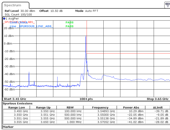
70MHz_30kHz_3515MHz_DFT-s-OFDM QPSK_RB1@188&amp;-22.05 dBm
