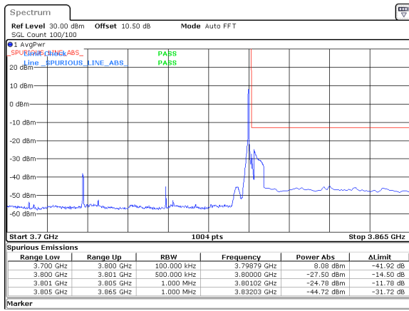
70MHz_30kHz_3765MHz_DFT-s-OFDM QPSK_RB1@188&amp;-24.78 dBm
