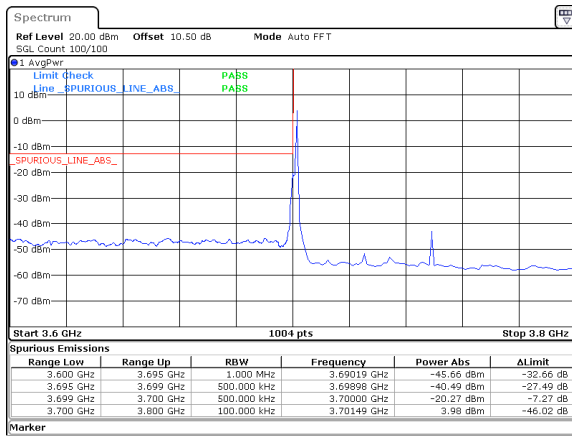
50MHz_30kHz_3725MHz_DFT-s-OFDM QPSK_RB1@0&amp;-20.27 dBm
