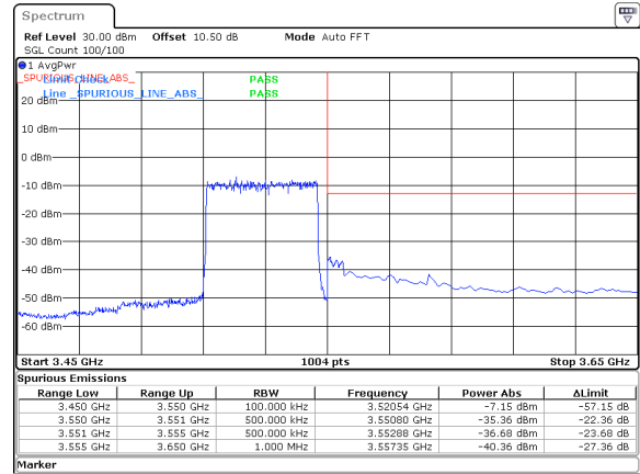
40MHz_30kHz_3530MHz_DFT-s-OFDM QPSK_RB100@0&-35.36 dBm
