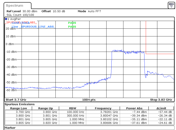
25MHz_30kHz_3787.5MHz_DFT-s-OFDM QPSK_RB64@0&amp;-35.11 dBm
