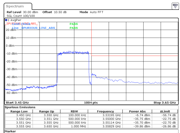
40MHz_30kHz_3530MHz_DFT-s-OFDM QPSK_RB100@0&amp;-35.70 dBm
