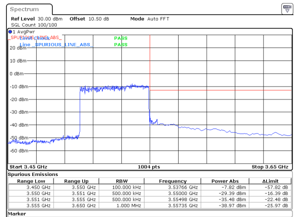
50MHz_15kHz_3525MHz_DFT-s-OFDM QPSK_RB270@0&amp;-29.39 dBm
