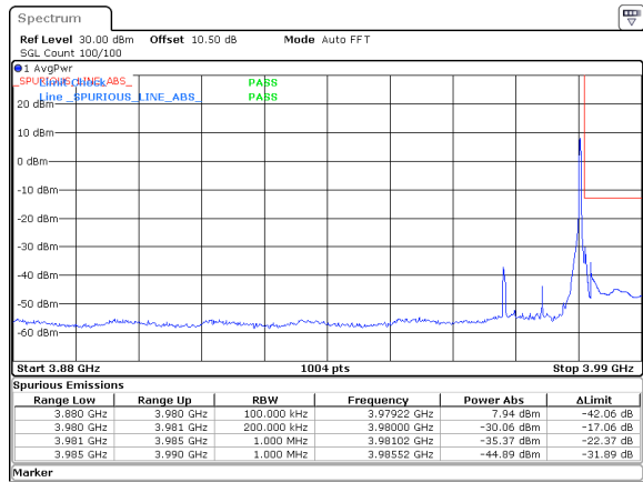
15MHz_30kHz_3972.5MHz_DFT-s-OFDM QPSK_RB1@37&-30.06 dBm
