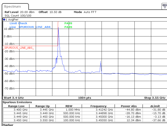
40MHz_15kHz_3470MHz_DFT-s-OFDM QPSK_RB1@0&amp;-16.13 dBm
