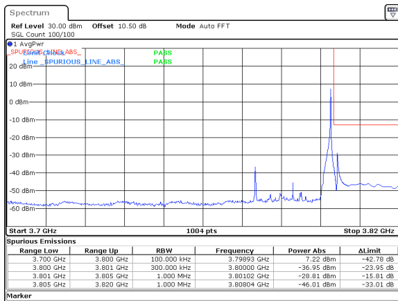
25MHz_30kHz_3787.5MHz_DFT-s-OFDM QPSK_RB1@64&amp;-28.81 dBm
