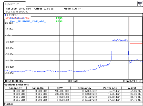
15MHz_30kHz_3972.5MHz_DFT-s-OFDM QPSK_RB36@0&-37.73 dBm
