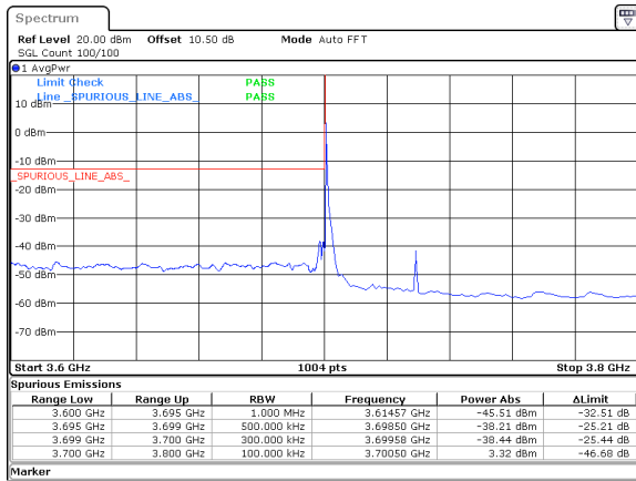
30MHz_15kHz_3715MHz_DFT-s-OFDM QPSK_RB1@0&amp;-38.21 dBm
