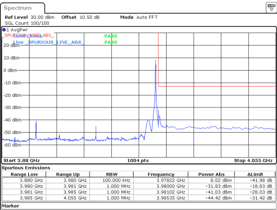
80MHz_30kHz_3940MHz_DFT-s-OFDM QPSK_RB1@216&-31.83 dBm
