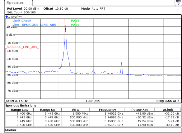
50MHz_30kHz_3475MHz_DFT-s-OFDM QPSK_RB1@0&-19.24 dBm
