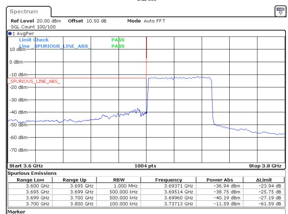
50MHz_30kHz_3725MHz_DFT-s-OFDM QPSK_RB128@0&amp;-36.94 dBm
