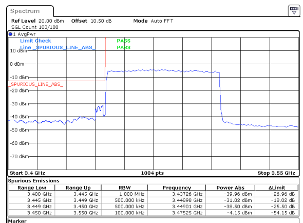
60MHz_30kHz_3480MHz_DFT-s-OFDM QPSK_RB162@0&amp;-31.02 dBm
