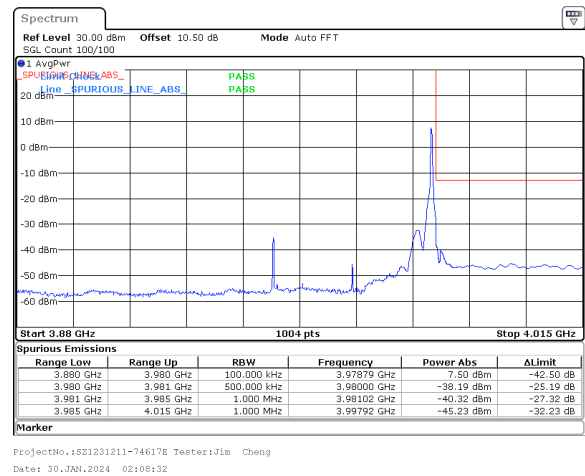
40MHz_30kHz_3960MHz_DFT-s-OFDM QPSK_RB1@105&-38.19 dBm
